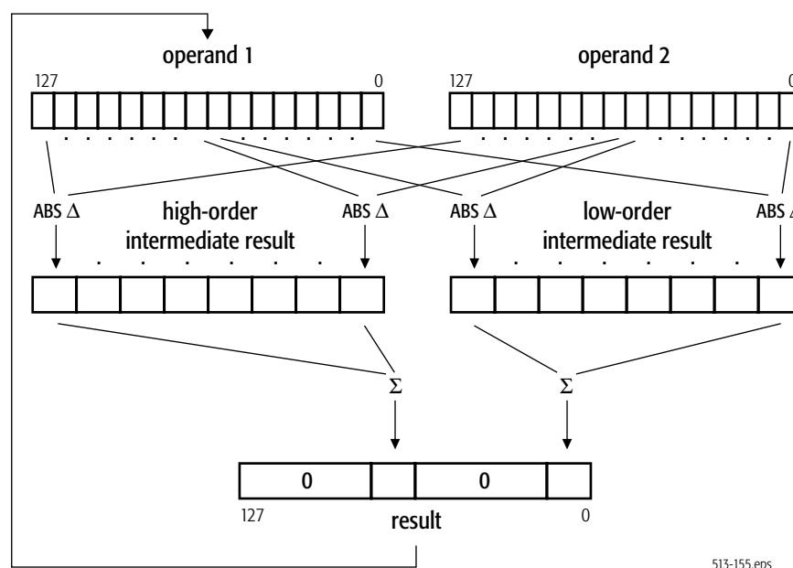
Figure 4-9. Sum-of-Absolute-Differences Operation
