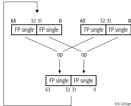
Figure 5-6. Floating-Point (3DNow!™) Operations
