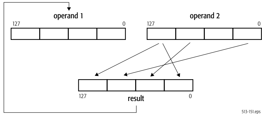
Figure 4-23. PSHUFD Shuffle Operation
