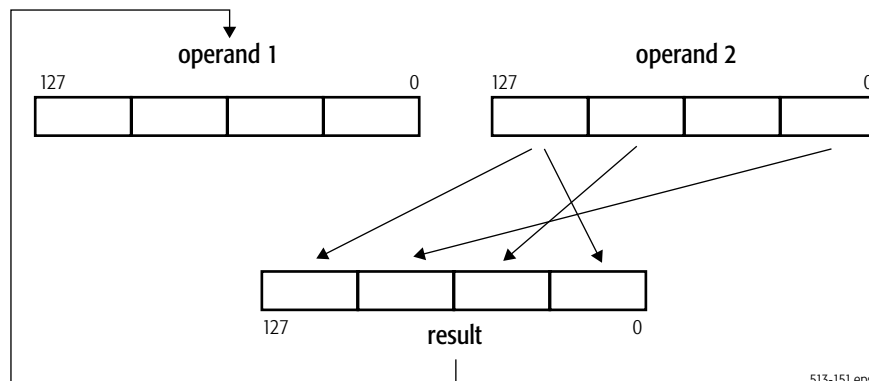
Figure 4-5. Shuffle Operation
