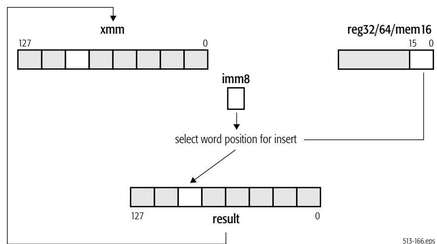
Figure 4-22. PINSRW Operation
