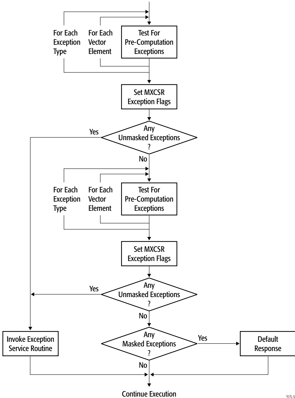
Figure 4-38. SIMD Floating-Point Detection Process
