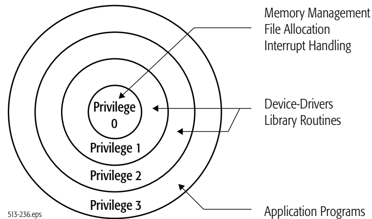
Figure 3-9. Privilege-Level Relationships
