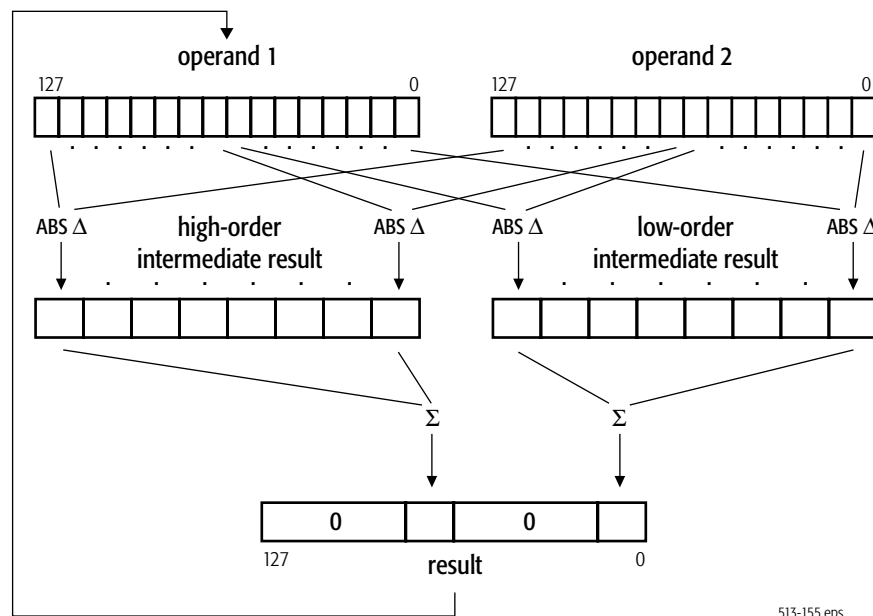
Figure 4-9. Sum-of-Absolute-Differences Operation
