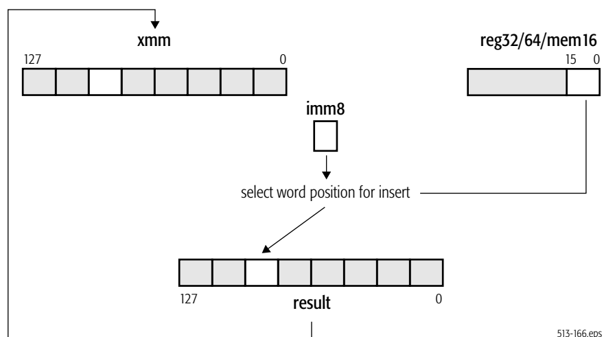
Figure 4-22. PINSRW Operation
