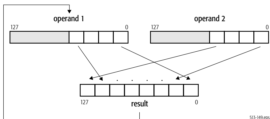
Figure 4-21. PUNPCKLWD Unpack and Interleave Operation
