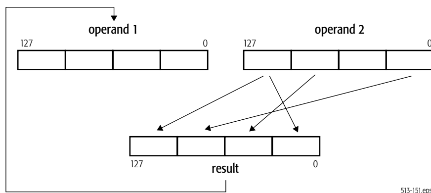
Figure 4-5. Shuffle Operation
