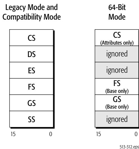
Figure 2-2. Segment Registers
