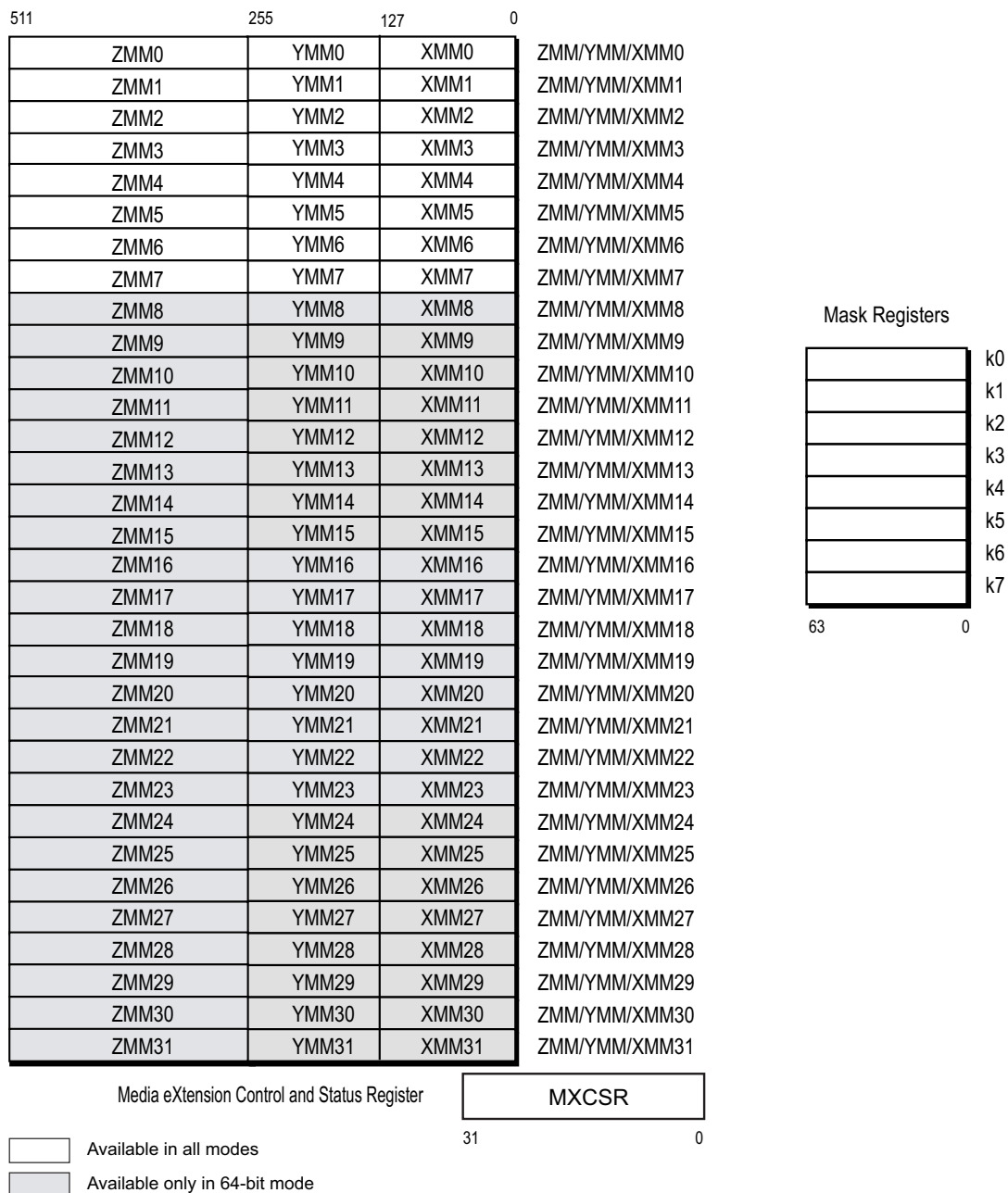
Figure 4-1. SSE Registers
