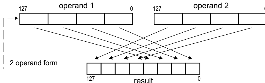
Figure 4-18. Pack Operation
