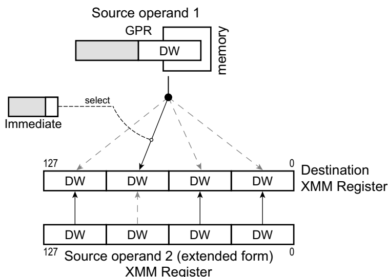
Figure 4-29. (V)PINSRD Operation
