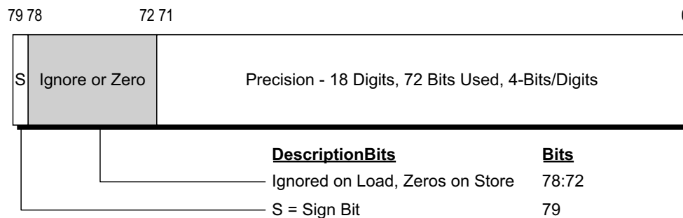
Figure 6-9. x87 Packed Decimal Data Type
