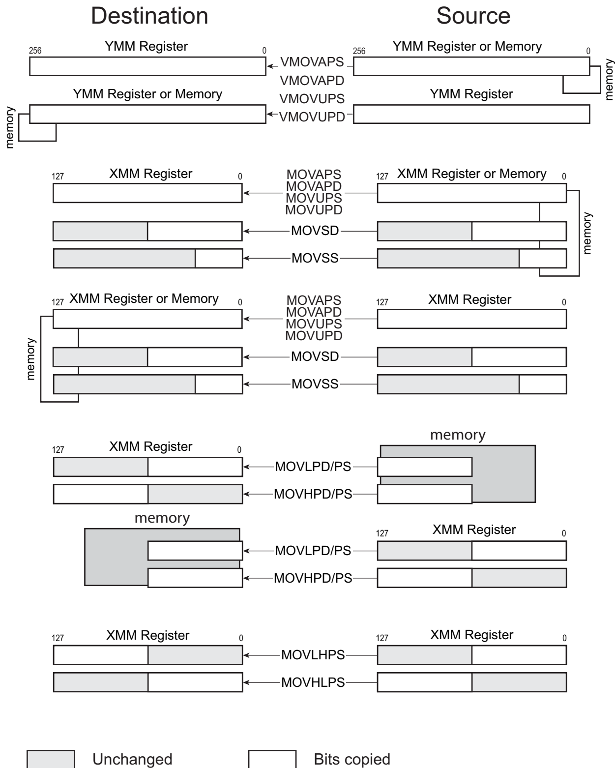
Figure 4-41. Floating-Point Move Operations
