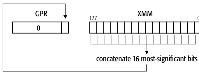
Figure 4-26. (V)PMOVMASKB Move Mask Operation
