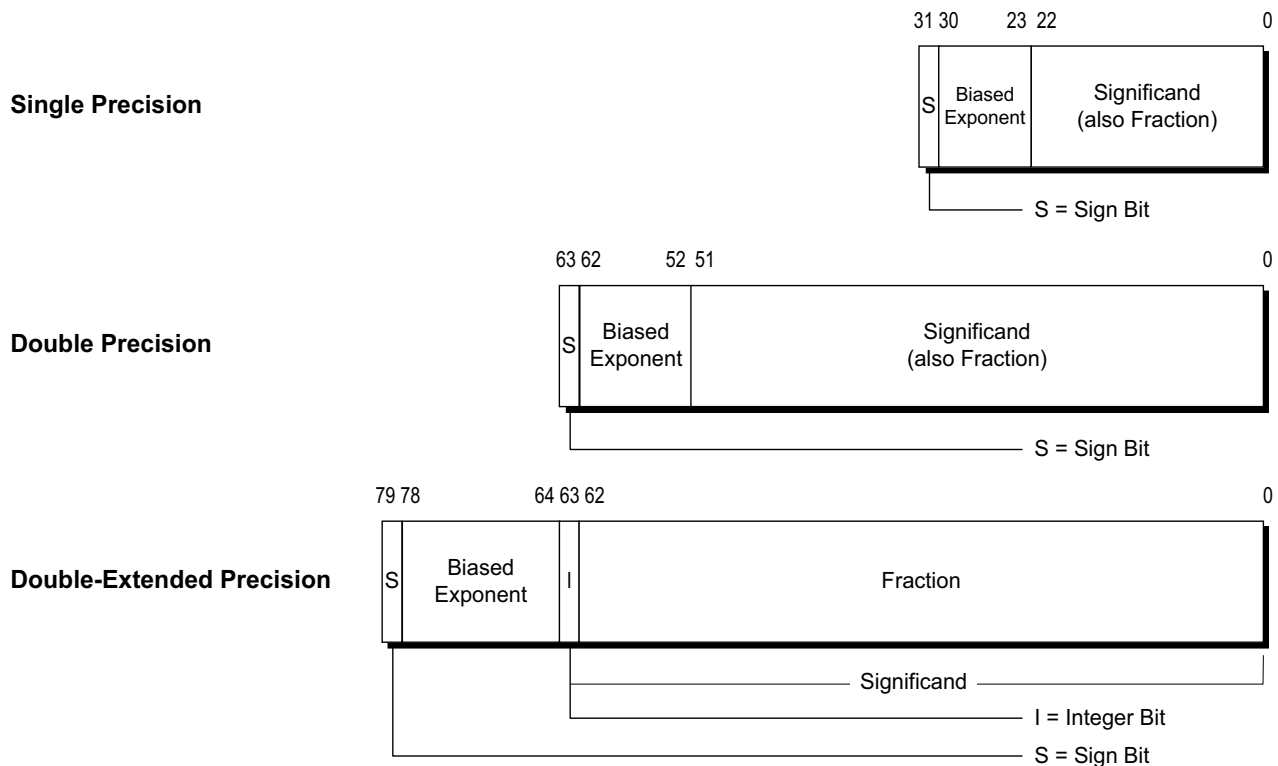
Figure 6-8. x87 Floating-Point Data Types
