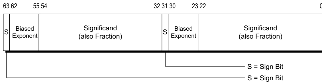
Figure 5-9. 64-Bit Floating-Point (3DNow!™) Vector Operand
