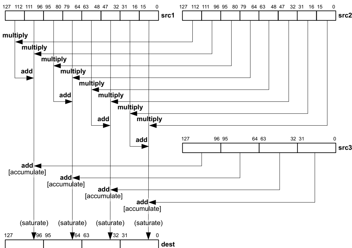
Figure 4-38. Operation of Multiply, Add and Accumulate Instructions
