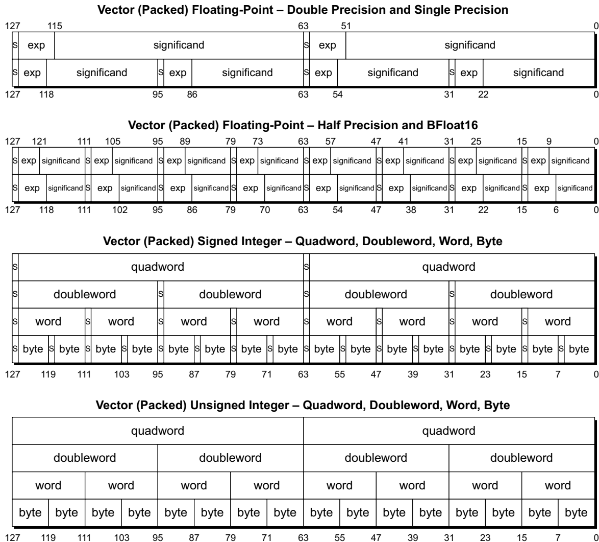
Figure 4-5. Examples of the 128-Bit Media Data Types
