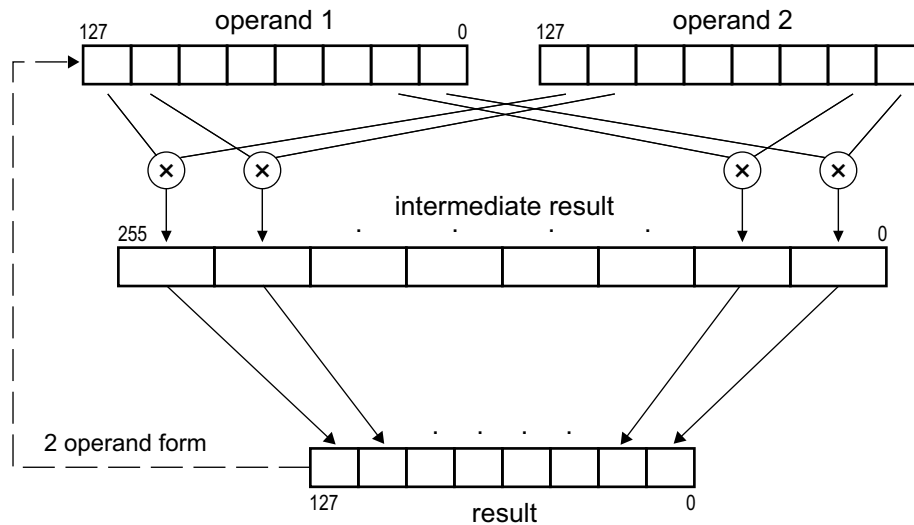
Figure 4-34. (V)PMULHW, (V)PMULLW, and (V)PMULHRWSW Instructions
