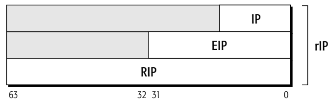
Figure 2-10. Instruction Pointer (rIP) Register
