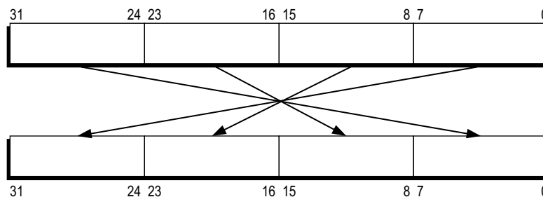
Figure 3-8. BSWAP Doubleword Exchange
