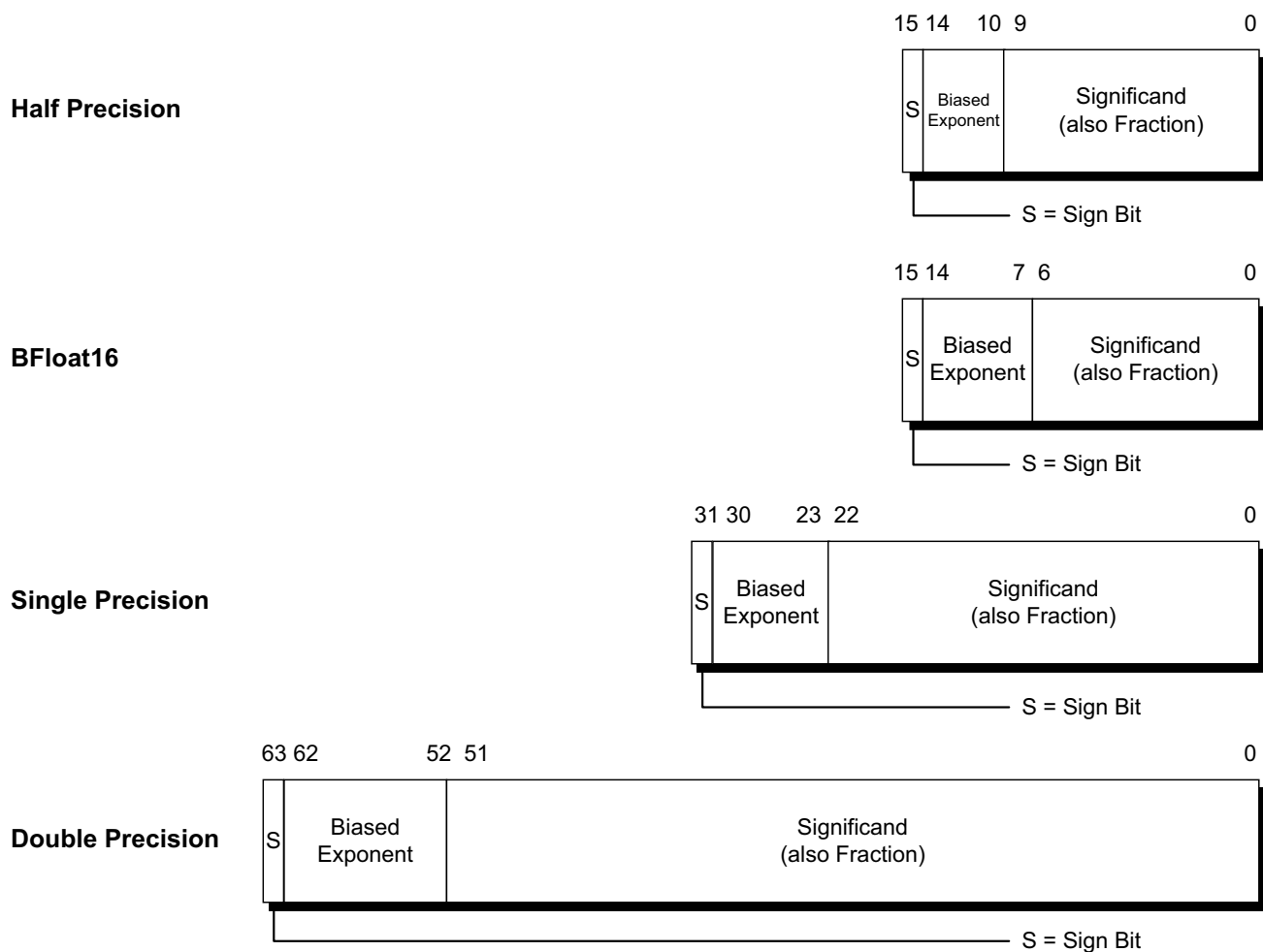
Figure 4-4. Floating-Point Data Types
