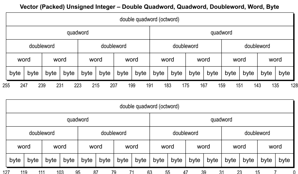
Figure 4-8. Examples of the 256-Bit Media Data Types (Continued)
