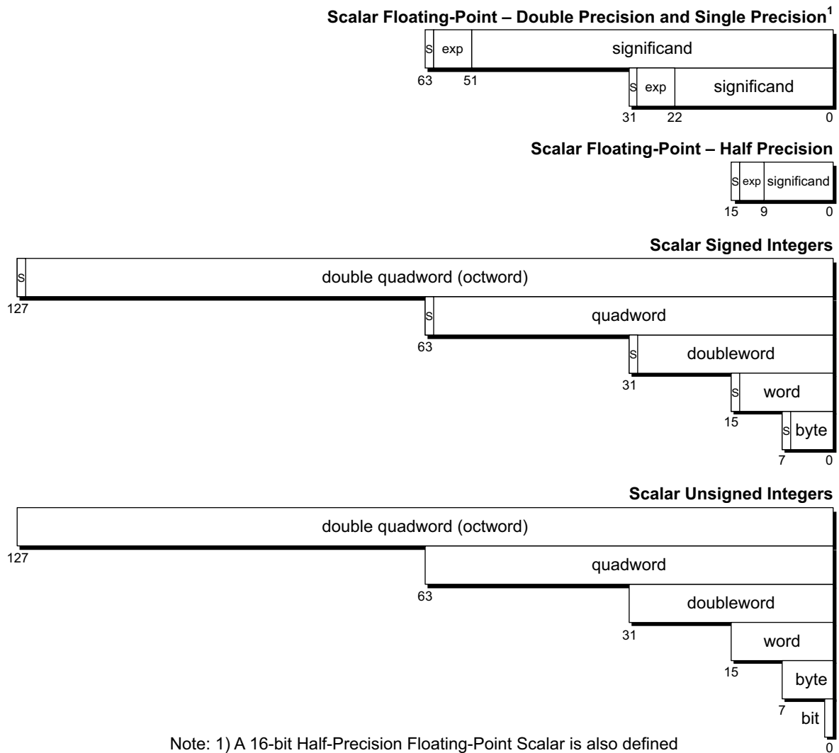
Figure 4-6. Examples of the 128-Bit Media Data Types (Continued)
