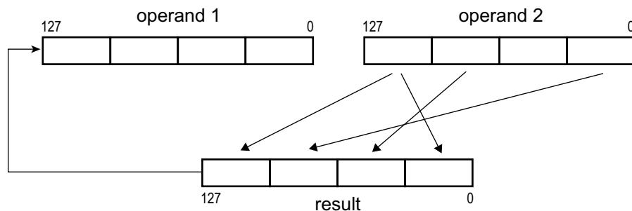
Figure 4-19. Shuffle Operation
