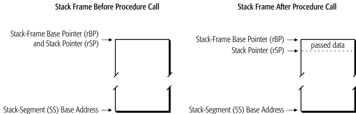
Figure 2-9. Stack Pointer Mechanism
