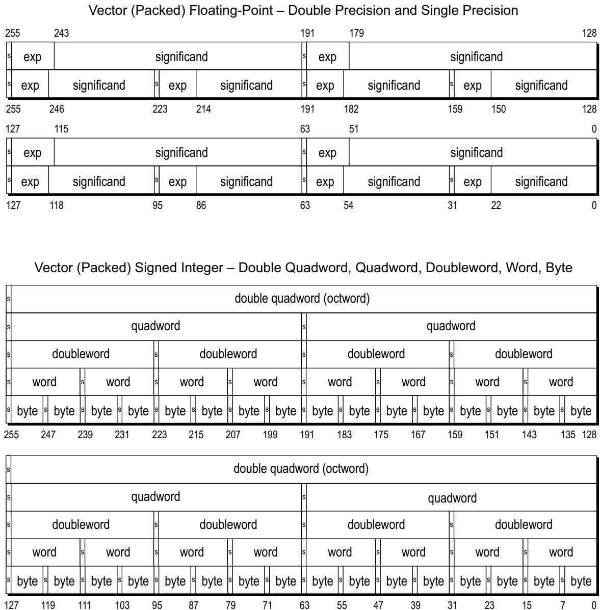
Figure 4-7. Examples of the 256-Bit Media Data Types
