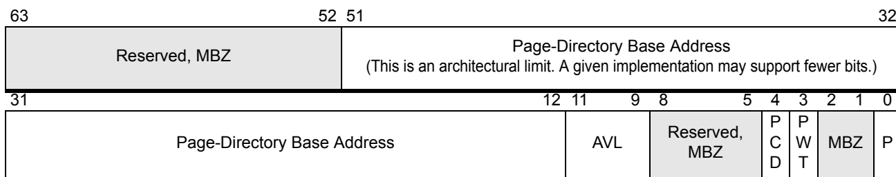
Figure 5-14. 2-Mbyte PDPE—PAE Paging Legacy-Mode
