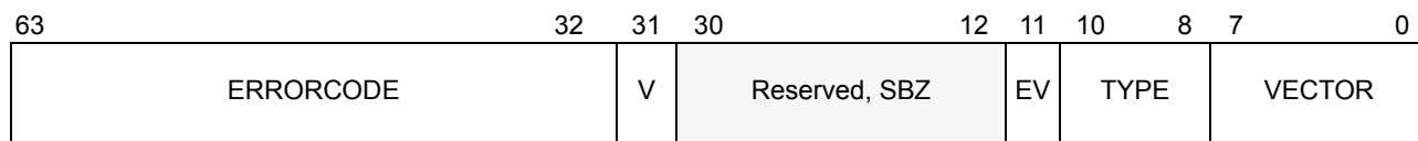
Figure 15-5. EVENTINJ Field in the VMCB
