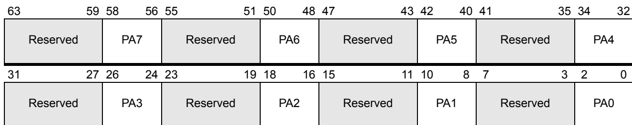
Figure 7-10. PAT Register
