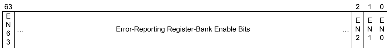
Figure 9-5. MC i _CTL Registers
