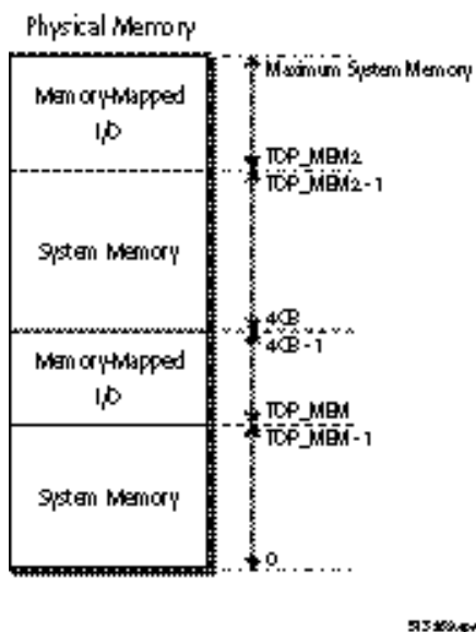
Figure 7-14. Memory Organization Using Top-of-Memory Registers
