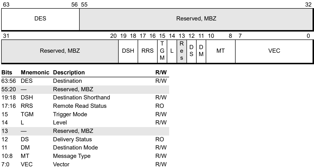
Figure 16-18. Interrupt Command Register (APIC Offset 300h–3010h)
