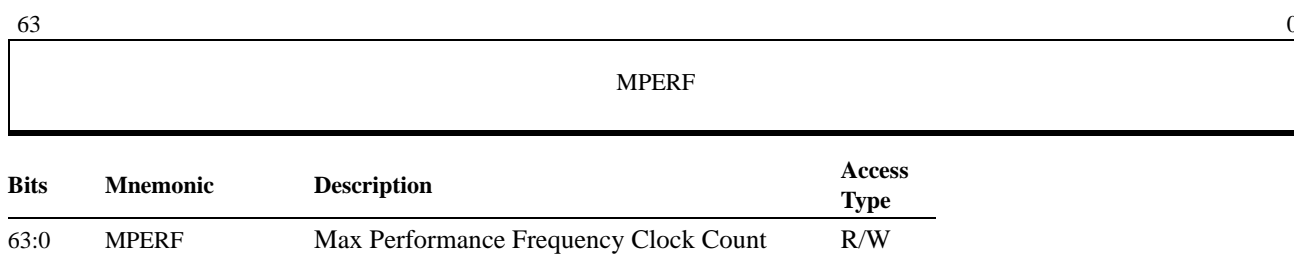
Figure 17-6. Max Performance Frequency Count (MSR0000_00E7h)
