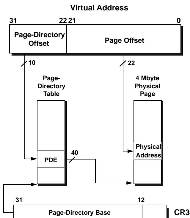
Figure 5-7. 4-Mbyte Page Translation—Non-PAE Paging Legacy-Mode
