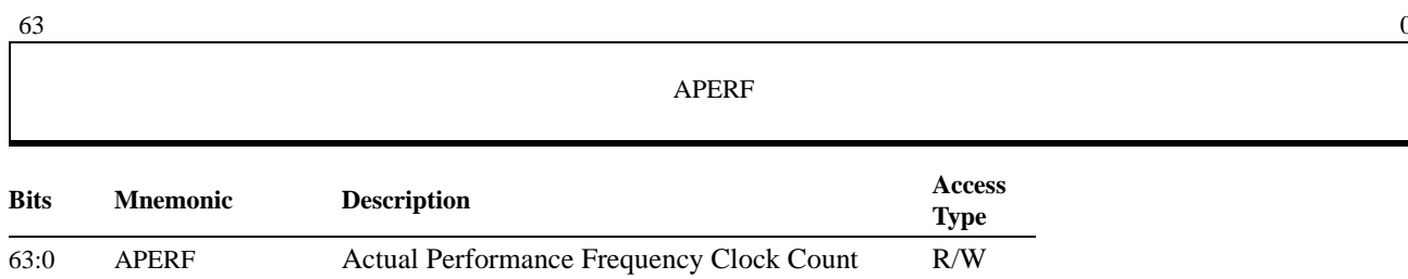
Figure 17-5. Actual Performance Frequency Count (MSR0000_00E8h)
