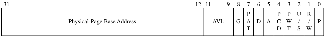
Figure 5-6. 4-Kbyte PTE—Non-PAE Paging Legacy-Mode
