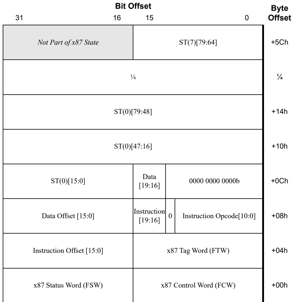
Figure 11-7. FSAVE/FNSAVE Image (16-Bit, Real/Virtual-8086 Modes)
