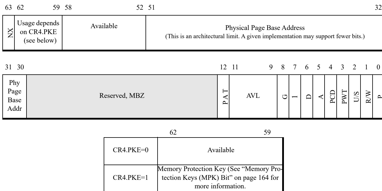
Figure 5-34. 1-Byte PDPE—Long Mode
