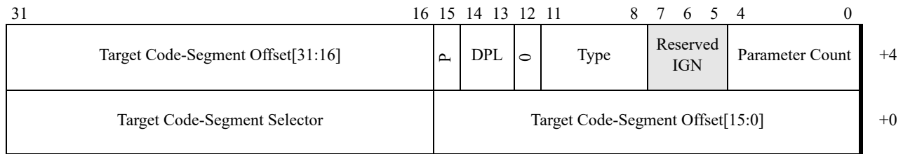
Figure 4-17. Call-Gate Descriptor—Legacy Mode
