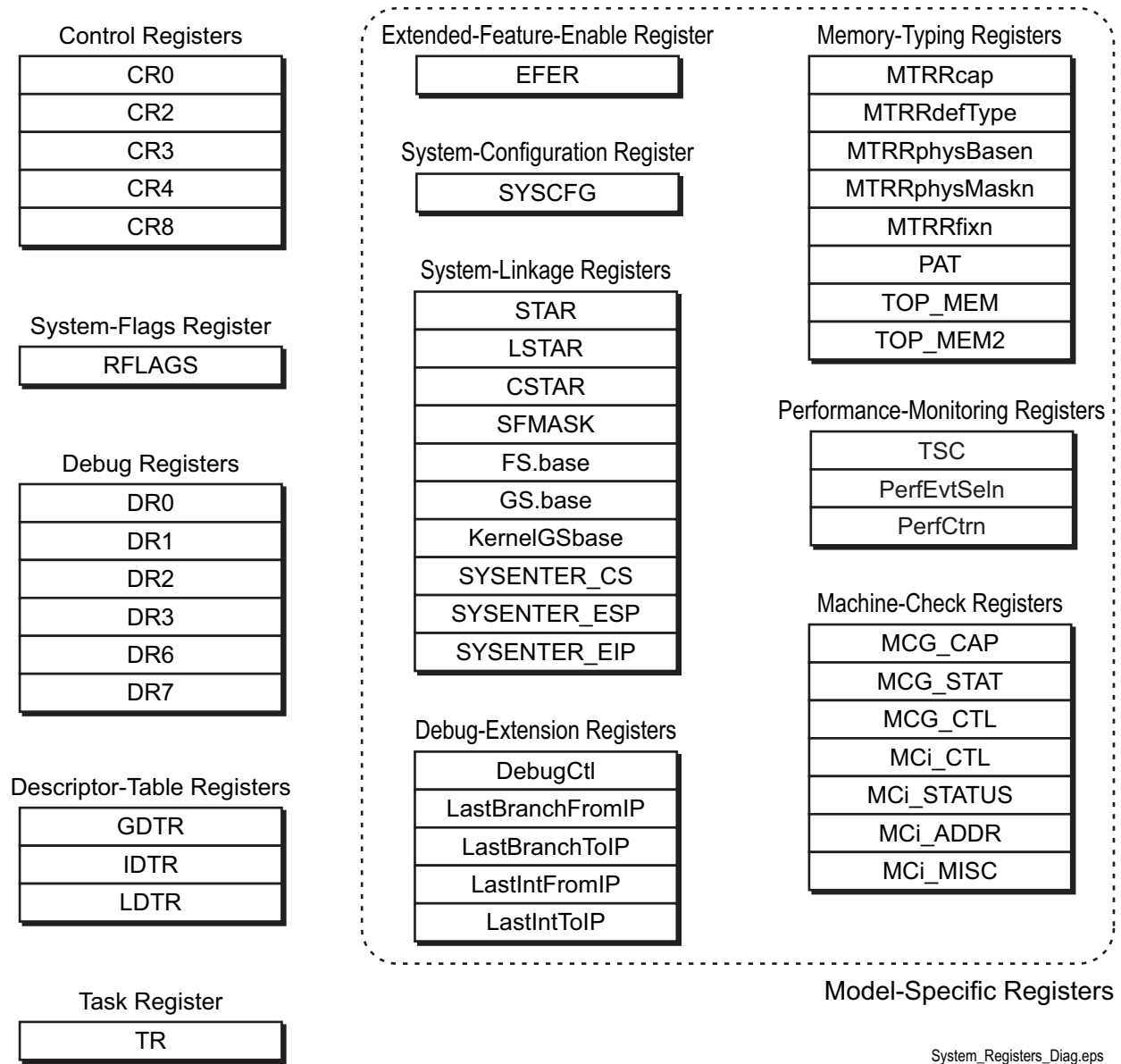
Figure 1-7. System Registers
