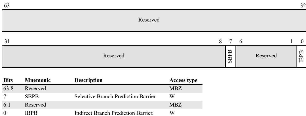
Figure 3-14. PRED_CMD Register
