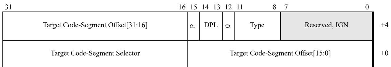
Figure 4-18. Interrupt-Gate and Trap-Gate Descriptors—Legacy Mode
