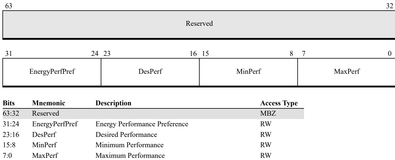
Figure 17-12. CPPC_REQUEST
