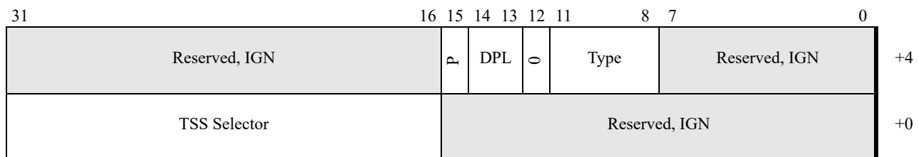
Figure 4-19. Task-Gate Descriptor—Legacy Mode
