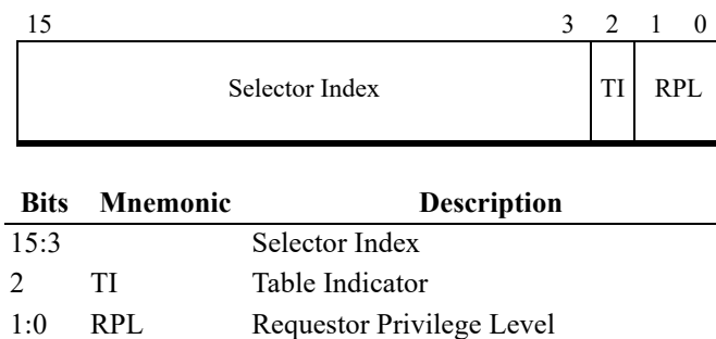
Figure 12-2. Task-Segment Selector
