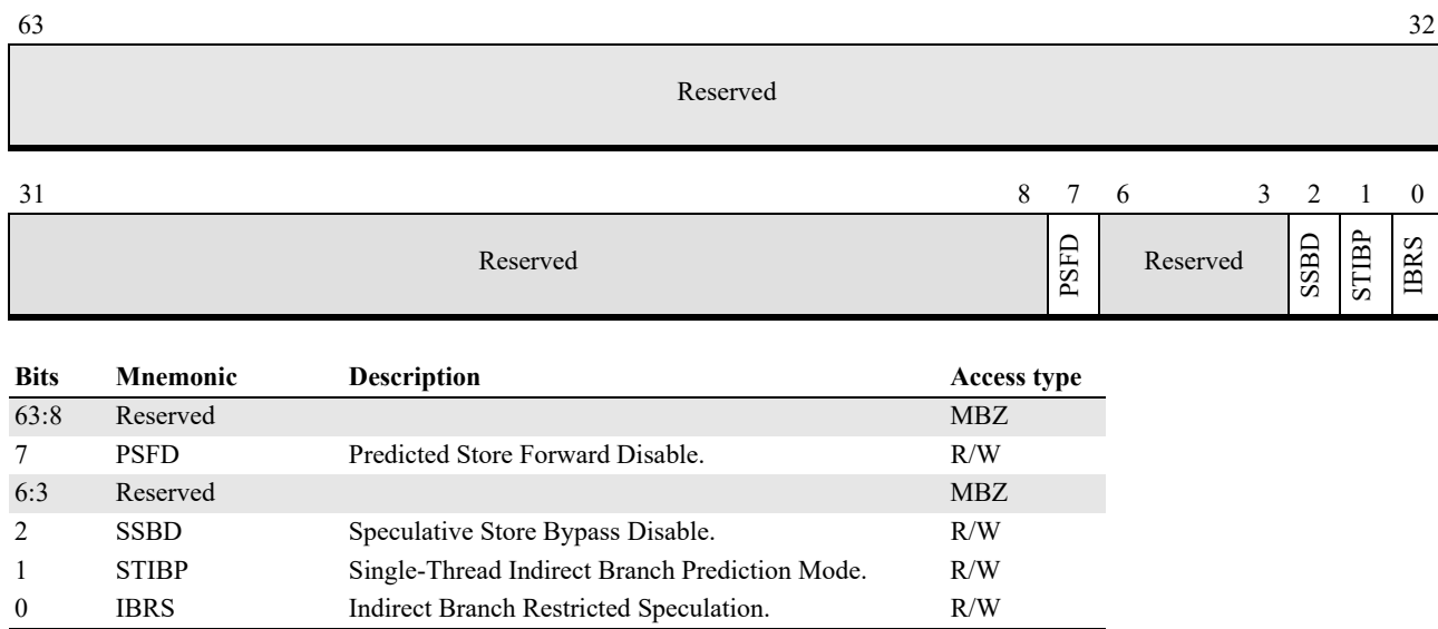
Figure 3-13. SPEC_CTRL Register
