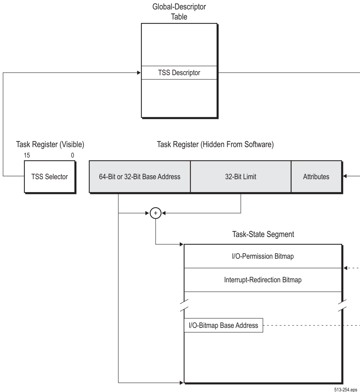
Figure 12-1. Task-Management Resources
