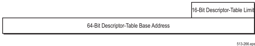
Figure 4-8. GDTR and IDTR Format—Long Mode
