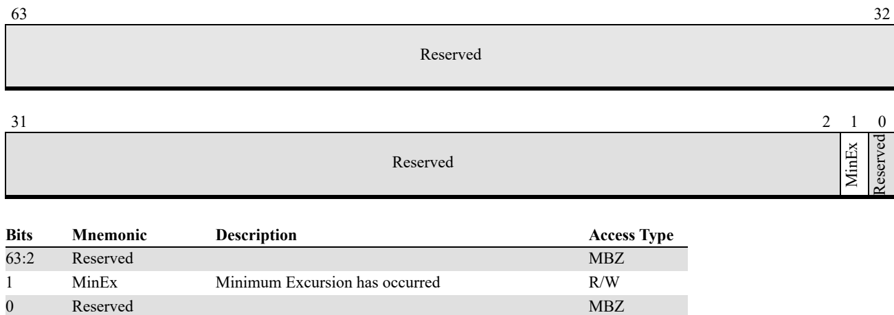
Figure 17-13. CPPC_STATUS
