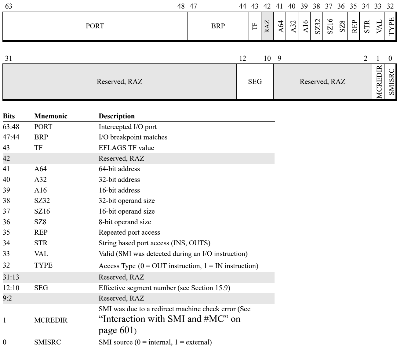
Figure 15-3. EXITINFO1 for SMI Intercept
