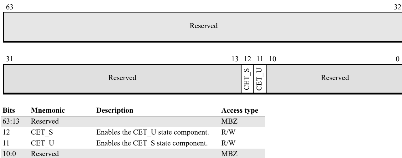
Figure 3-12. XSS Register
