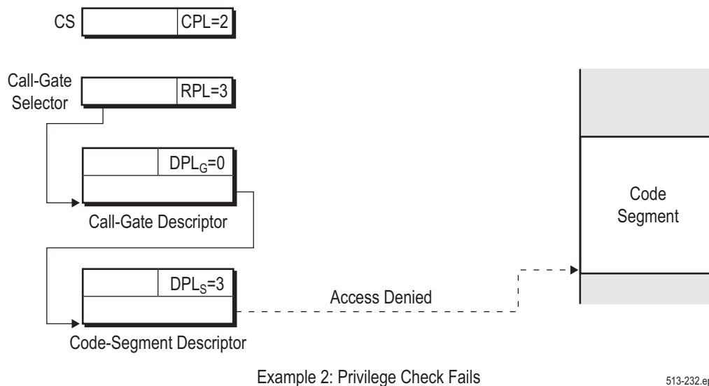
Figure 4-32. Privilege-Check Examples for Call Gates
