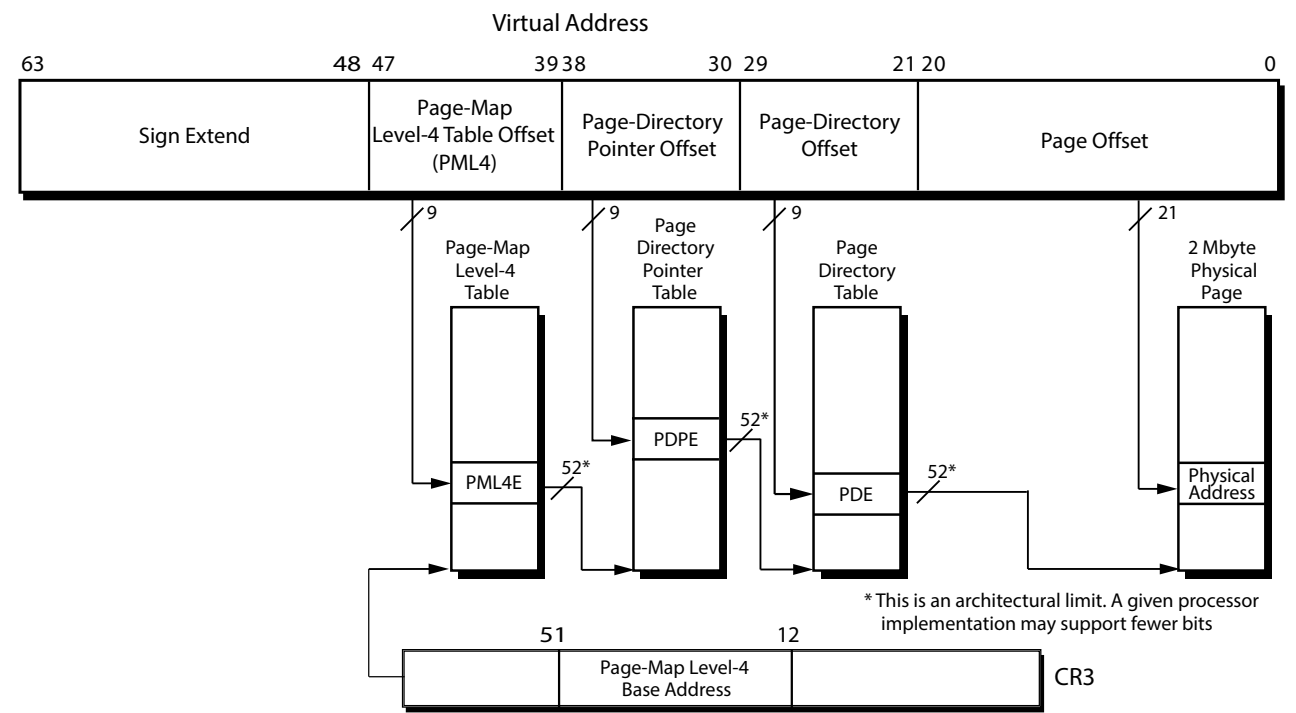
Figure 5-24. 2-Mbyte Page Translation—Long Mode 4-Level Paging
