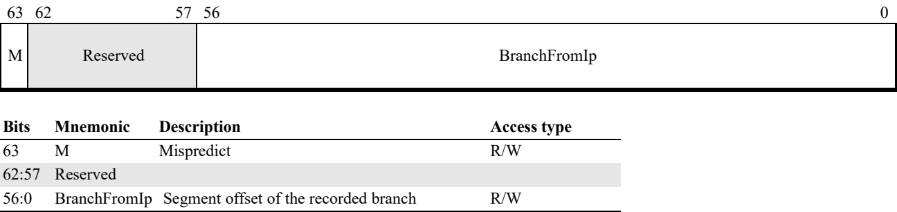
Figure 13-7. LastBranchStackFromIp MSR
