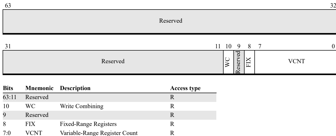
Figure 7-12. MTRR Capability Register Format
