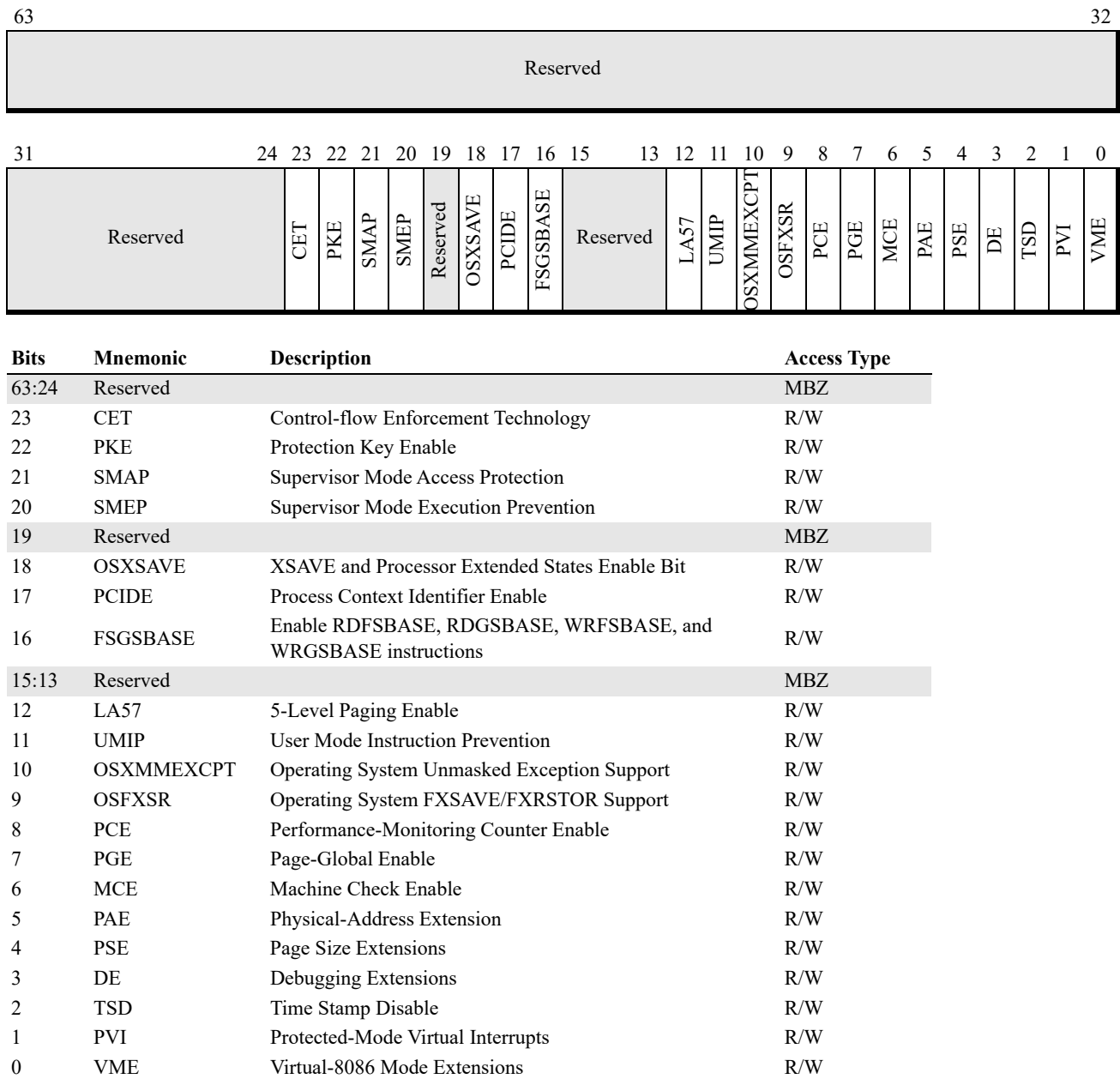
Figure 3-7. CR4 Register
