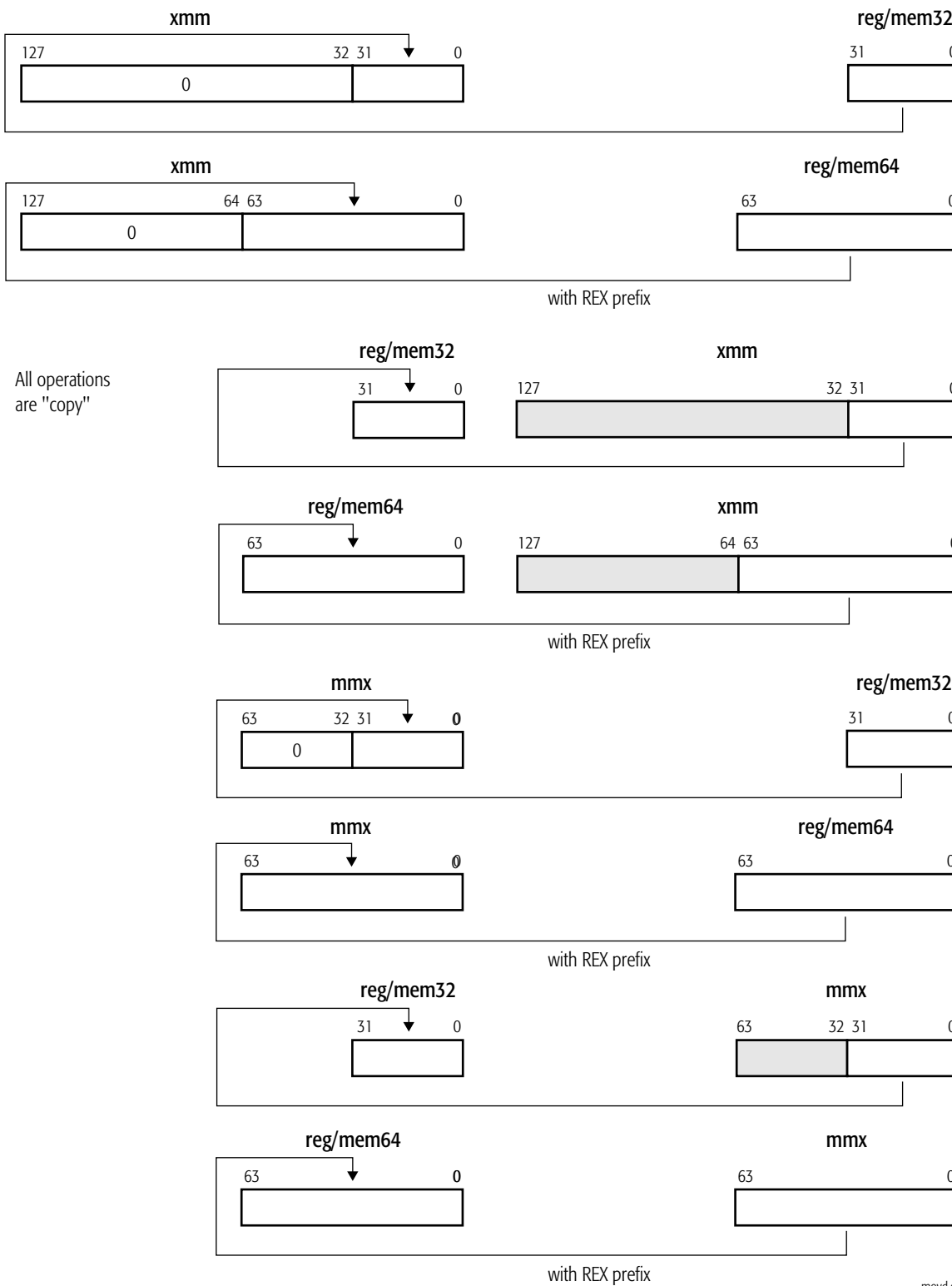
Figure 3-1. MOVQ Instruction Operation
