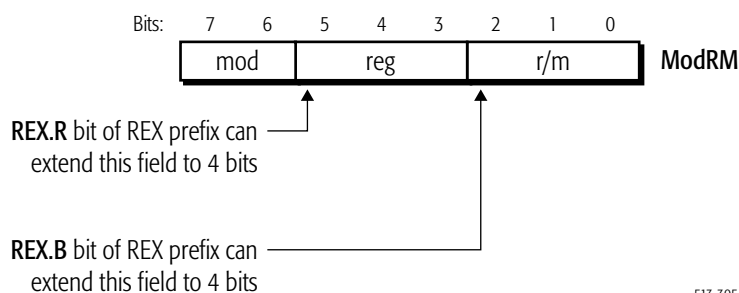
Figure 1-4. ModRM-Byte Format
