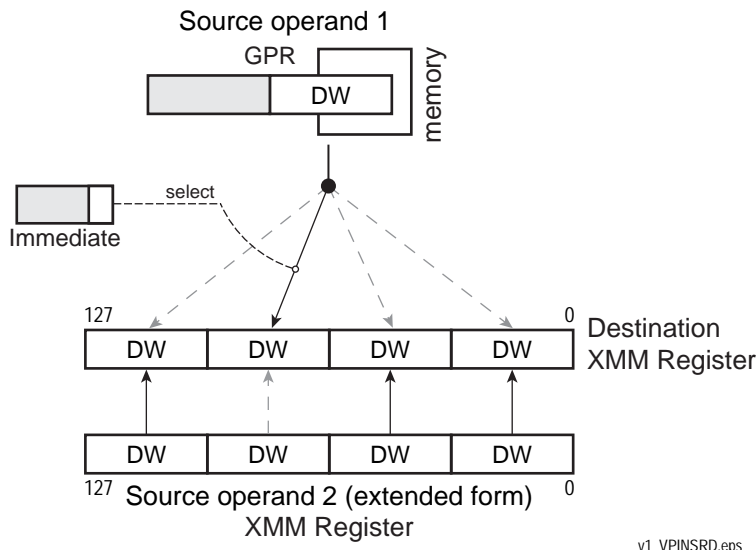
Figure 4-28. (V)PINSRD Operation
