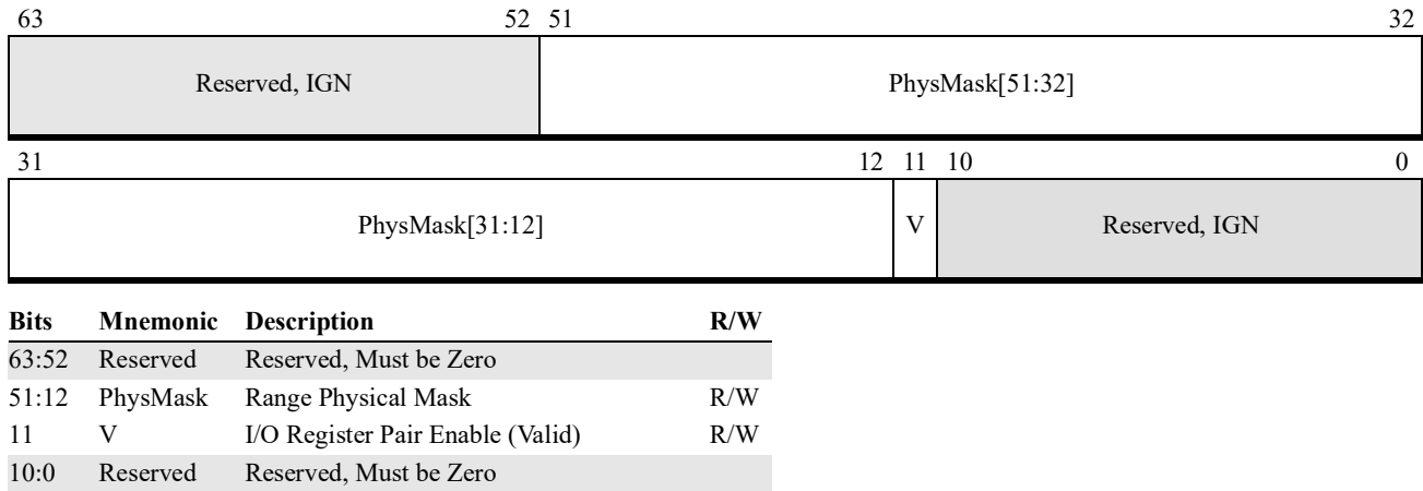
Figure 7-13. IORRMaskn Register
