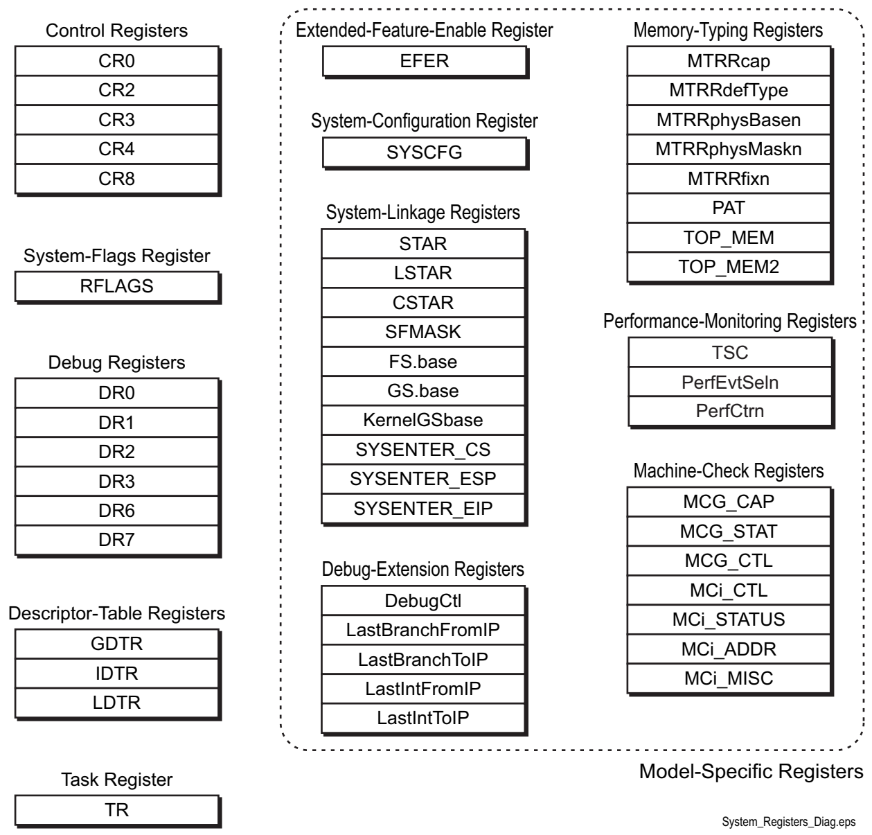
Figure 2-6. System Registers
