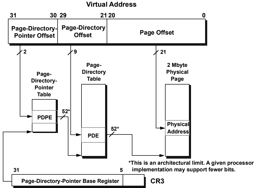
Figure 5-13. 2-Mbyte PAE Page Translation—Legacy Mode
