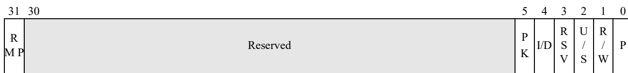
Figure 8-3. Page-Fault Error Code
