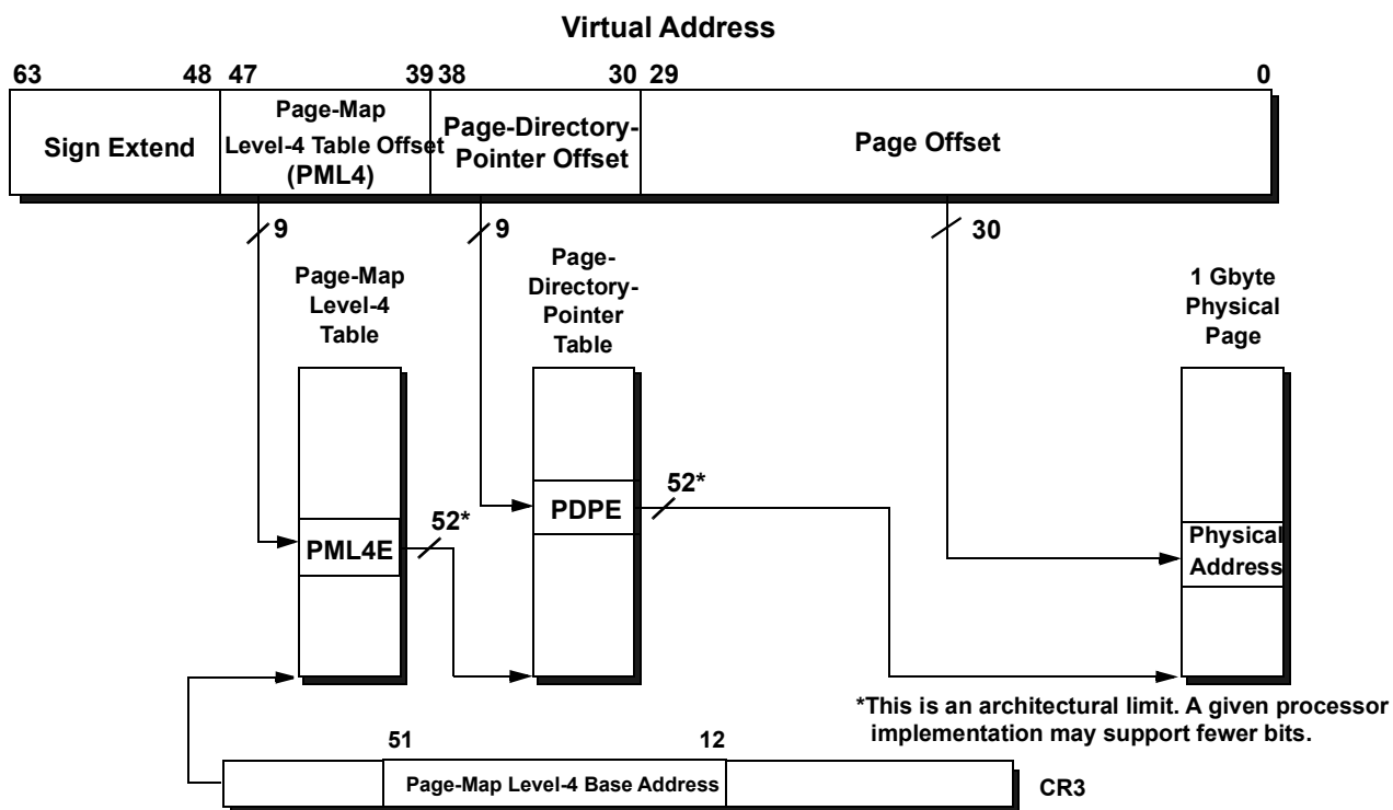
Figure 5-26. 1-Gbyte Page Translation—Long Mode
