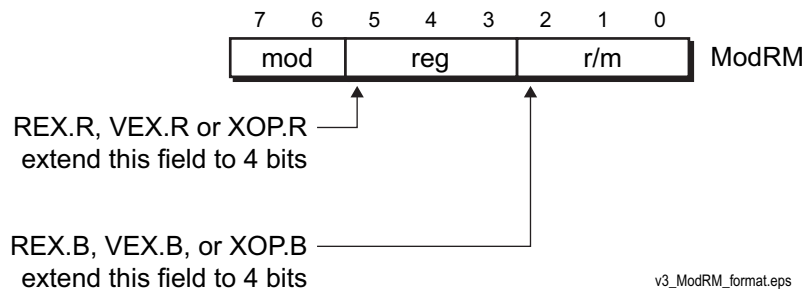
Figure 1-4. ModRM-Byte Format
