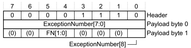
Figure D4-16 Exception trace packet format
