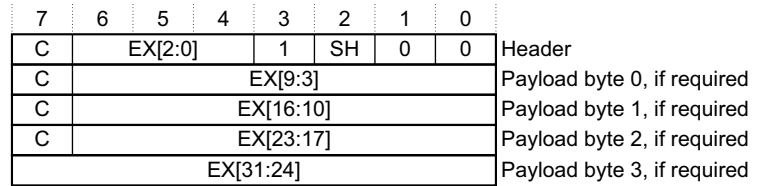
Figure D4-10 Extension packet format
