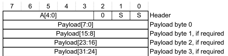
Figure D4-12 Instrumentation packet format
