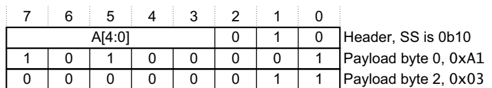
Figure D4-13 Instrumentation packet for a halfword write of 0x03A1
