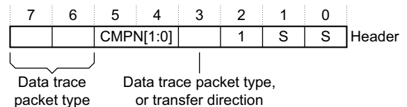
Figure D4-19 Data trace packet header format
