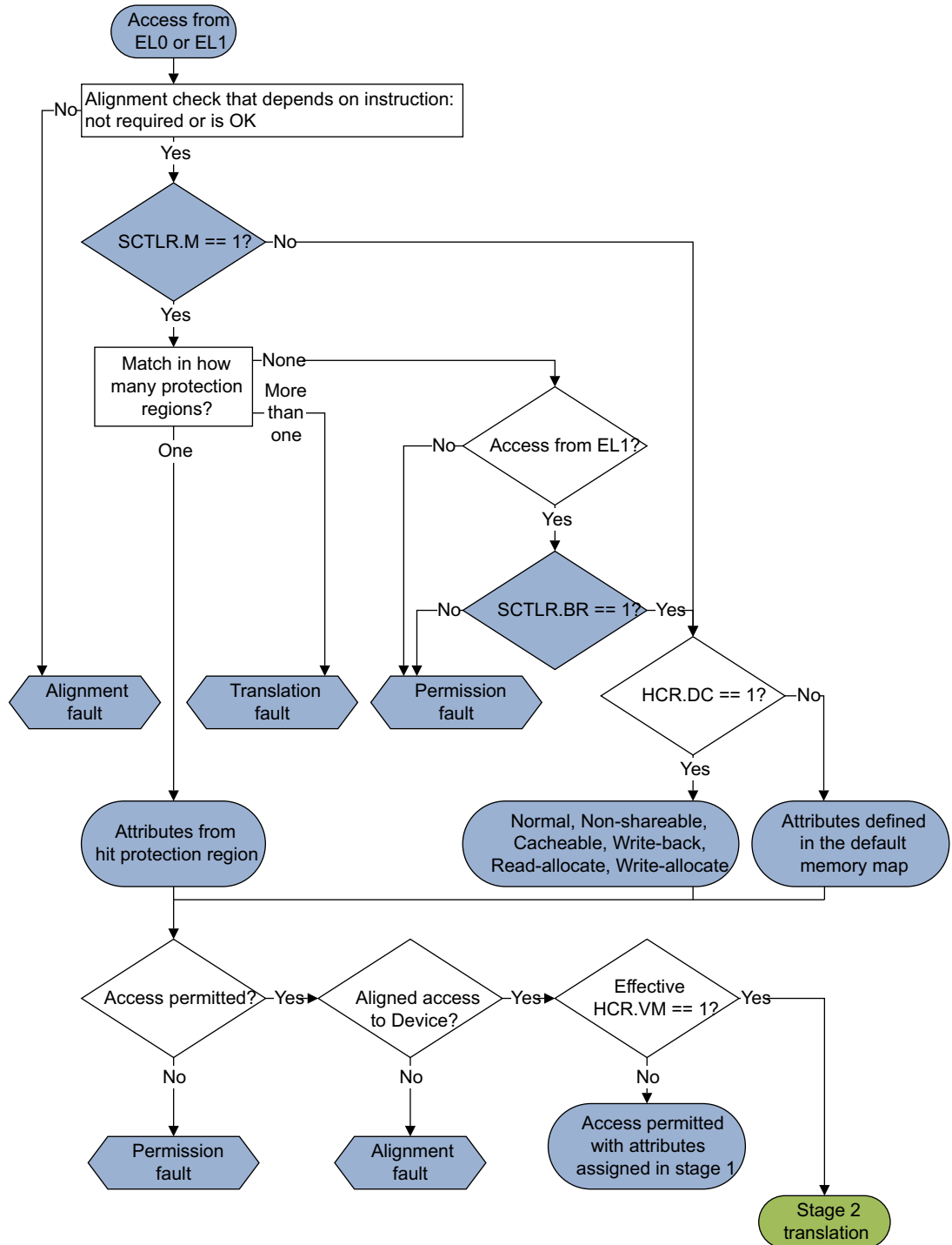
Figure C1-2 Stage 1 translation for EL1 and EL0 accesses
