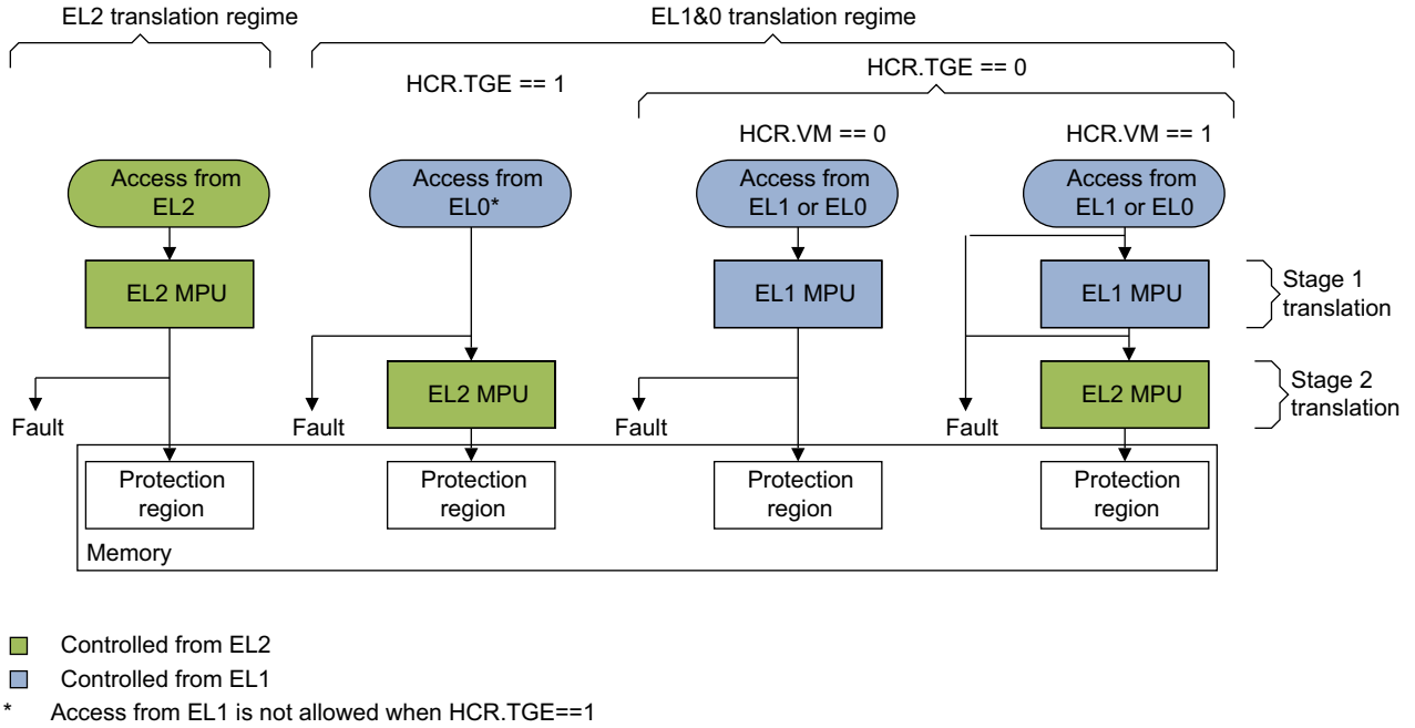
Figure C1-1 PMSAv8-32 memory access permission and attribute control
