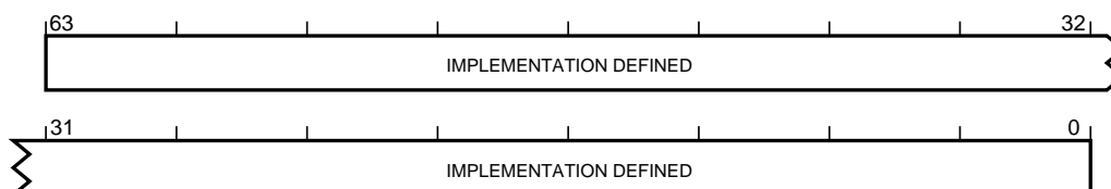
Figure 4.5: ERR<n>MISC0
