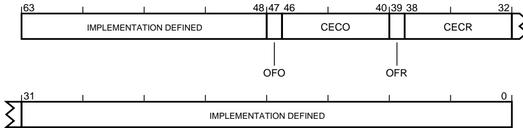
Figure 4.9: ERR<n>MISCO
