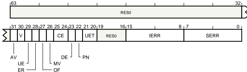
Figure 4.18: ERR<n>STATUS
