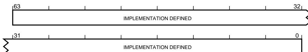
Figure 4.10: ERR<n>MISC1
