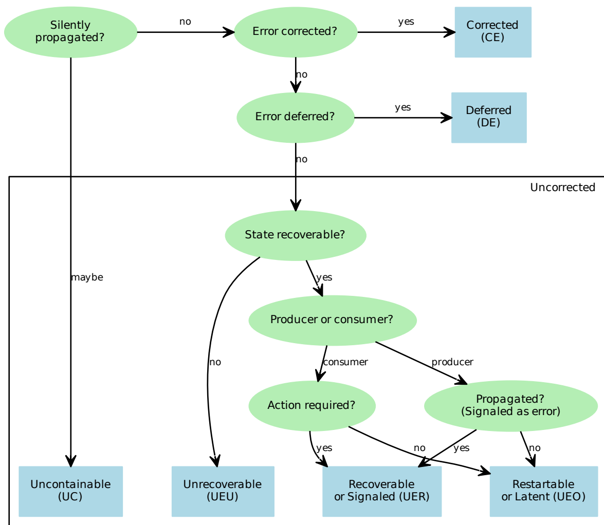
Figure 3.2: Component error state types
