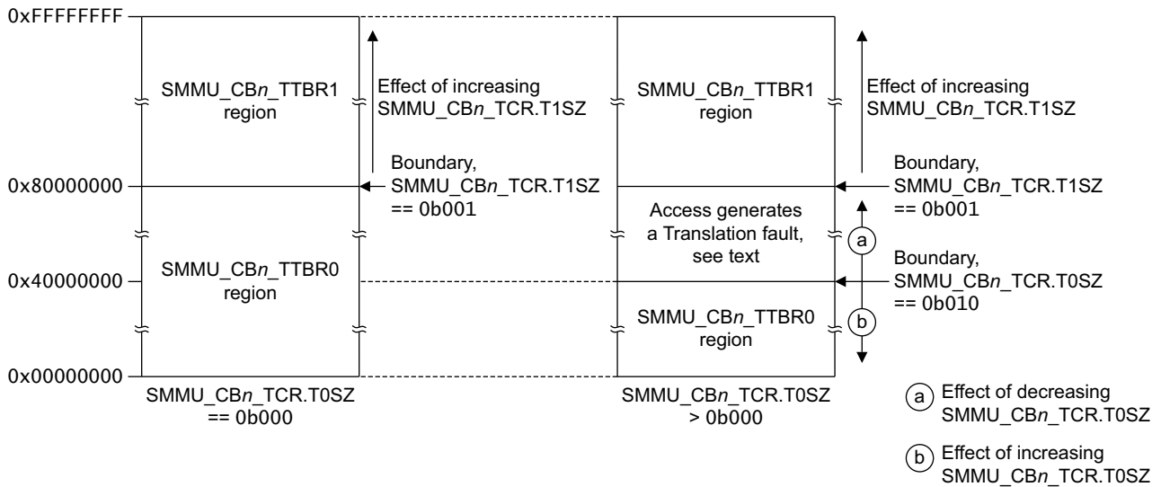
Figure 1-5 Control of TTBR0 and TTBR1 regions when SMMU_CBn_TCR.T1SZ is nonzero
