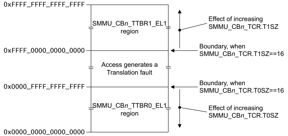
Figure 1-6 AArch64 TTBR boundaries and VA ranges
