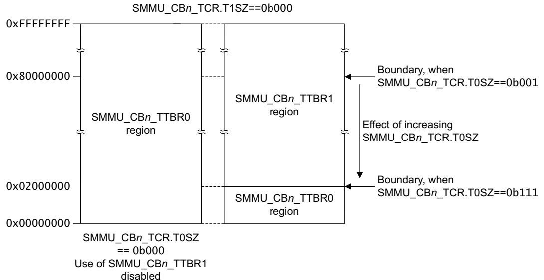
Figure 1-4 Control of TTBR0 and TTBR1 regions, when SMMU_CBN_TCR.T1SZ is zero
