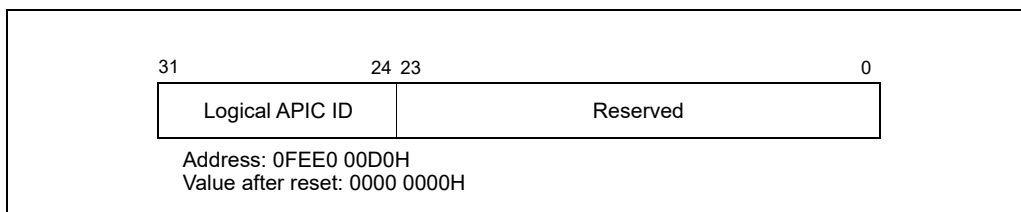
Figure 12-13. Logical Destination Register (LDR)
