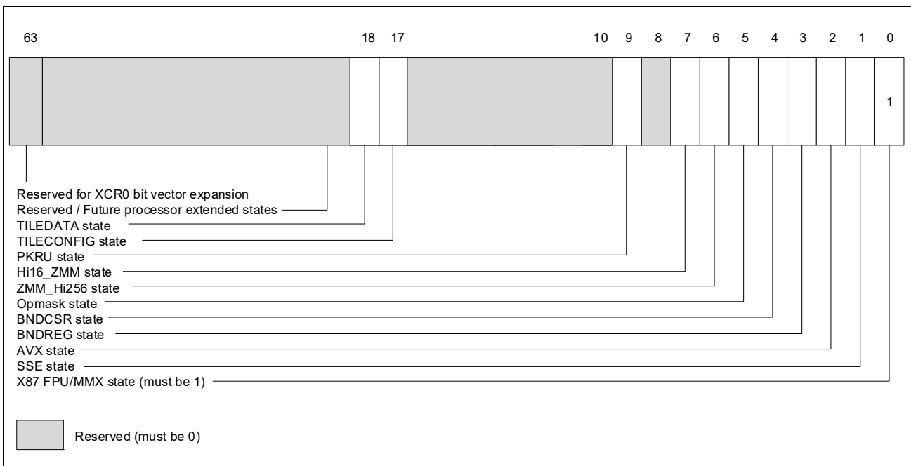
Figure 2-8. XCR0
