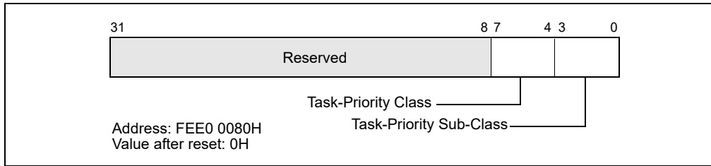
Figure 12-18. Task-Priority Register (TPR)
