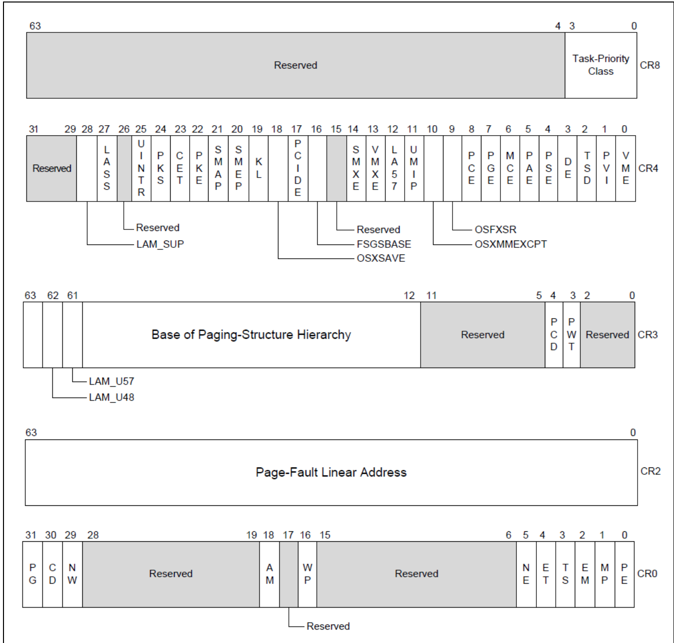
Figure 2-7. Control Registers
