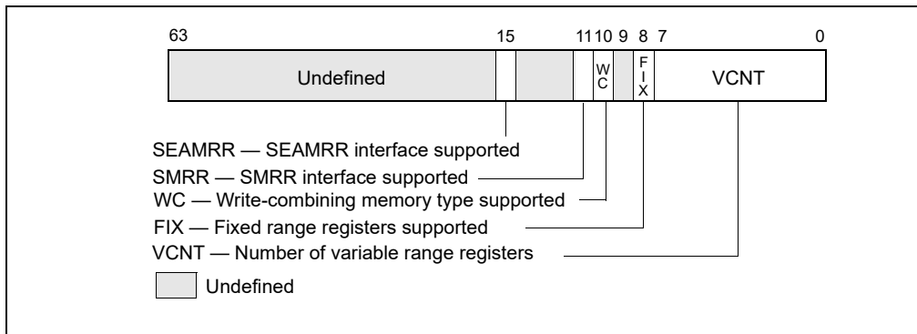
Figure 13-5. IA32_MTRRCAP Register
