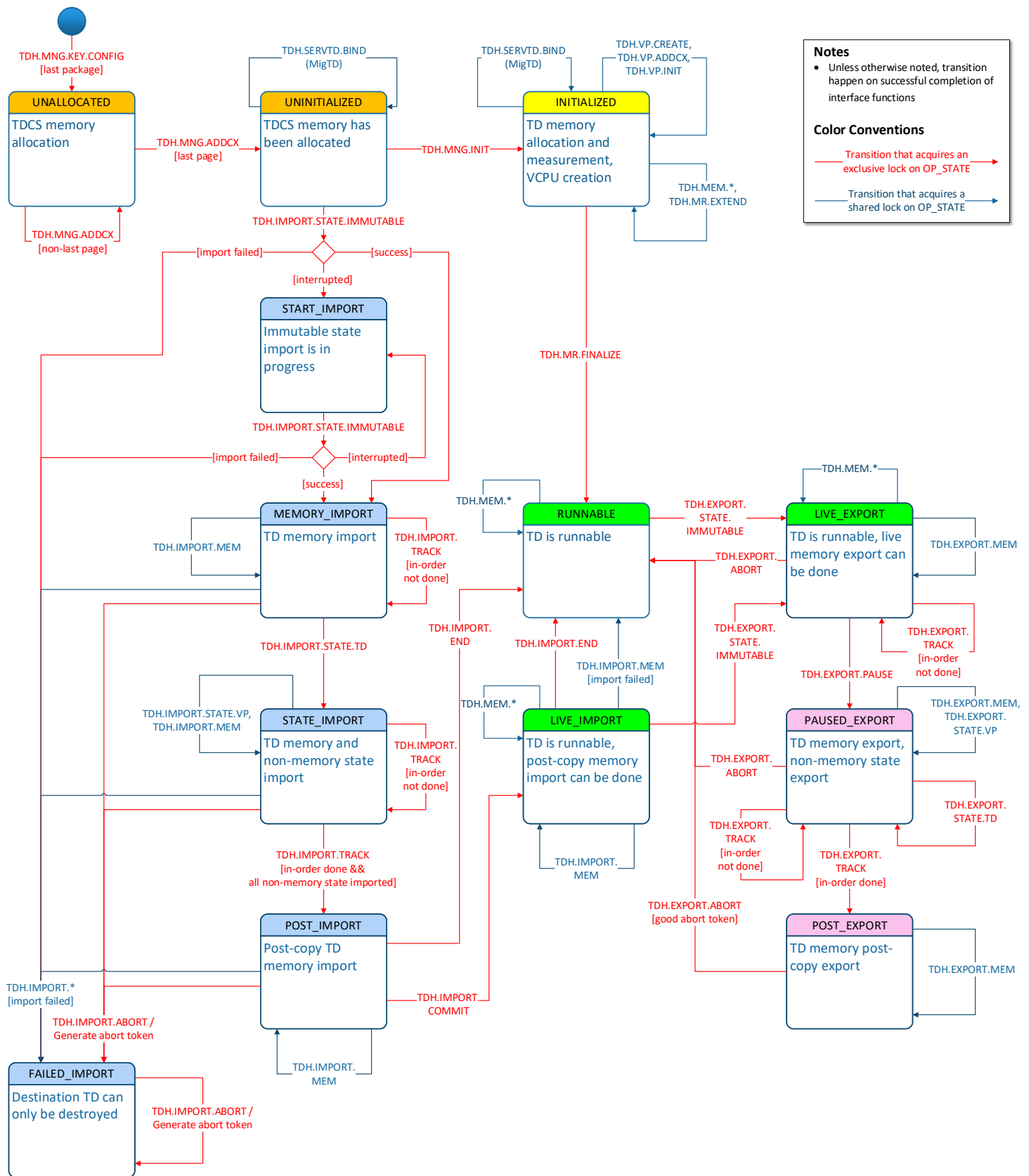
Figure 6.8: TD Operation State Machine (Sub-States of TD_KEYS_CONFIGURED)
