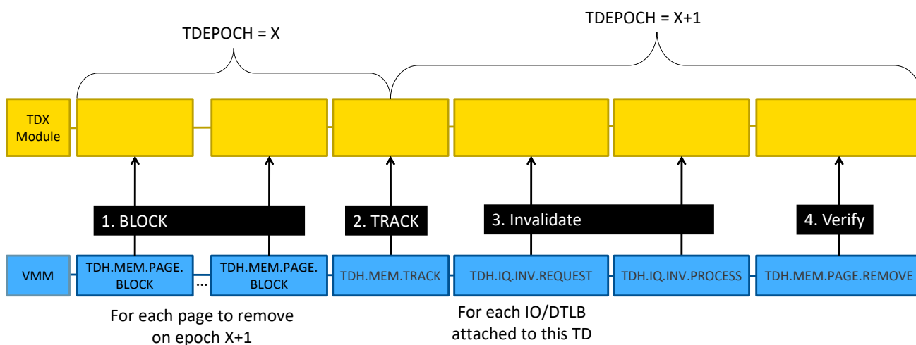
Figure 2.11: TD Memory Management with IOTLB Tracking
