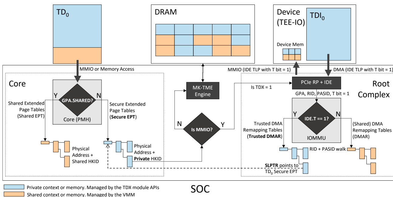
Figure 2.2: Trusted DMA and Secure-EPT
