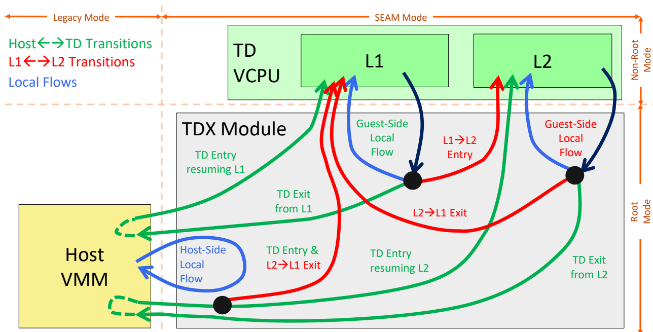
Figure 11.5: TDX Transitions
