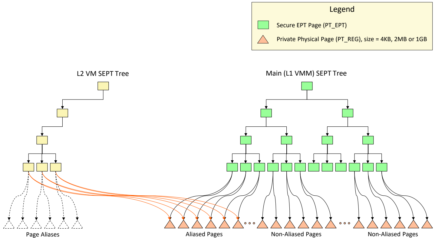
Figure 21.2: Page Aliasing
