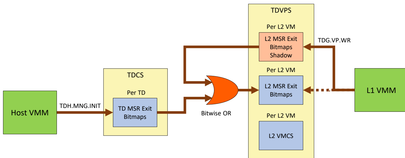
Figure 23.1: MSR Virtualization Policy Configuration
