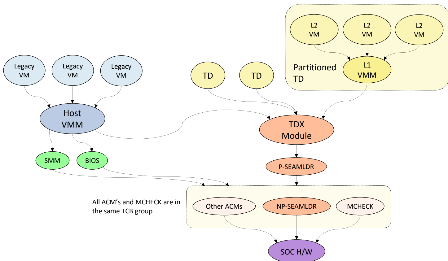
Figure 11.3: TDX TCB Dependency Diagram
