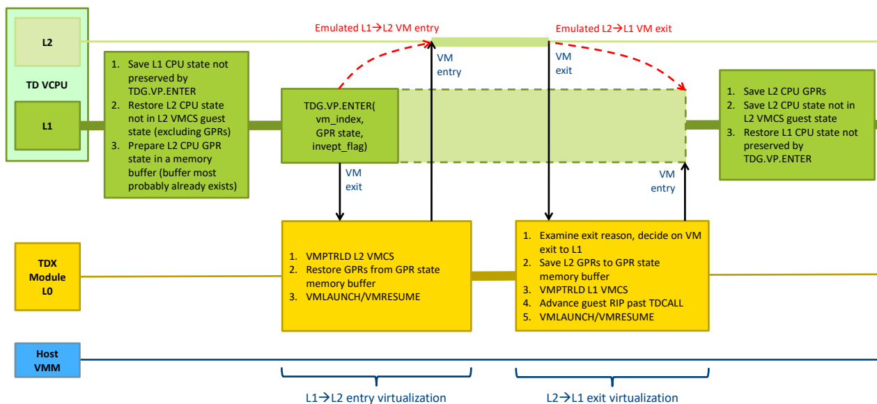
Figure 22.2: Example of L1→L2 VM Entry and Exit
