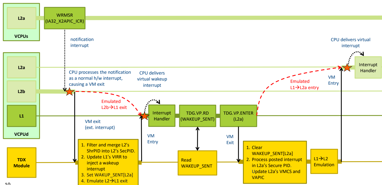
Figure 5.5: Example of a Wakeup Interrupt when the Destination VCPU is Running in Another L2
