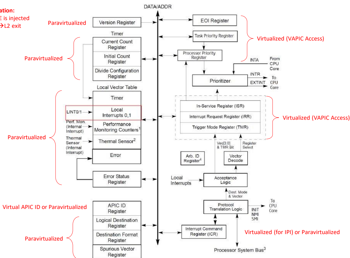
Figure 3.1: Virtual APIC Access by Guest TD
