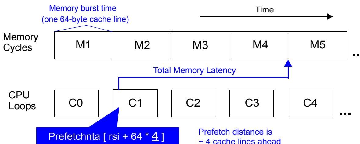
Figure 5. Memory-Limited Code
