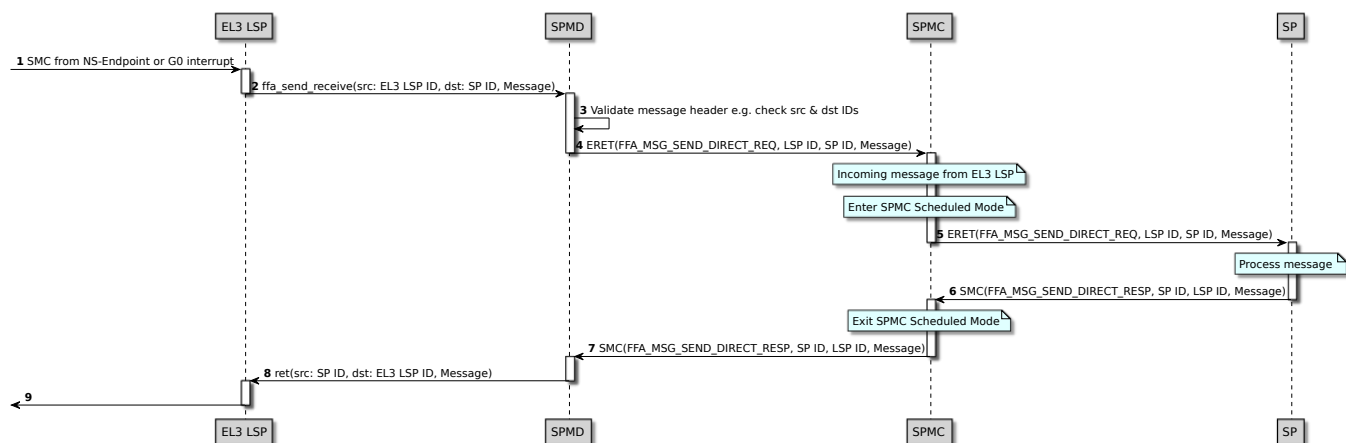
Figure 7.4: Example EL3 LSP Messaging Sequence
