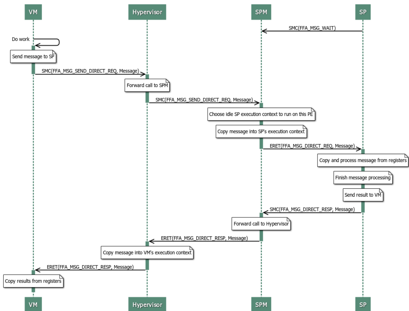
Figure 7.3: Example Direct message exchange between a VM and SP
