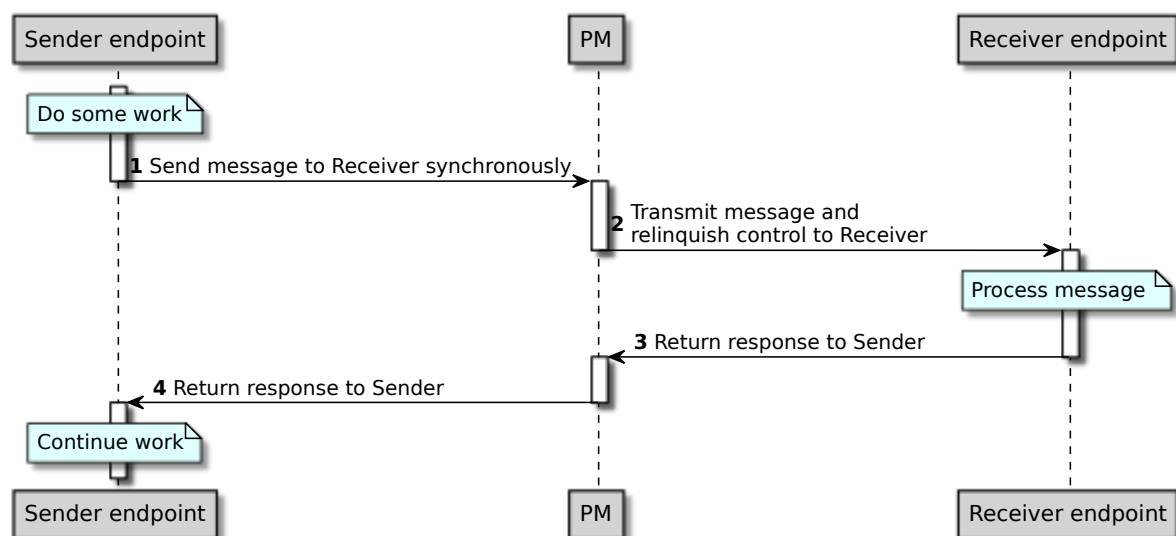
Figure 7.1: Example synchronous message exchange
