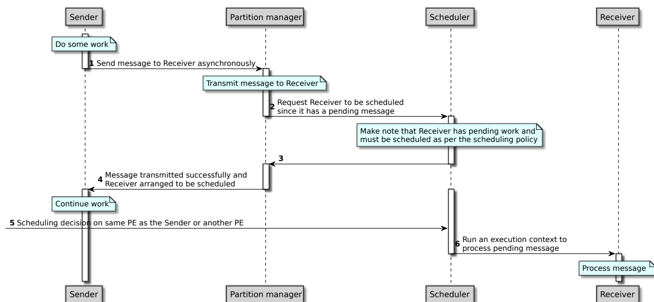
Figure 7.2: Example asynchronous message exchange
