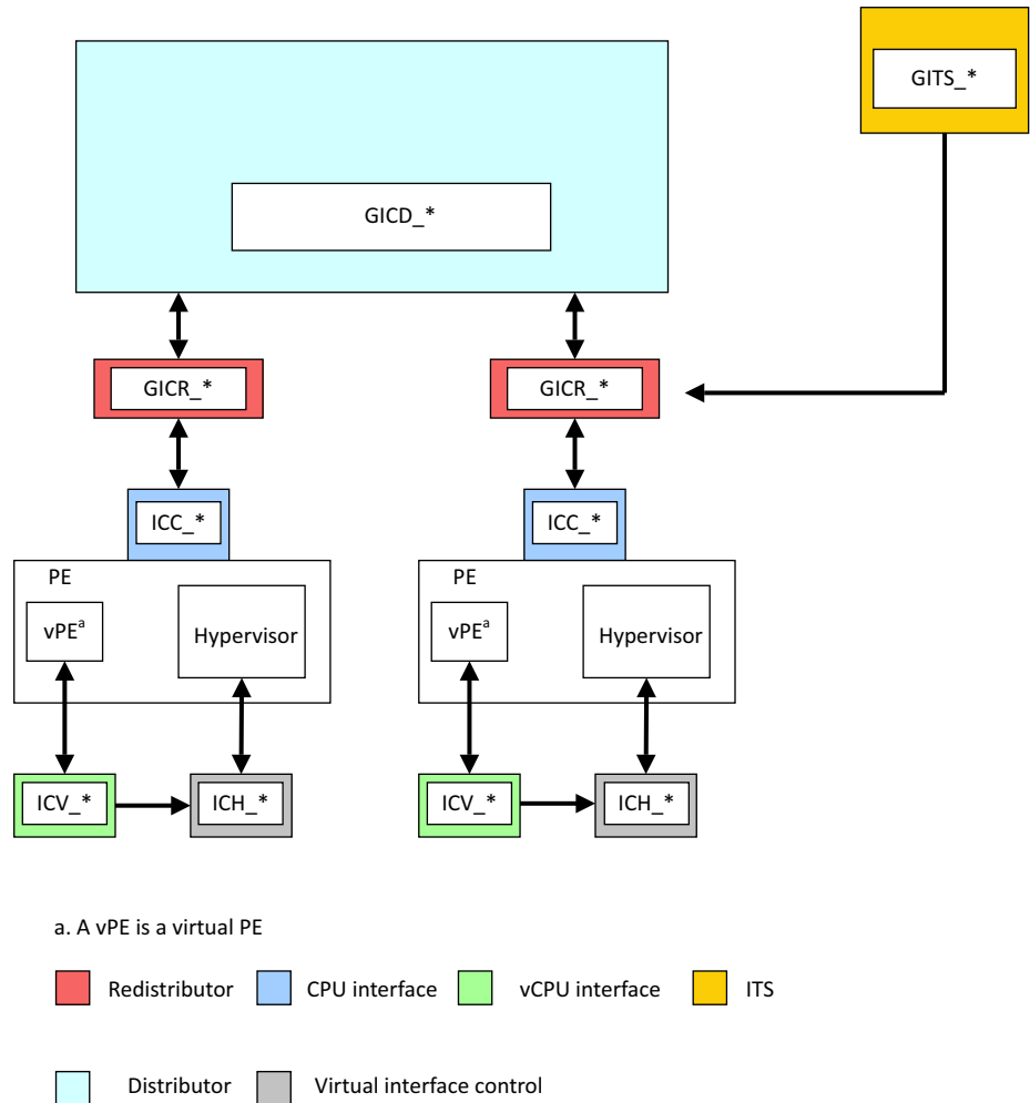
Figure 9-1 Register interfaces without legacy support (GICv3 only)
