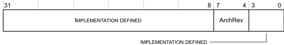
Figure 9-2 GICD_PIDR2 bit assignments
