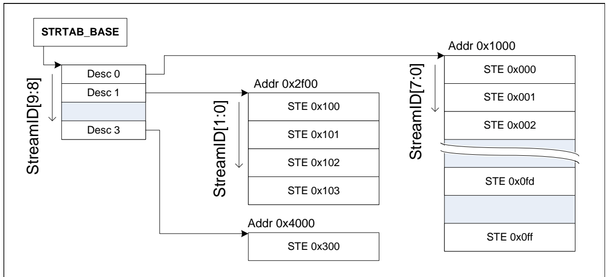
Figure 3.2: Example Two level Stream table with SPLIT == 8
