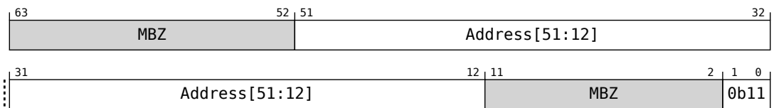
Figure 3.12: Level 0 Table entry
