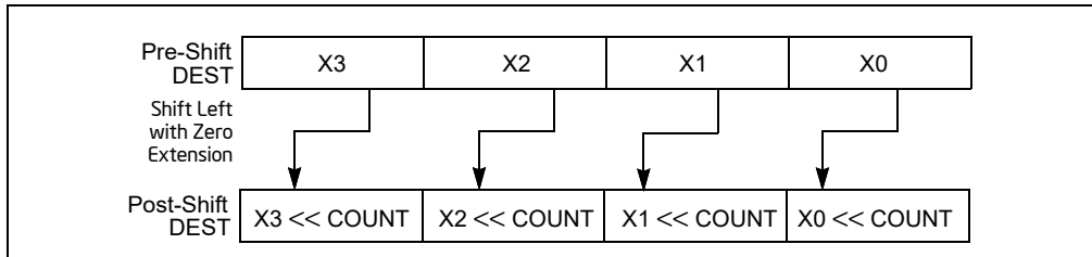
Figure 1-17. PSSLW, PSLLD, and PSLLQ Instruction Operation Using 64-bit Operand
