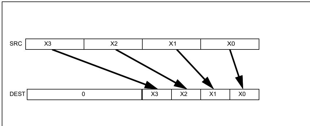
Figure 1-5. VCVTTPD2DQ (VEX.256 Encoded Version)
