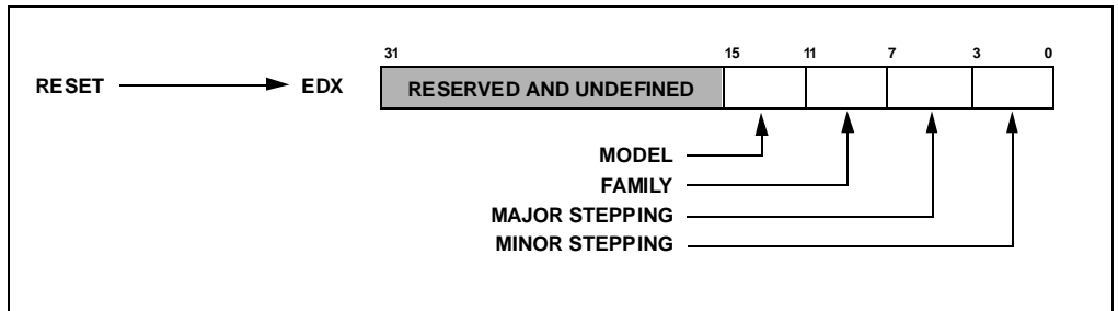
Figure 2. Processor Signature Format on Intel386™ Processors
