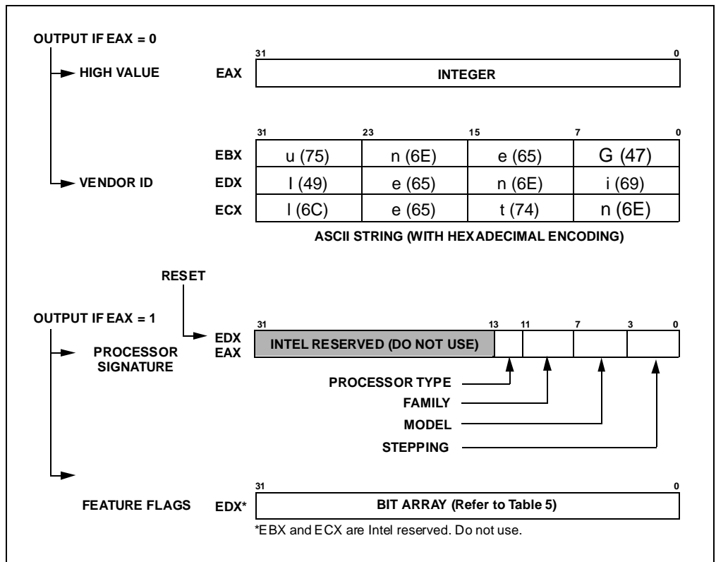
Figure 1. CPUID Instruction Outputs
