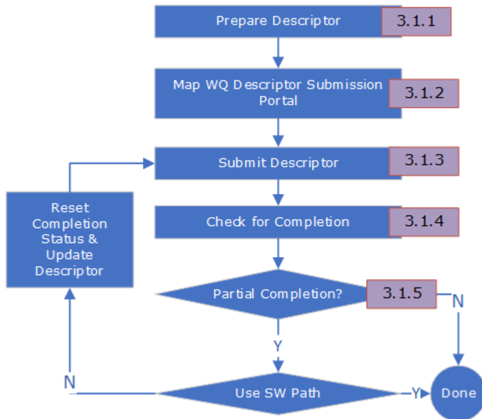
Figure 4-1. Descriptor Processing Sequence
