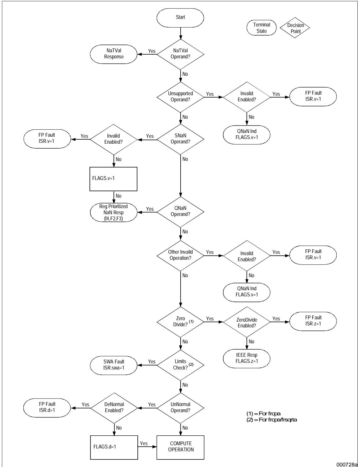
Figure 5-11. Floating-point Exception Fault Prioritization
