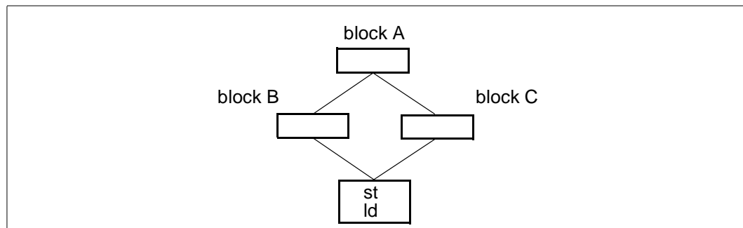
Figure 3-3. Minimizing Code Size During Speculation
