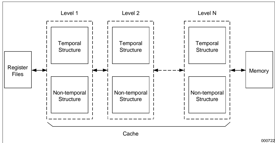
Figure 4-4. Memory Hierarchy
