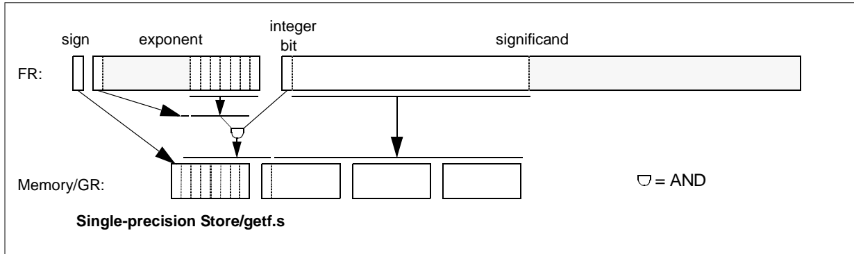
Figure 5-7. Floating-point Register to Memory Data Translation – Single Precision
