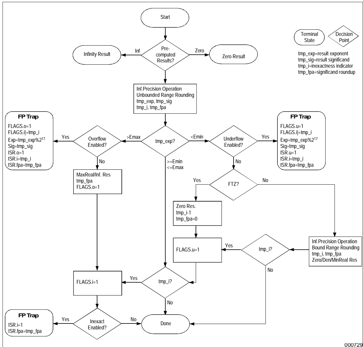
Figure 5-12. Floating-point Exception Trap Prioritization
