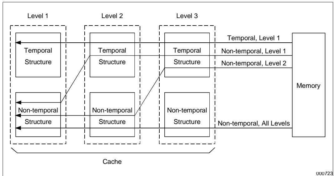
Figure 4-5. Allocation Paths Supported in the Memory Hierarchy
