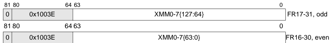
Figure 6-13. Streaming SIMD Extension Registers (XMM0-XMM7)
