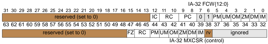
Figure 6-8. IA-32 Floating-point Control Register (FCR)
