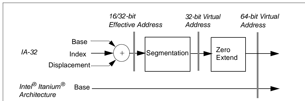
Figure 6-14. Memory Addressing Model
