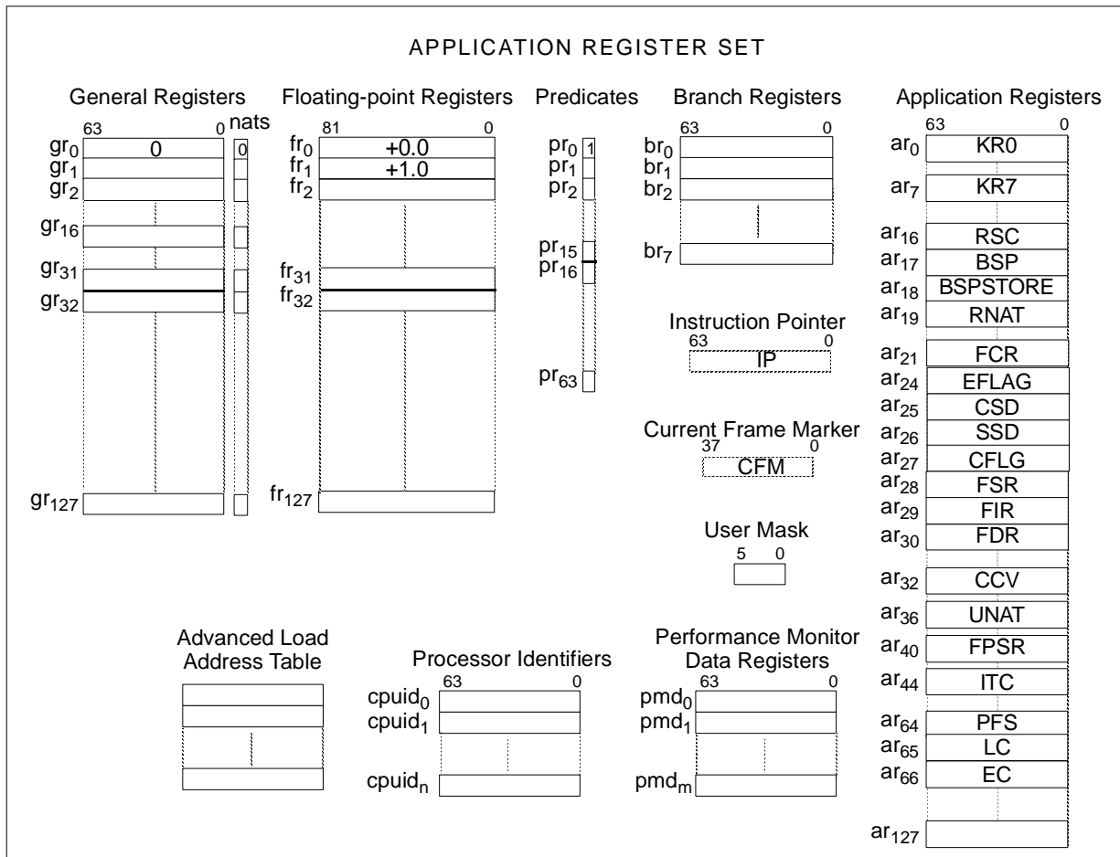
Figure 3-1. Application Register Model
