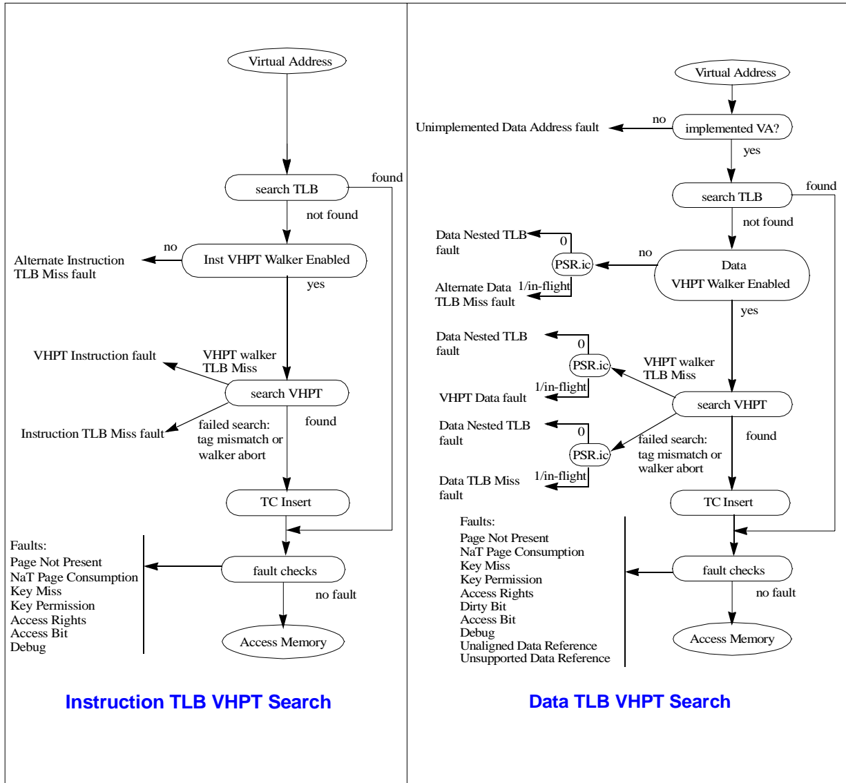
Figure 4-16. TLB/VHPT Search
