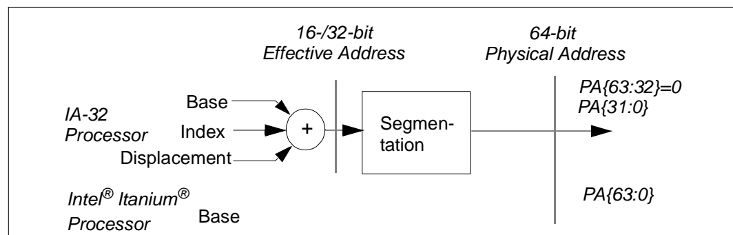
Figure 10-5. Physical Memory Addressing
