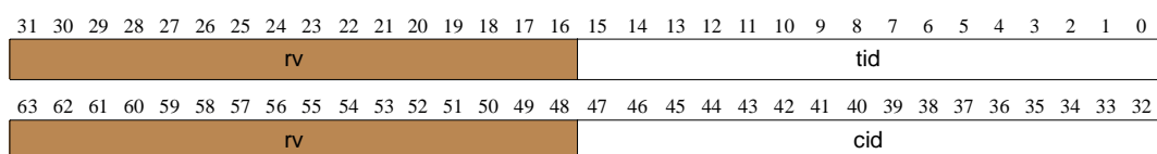
Figure 11-33. Layout of proc_n_log_info1 Return Value
