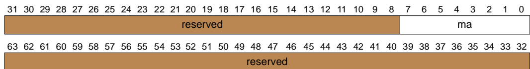
Figure 11-42. Layout of attrib Return Value
