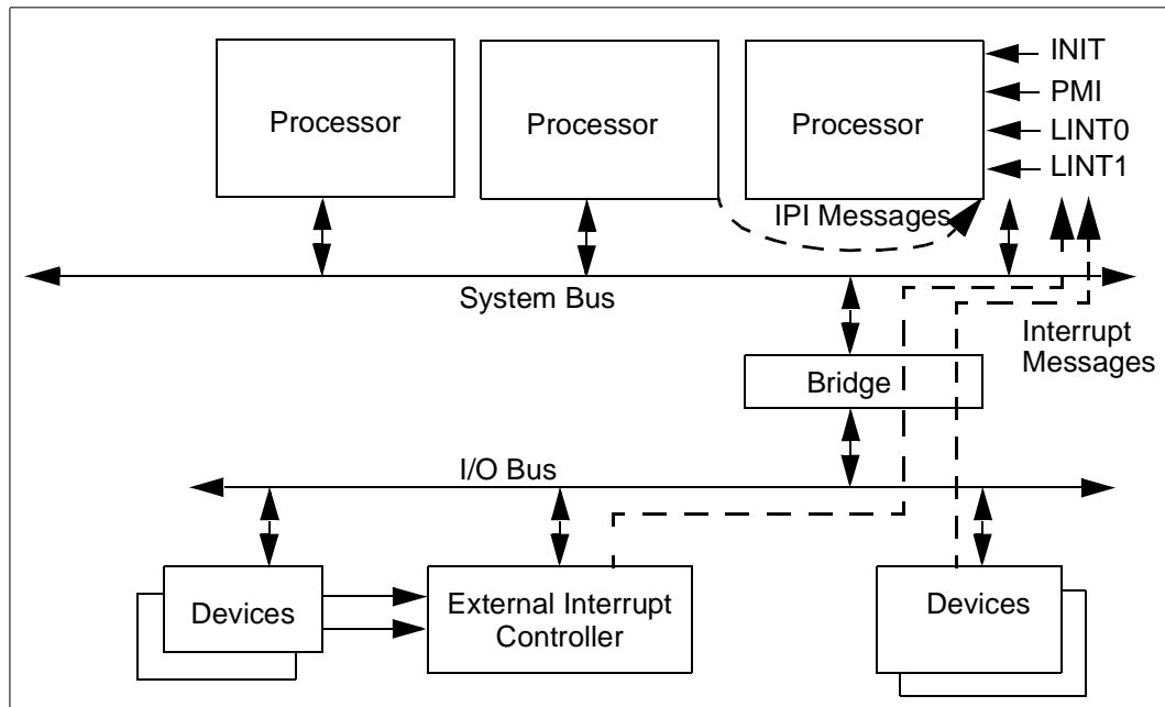
Figure 5-3. Interrupt Architecture Overview
