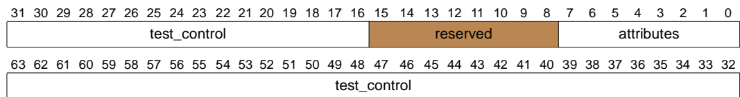
Figure 11-46. Layout of test_param Argument
