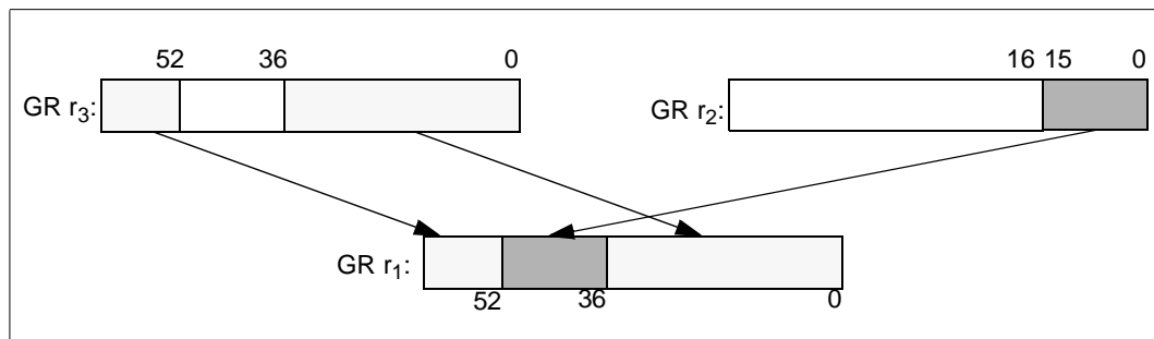
Figure 2-5. Deposit Example (merge_form)
