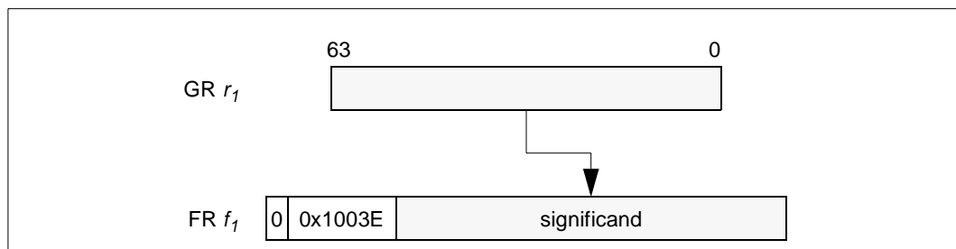
Figure 2-42. Function of setf.sig
