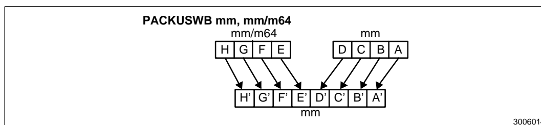
Figure 2-4. Operation of the PACKUSWB Instruction
