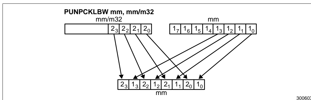
Figure 2-23. Low-order Unpacking and Interleaving of Bytes with the PUNPCKLBW Instruction
