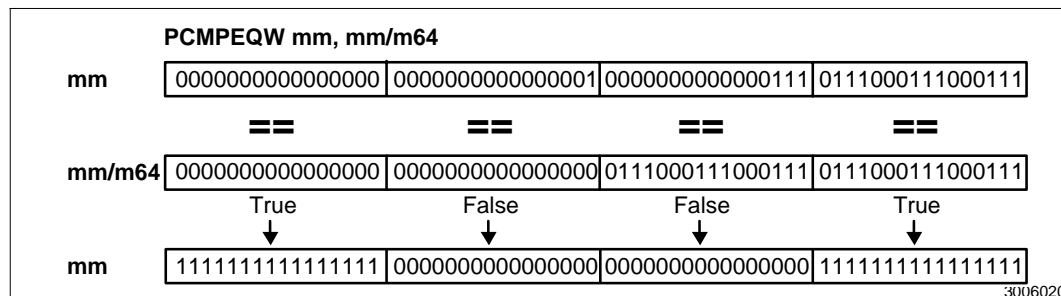
Figure 2-10. Operation of the PCMPEQW Instruction
