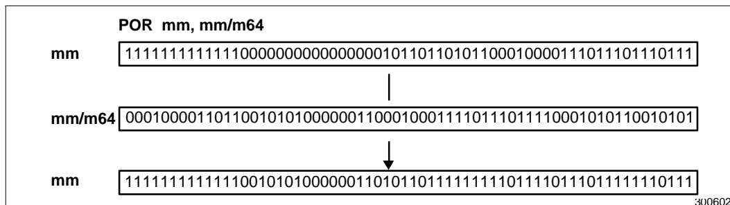
Figure 2-15. Operation of the POR Instruction.
