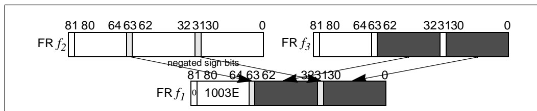
Figure 2-16. Floating-point Parallel Merge Sign Operation
