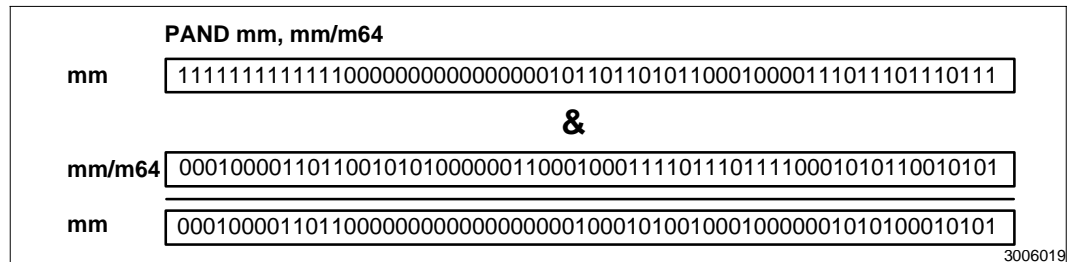
Figure 2-8. Operation of the PAND Instruction
