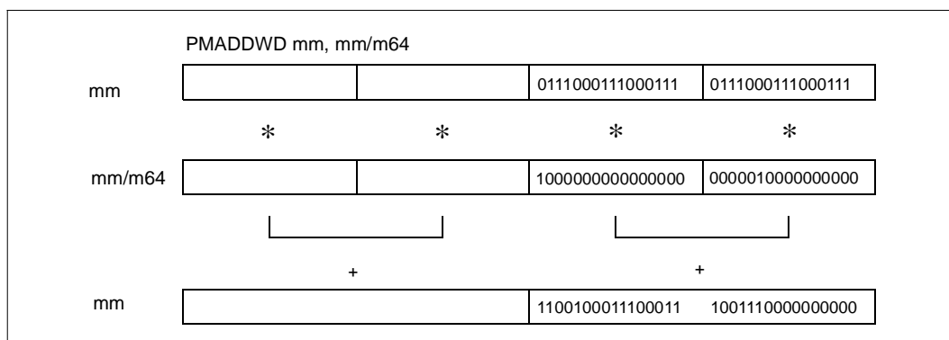
Figure 2-12. Operation of the PMADDWD Instruction
