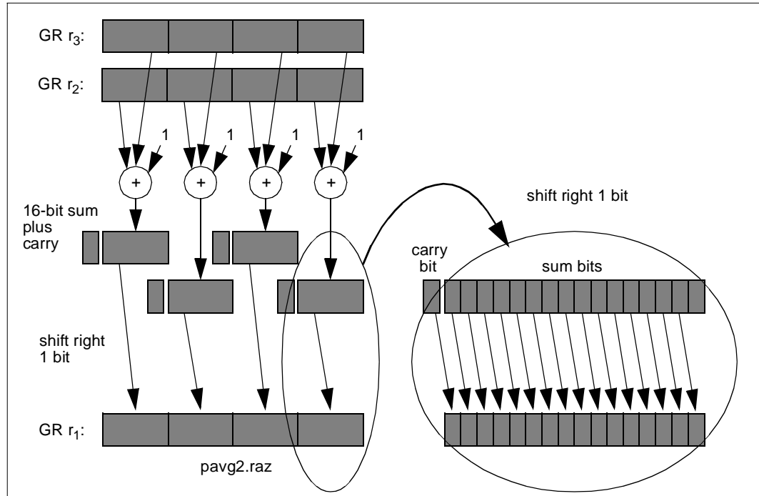
Figure 2-31. Parallel Average with Round Away from Zero Example
