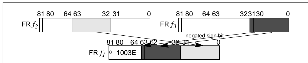
Figure 2-20. Floating-point Swap Negate Right
