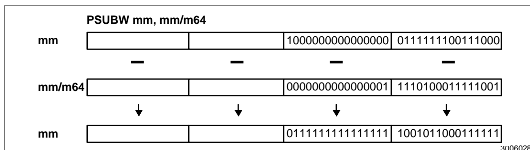
Figure 2-19. Operation of the PSUBW Instruction
