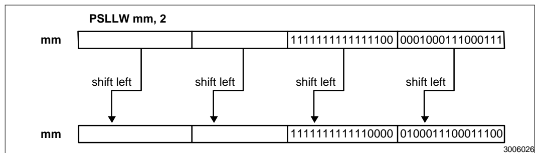
Figure 2-16. Operation of the PSLLW Instruction
