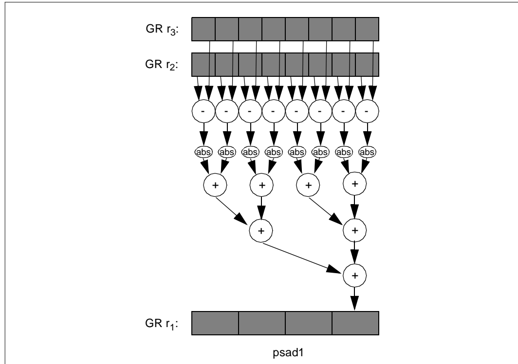
Figure 2-38. Parallel Sum of Absolute Difference Example
