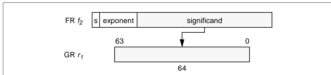
Figure 2-24. Function of getf.sig
