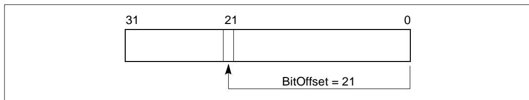
Figure 1-1. Bit Offset for BIT[EAX,21]
