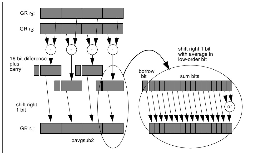
Figure 2-32. Parallel Average Subtract Example
