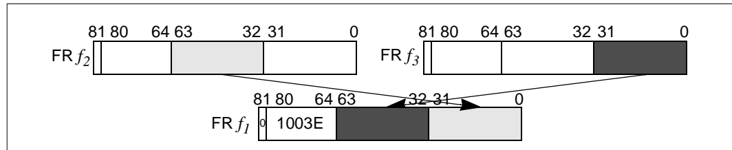
Figure 2-19. Floating-point Swap Negate Left
