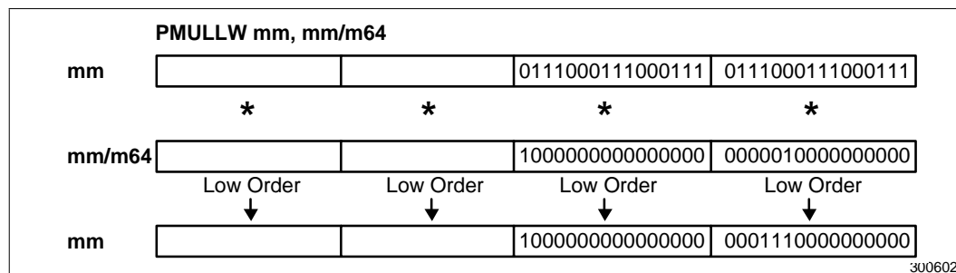
Figure 2-14. Operation of the PMULLW Instruction
