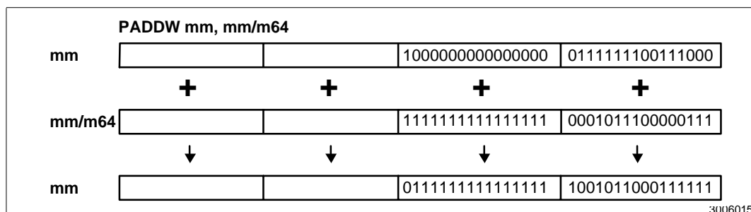
Figure 2-5. Operation of the PADDW Instruction
