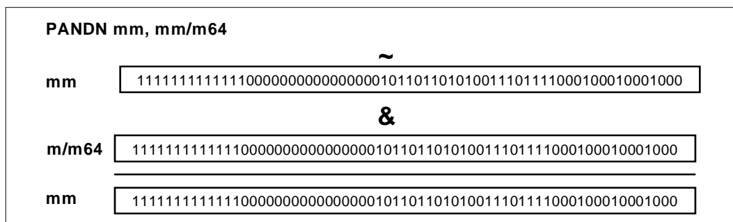
Figure 2-9. Operation of the PANDN Instruction
