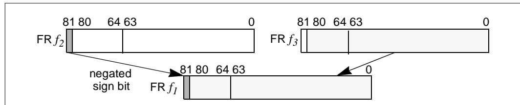
Figure 2-9. Floating-point Merge Sign Operation
