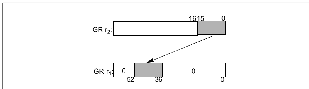
Figure 2-6. Deposit Example (zero_form)
