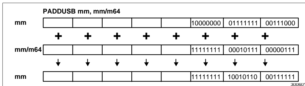
Figure 2-7. Operation of the PADDUSB Instruction
