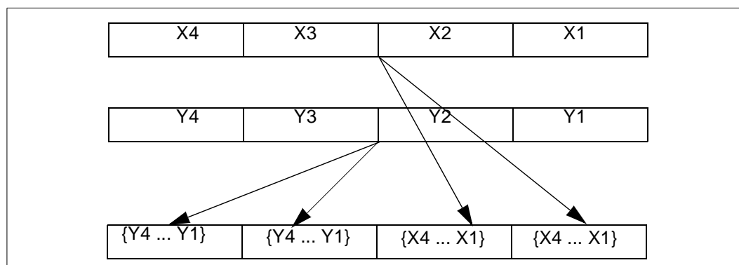
Figure 3-5. Packed Shuffle Operation
