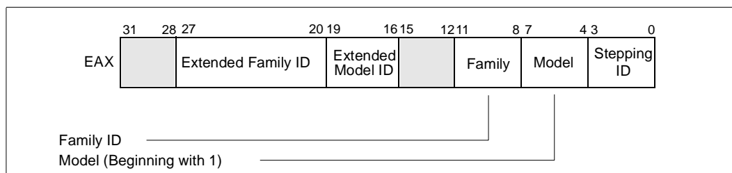
Figure 1-3. Version Information in Registers EAX
