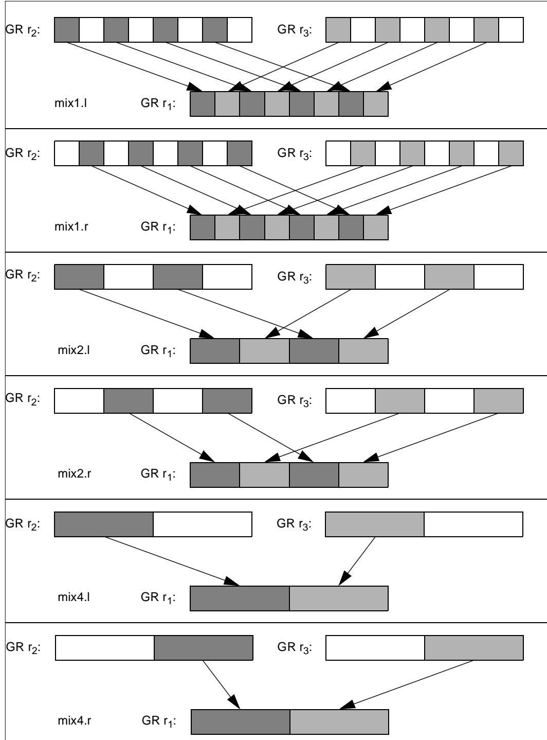
Figure 2-25. Mix Example
