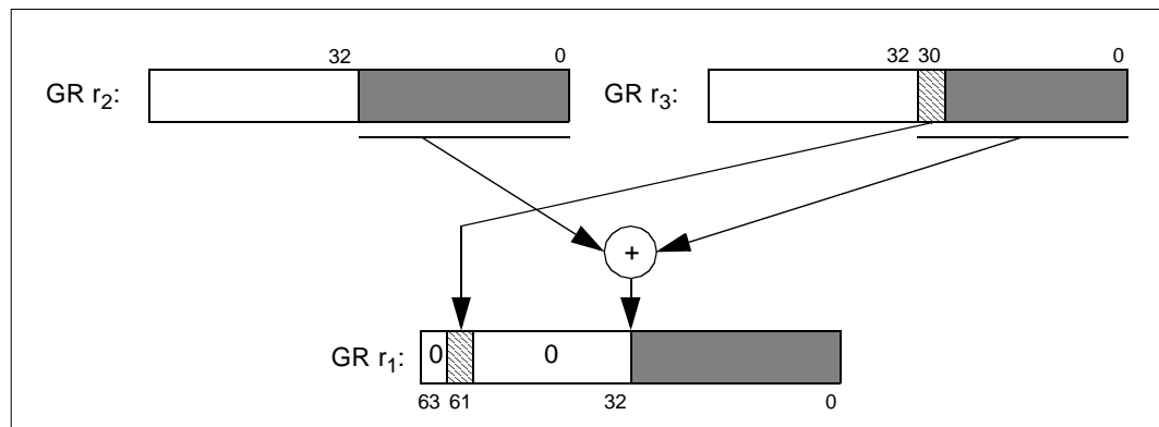
Figure 2-1. Add Pointer
