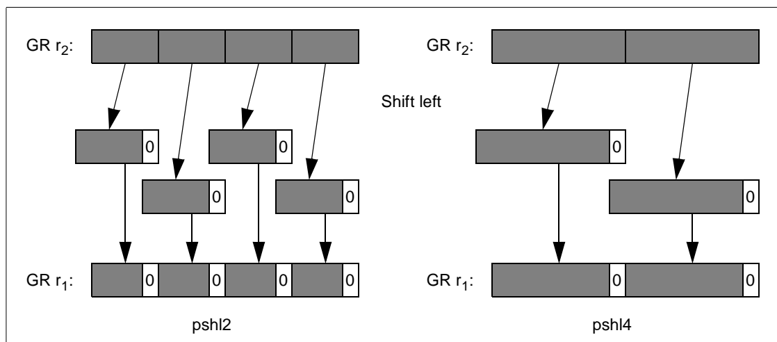
Figure 2-39. Parallel Shift Left Example
