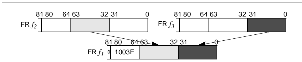
Figure 2-13. Floating-point Mix Left-Right
