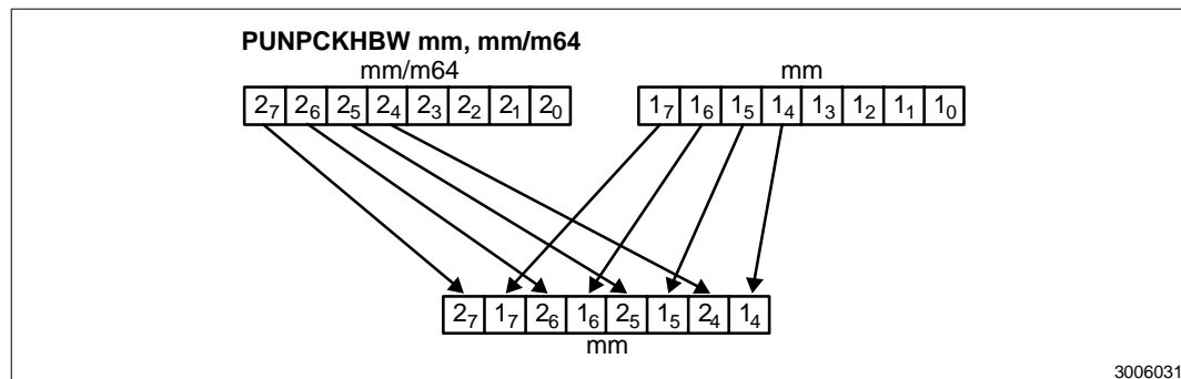
Figure 2-22. High-order Unpacking and Interleaving of Bytes with the PUNPCKHBW Instruction
