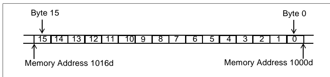
Figure 3-11. Four Packed FP Data in Memory (at address 1000H)
