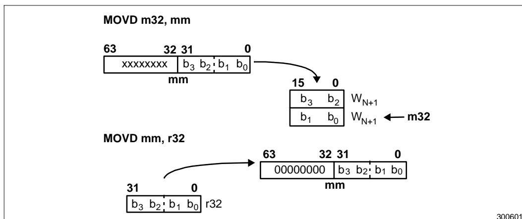
Figure 2-1. Operation of the MOVD Instruction
