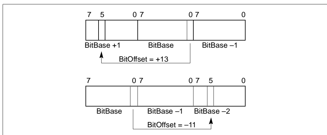
Figure 1-2. Memory Bit Indexing
