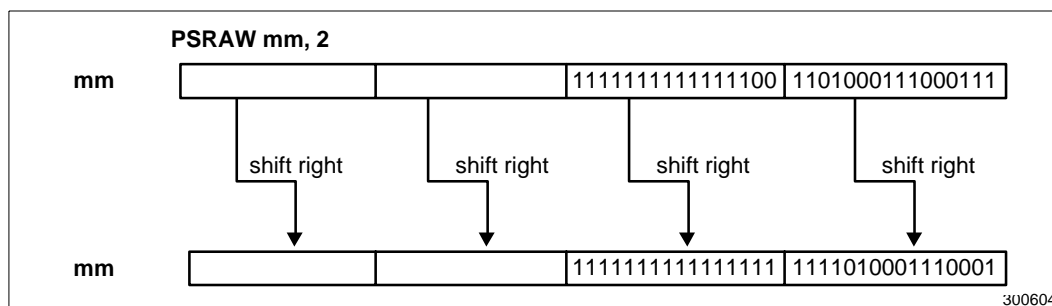
Figure 2-17. Operation of the PSRAW Instruction
