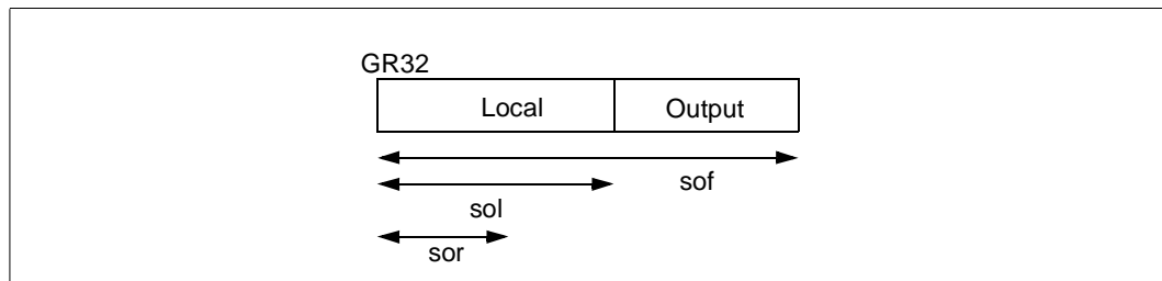
Figure 2-2. Stack Frame
