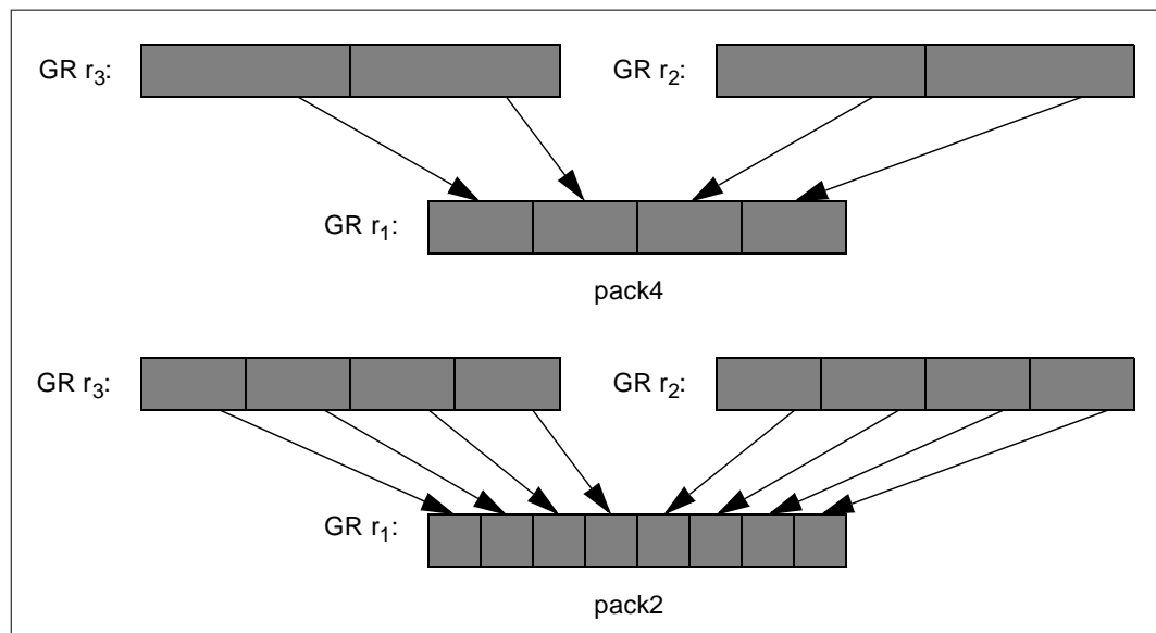
Figure 2-28. Pack Operation
