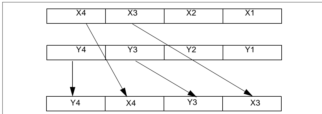
Figure 3-6. Unpack High Operation
