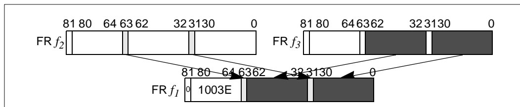
Figure 2-17. Floating-point Parallel Merge Sign and Exponent Operation
