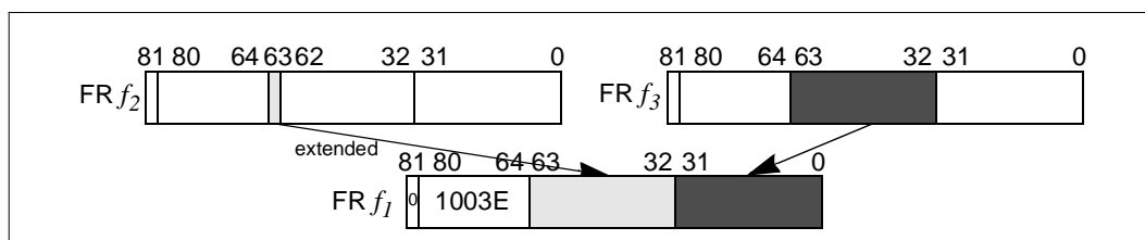
Figure 2-22. Floating-point Sign Extend Right
