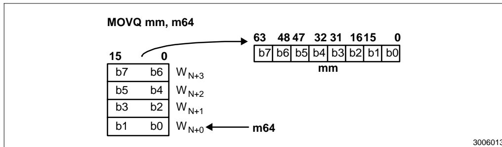
Figure 2-2. Operation of the MOVQ Instruction
