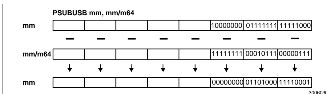
Figure 2-21. Operation of the PSUBUSB Instruction
