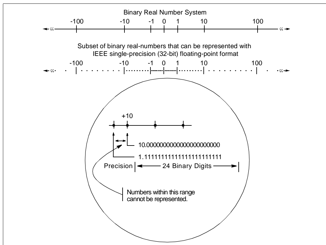
Figure 3-8. Binary Real Number System
