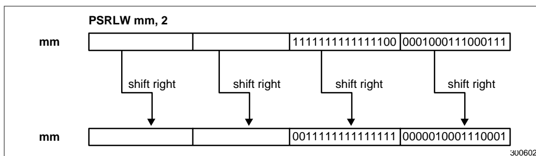
Figure 2-18. Operation of the PSRLW Instruction
