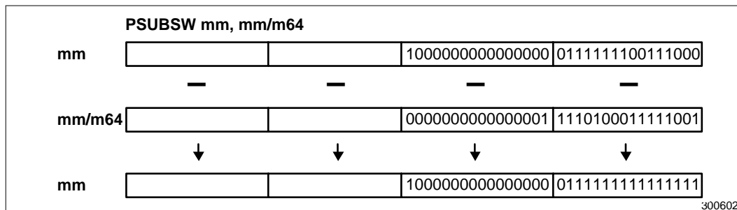
Figure 2-20. Operation of the PSUBSW Instruction
