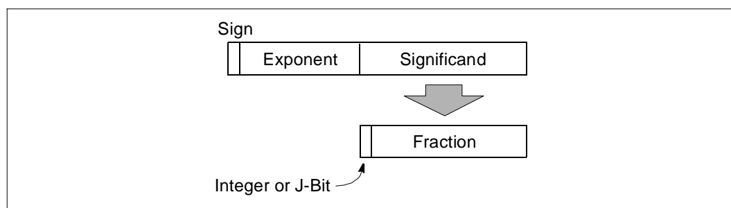
Figure 3-9. Binary Floating-point Format
