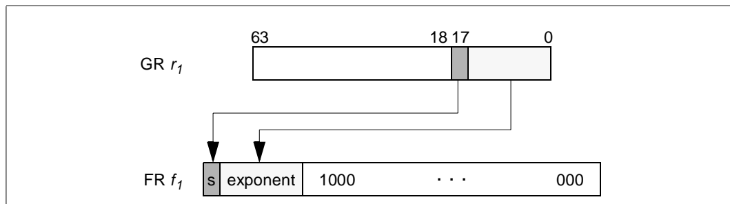
Figure 2-41. Function of setf.exp
