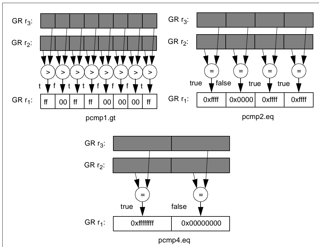
Figure 2-33. Parallel Compare Example
