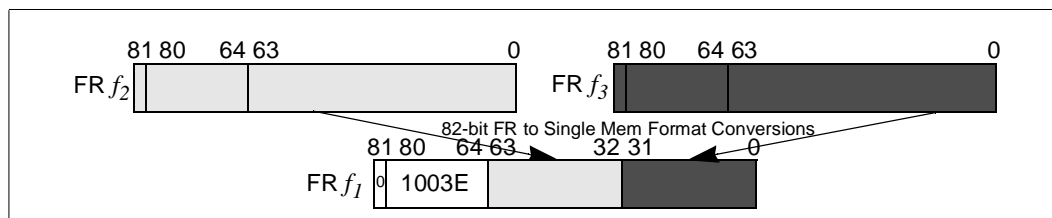
Figure 2-14. Floating-point Pack
