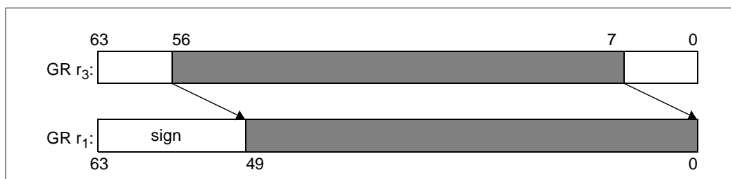
Figure 2-7. Extract Example
