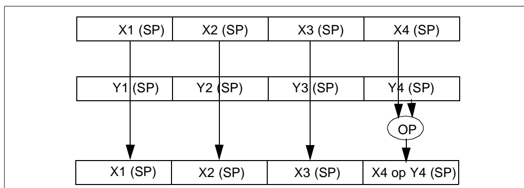
Figure 3-4. Scalar Operation
