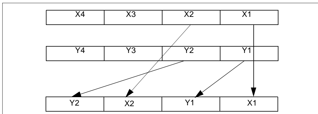
Figure 3-7. Unpack Low Operation
