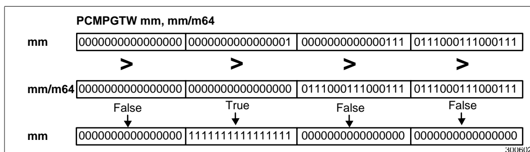
Figure 2-11. Operation of the PCMPGTW Instruction
