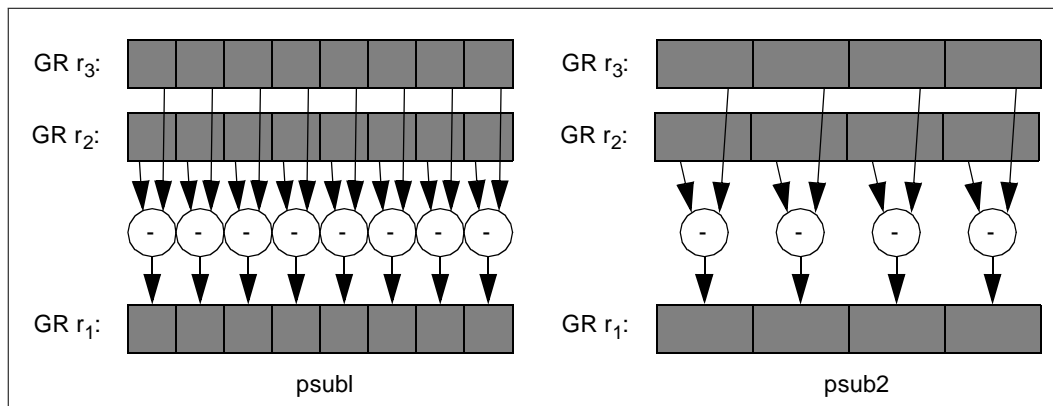
Figure 2-40. Parallel Subtract Example
