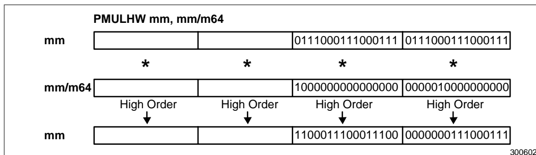
Figure 2-13. Operation of the PMULHW Instruction
