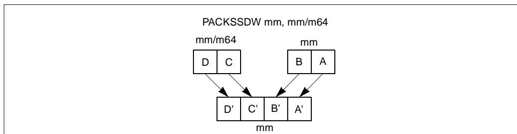
Figure 2-3. Operation of the PACKSSDW Instruction
