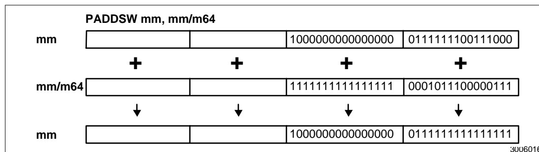
Figure 2-6. Operation of the PADDSW Instruction
