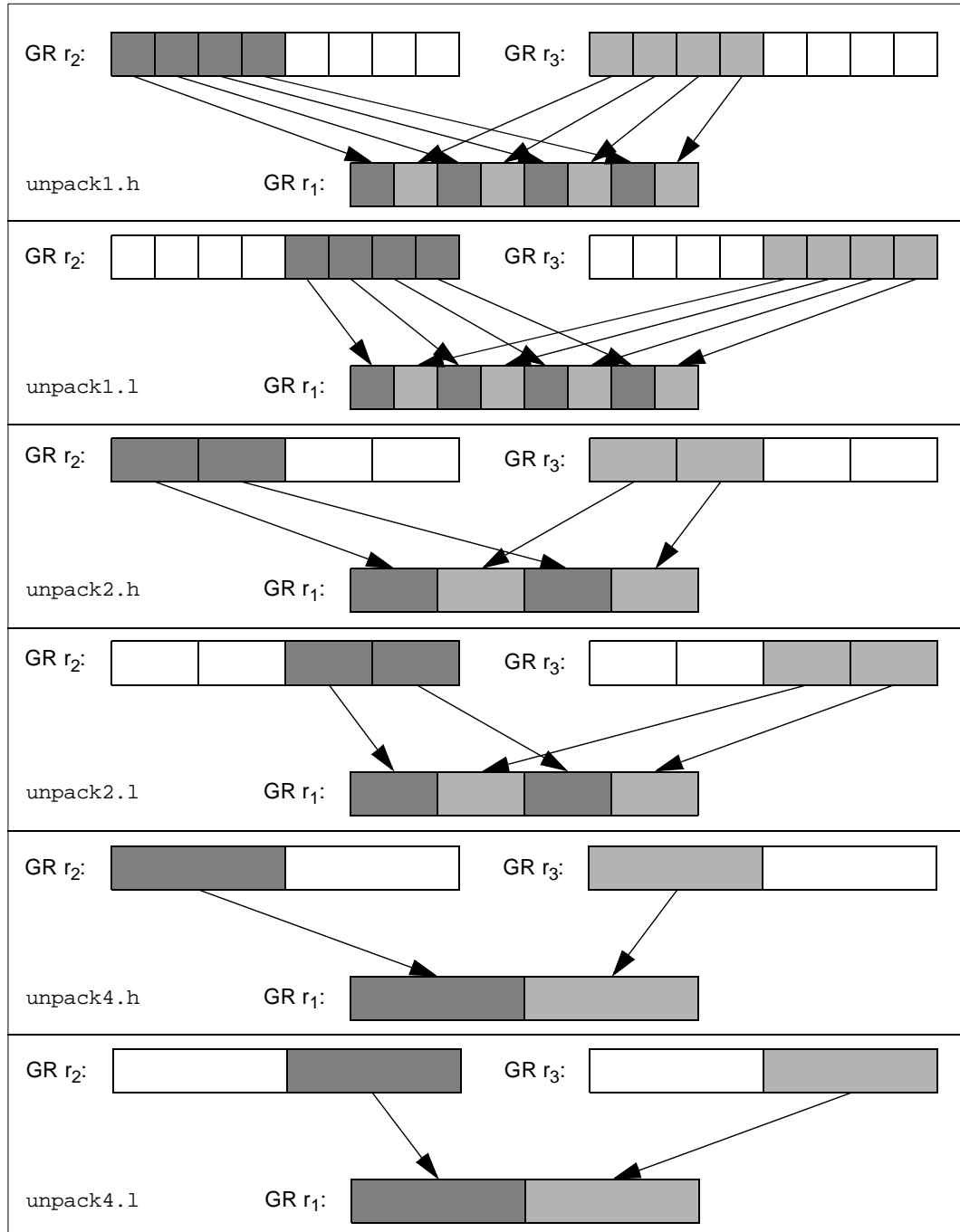
Figure 2-45. Unpack Operation
