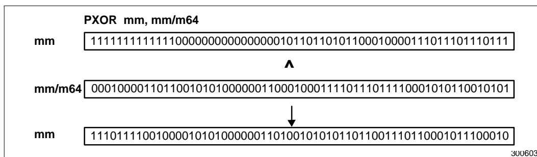
Figure 2-24. Operation of the PXOR Instruction
