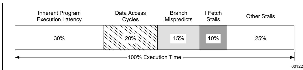
Figure 10-2. Itanium® Processor Family Cycle Accounting
