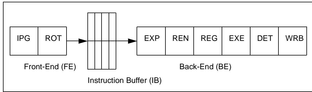
Figure A-1. Core Pipeline of the Itanium ® 2 Processor
