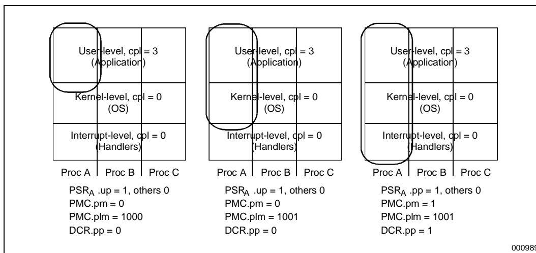
Figure 10-6. Single Process Monitor
