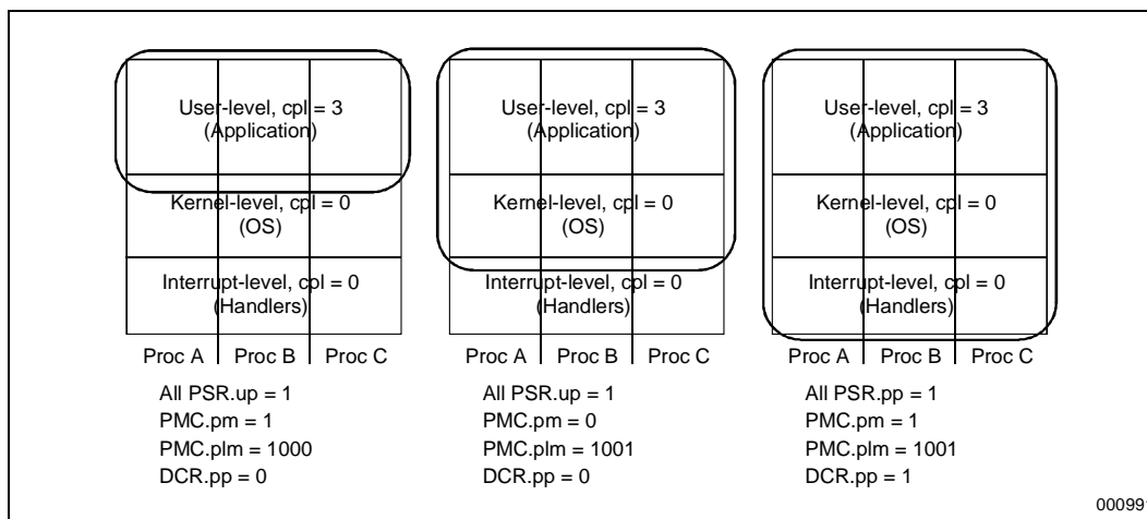
Figure 10-8. System Wide Monitor
