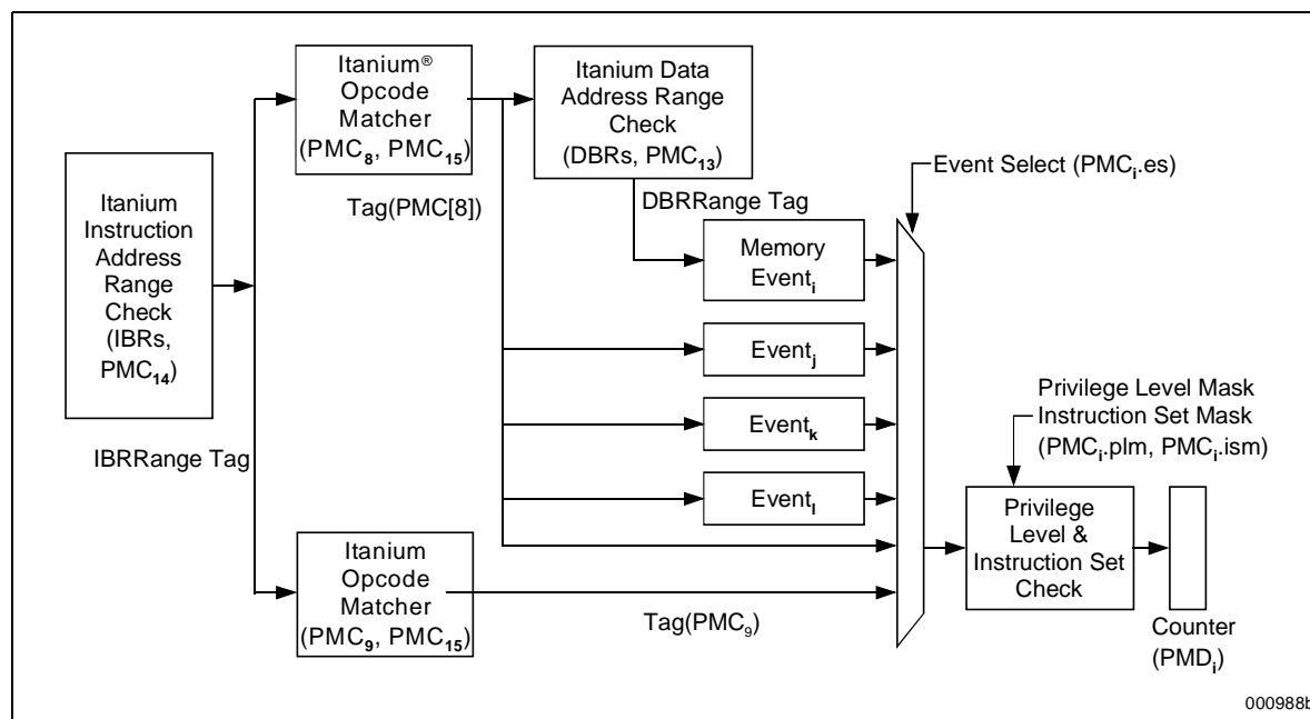
Figure 10-5. Instruction Tagging Mechanism in the Itanium® 2 Processor
