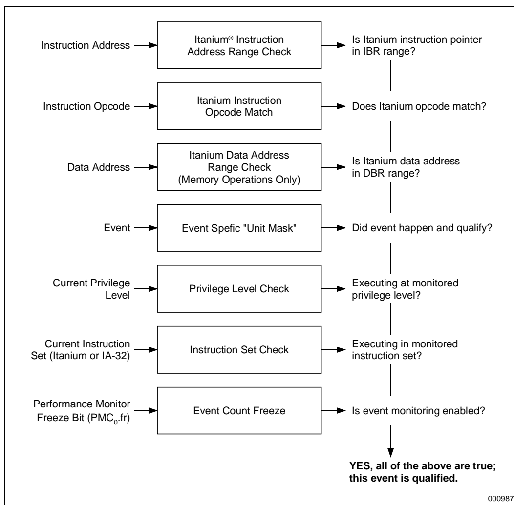
Figure 10-4. Itanium® 2 Processor Event Qualification
