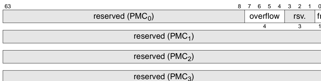
Figure 10-13. Itanium® 2 Processor Performance Monitor Overflow Status Registers (PMC 0,1,2,3 )
