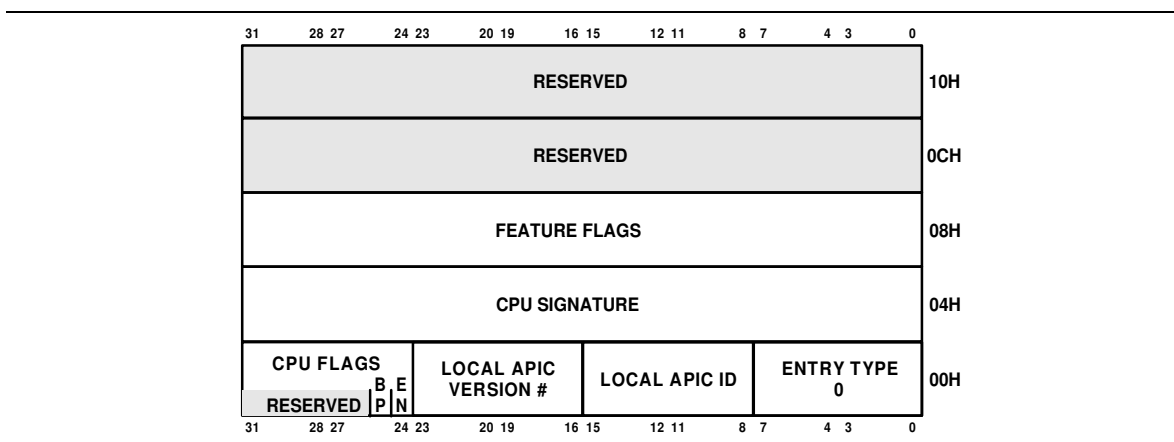
Figure 4-4. Processor Entry
