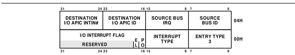
Figure 4-7. I/O Interrupt Entry
