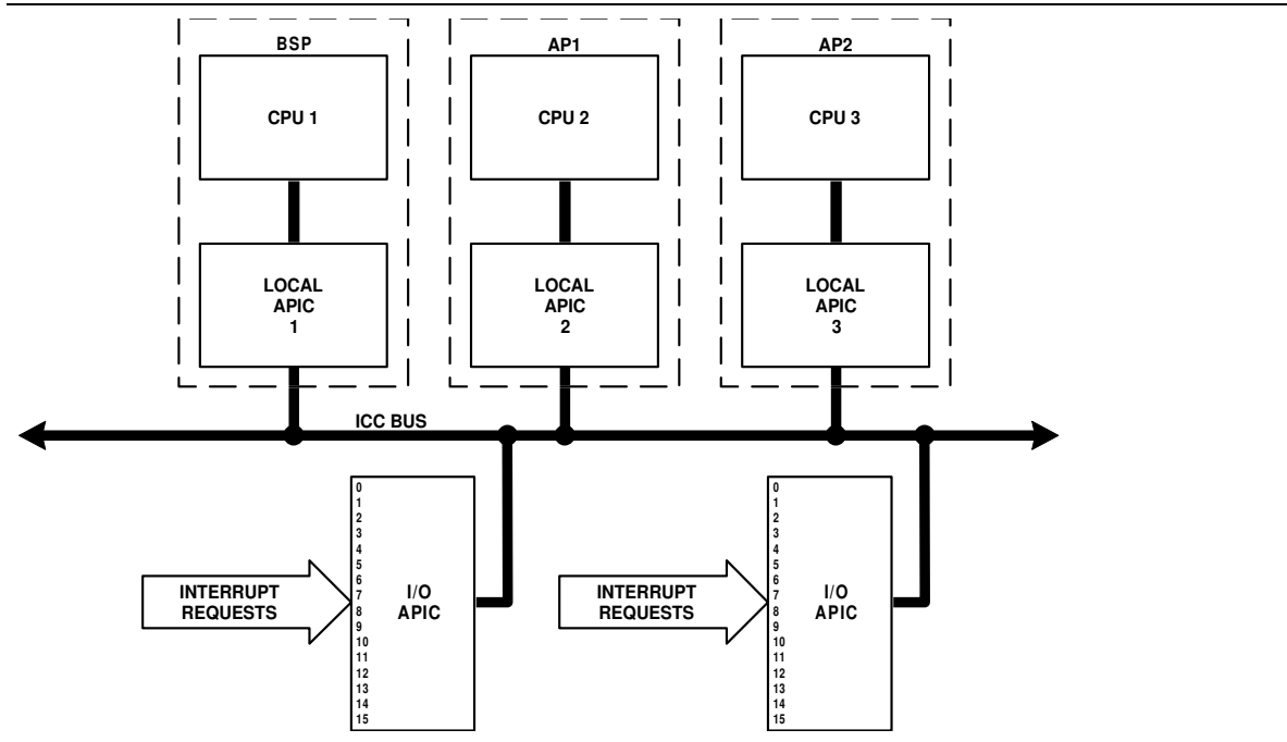
Figure 2-2. APIC Configuration
