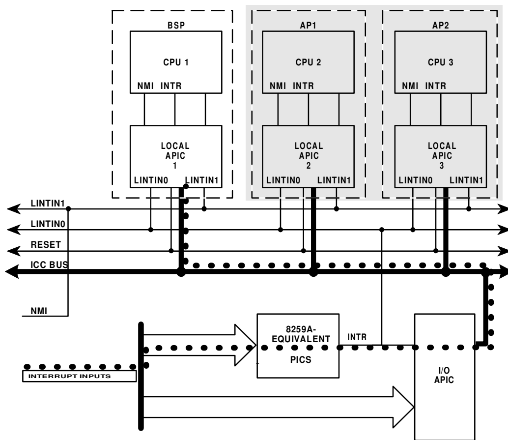
Figure 3-4. Virtual-wire Mode via I/O APIC
