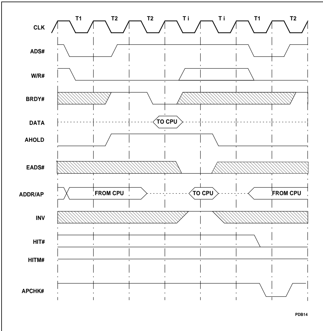
Figure 6-22. Inquire Cycle that Invalidates Non-M-State Line
