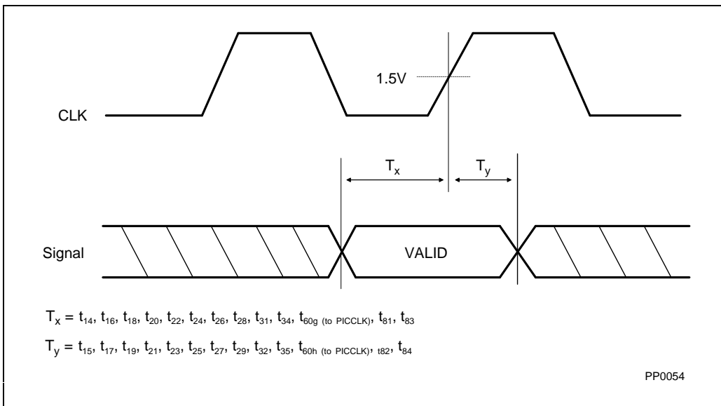
Figure 23-4. Setup and Hold Timings
