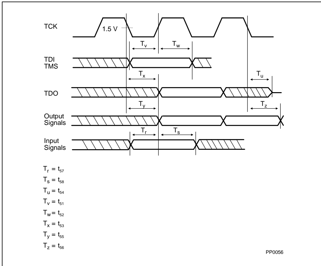
Figure 23-6. Test Timings
