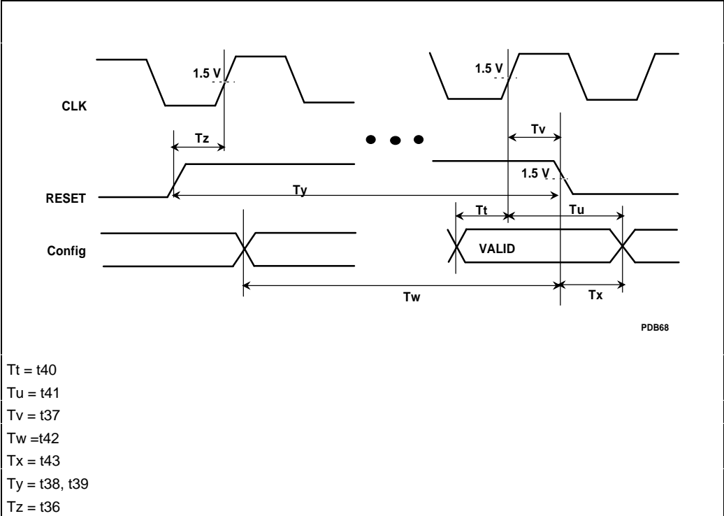
Figure 7-5. Reset and Configuration Timings
