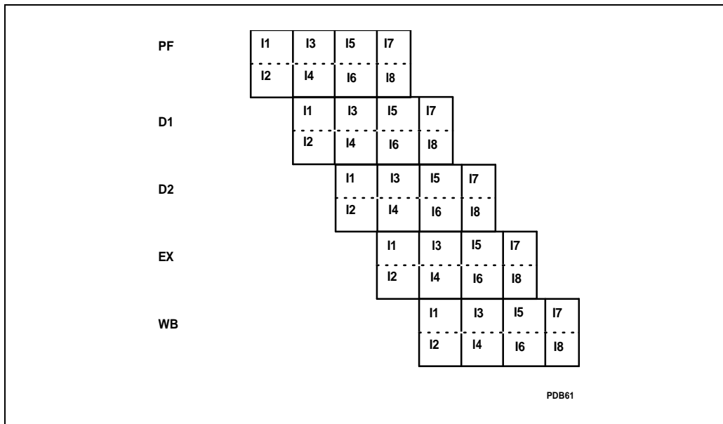
Figure 3-2. Pentium® Processor Pipe-line Execution
