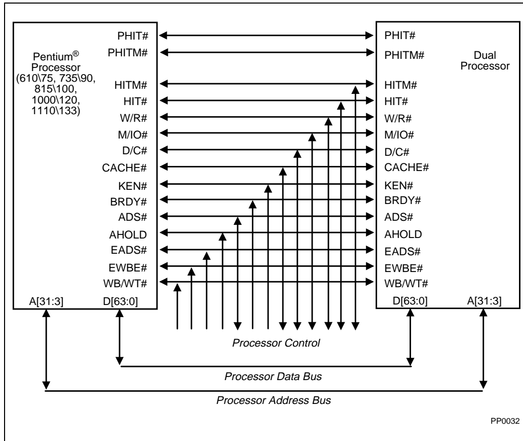
Figure 20-5. Cache Consistency Interface
