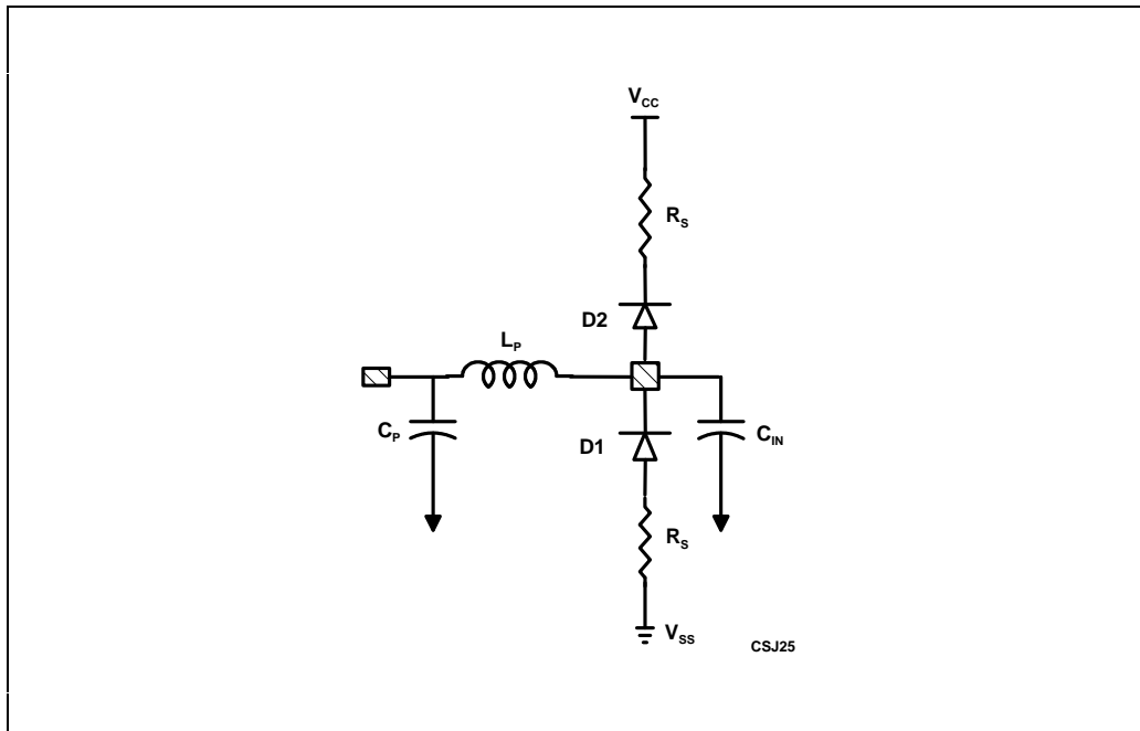
Figure 8-4. Complete Input Model Including Diode
