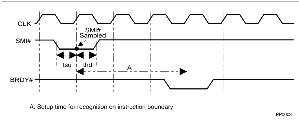
Figure 14-3. SMI# Timing
