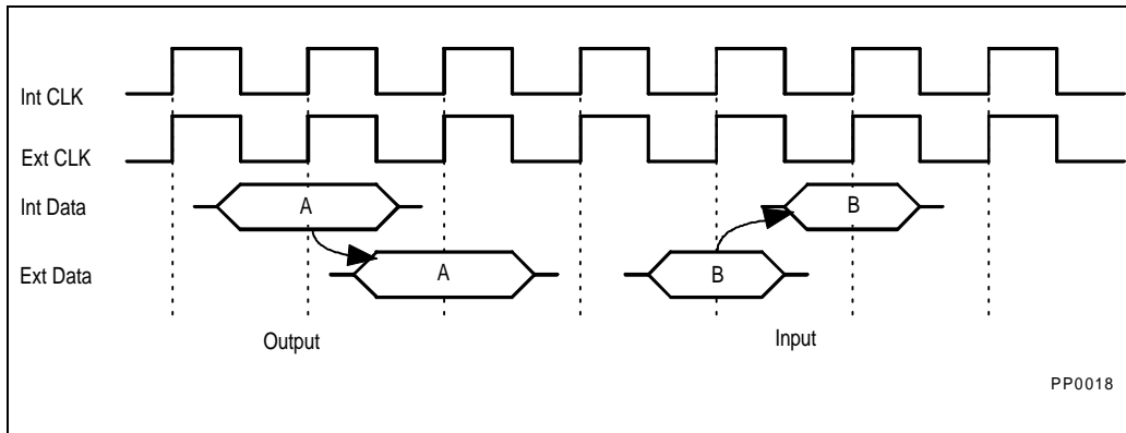
Figure 19-1. Pentium® Processor (510\60, 567\66) Synchronous Internal/External Data Movement
