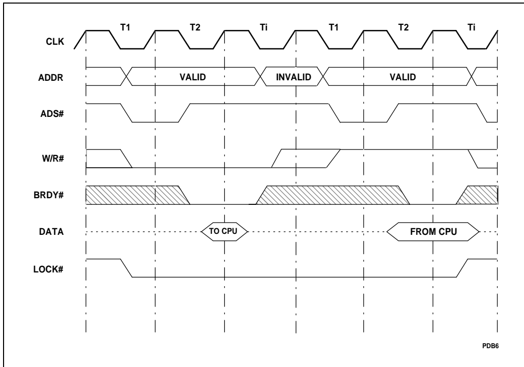
Figure 6-11. LOCK# Timing
