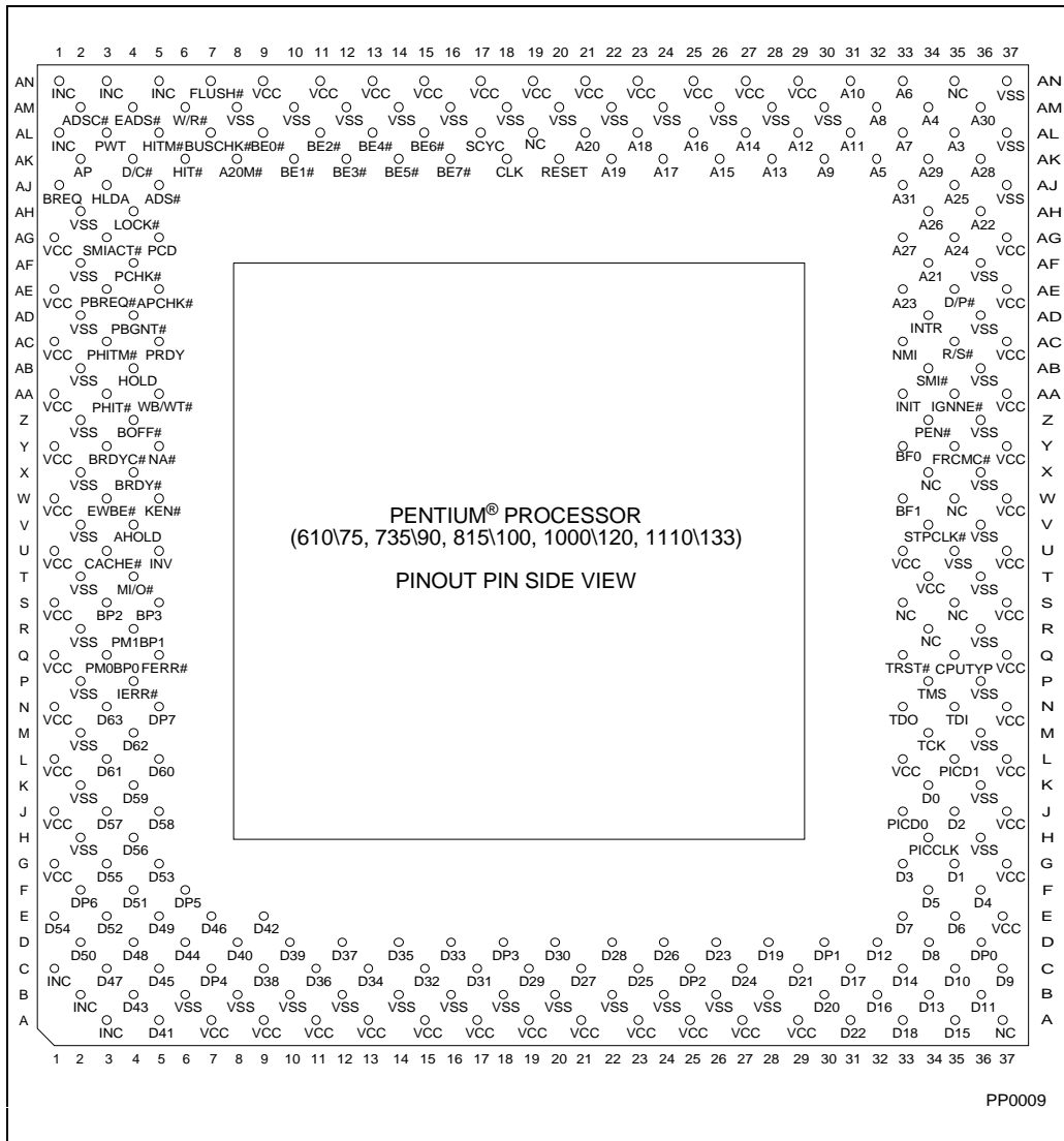
Figure 17-2. Pentium® Processor (610\75, 735\90, 815\100, 1000\120, 1110\133) Pinout — Pin Side View
