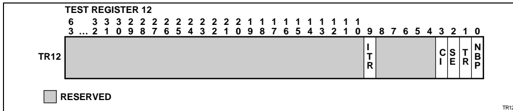
Figure 33-4. Test Register TR12
