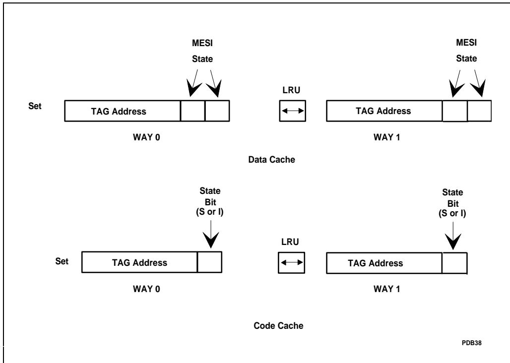
Figure 3-3. Conceptual Organization of Code and Data Caches
