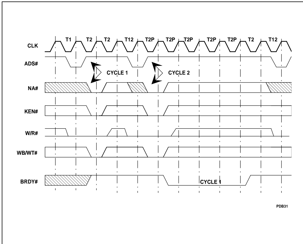
Figure 6-19. KEN# and WB/WT# Sampling with NA#
