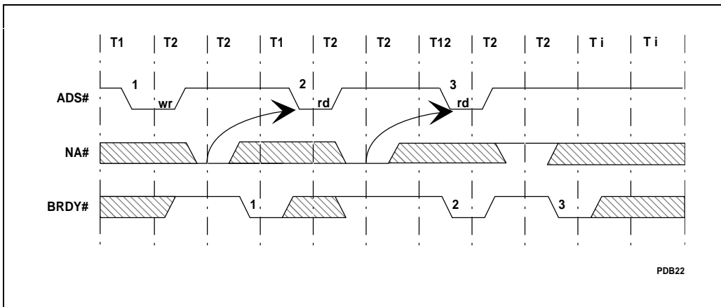
Figure 6-30. Bus Cycles Without Dead Clock
