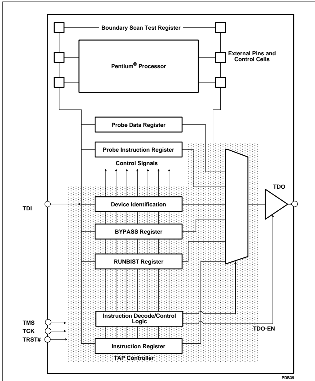
Figure 11-1. Test Access Port Block Diagram
