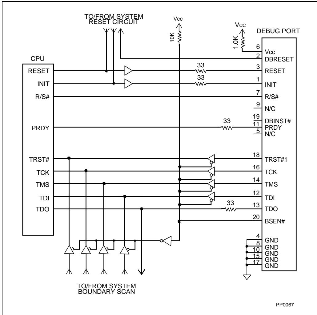
Figure 31-3. Single CPU — Boundary Scan Used
