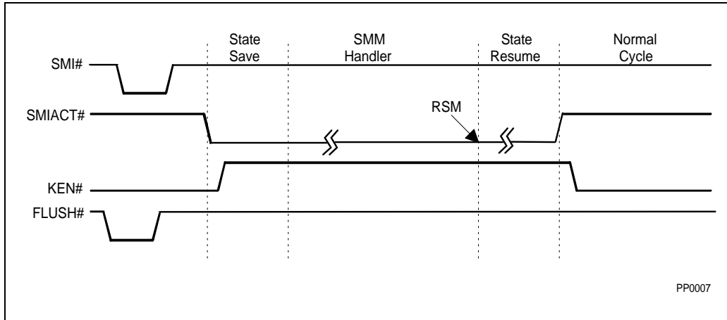
Figure 14-7. Flush with Non-Cached SMM with Overlay
