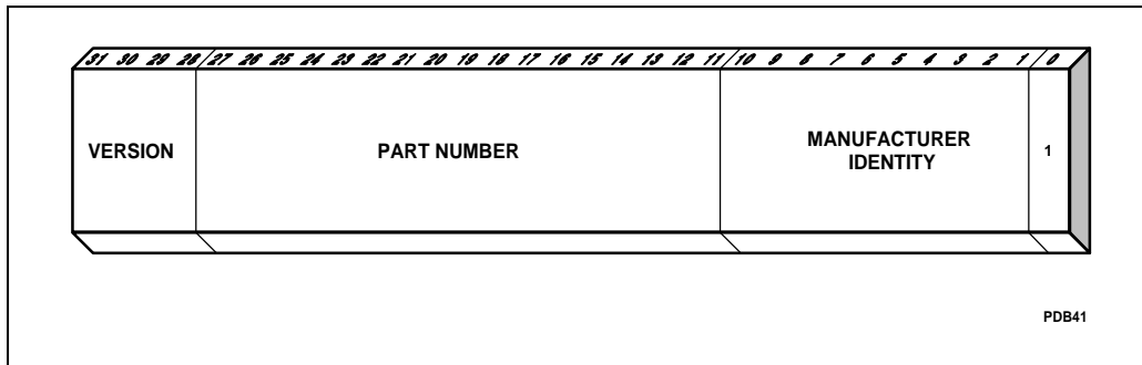
Figure 11-3. Format of the Device ID Register
