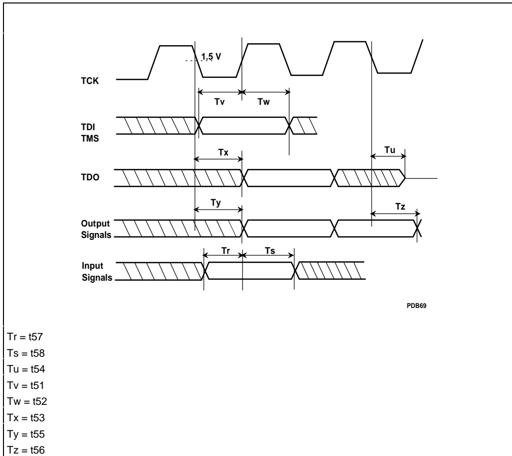
Figure 7-6. Test Timings
