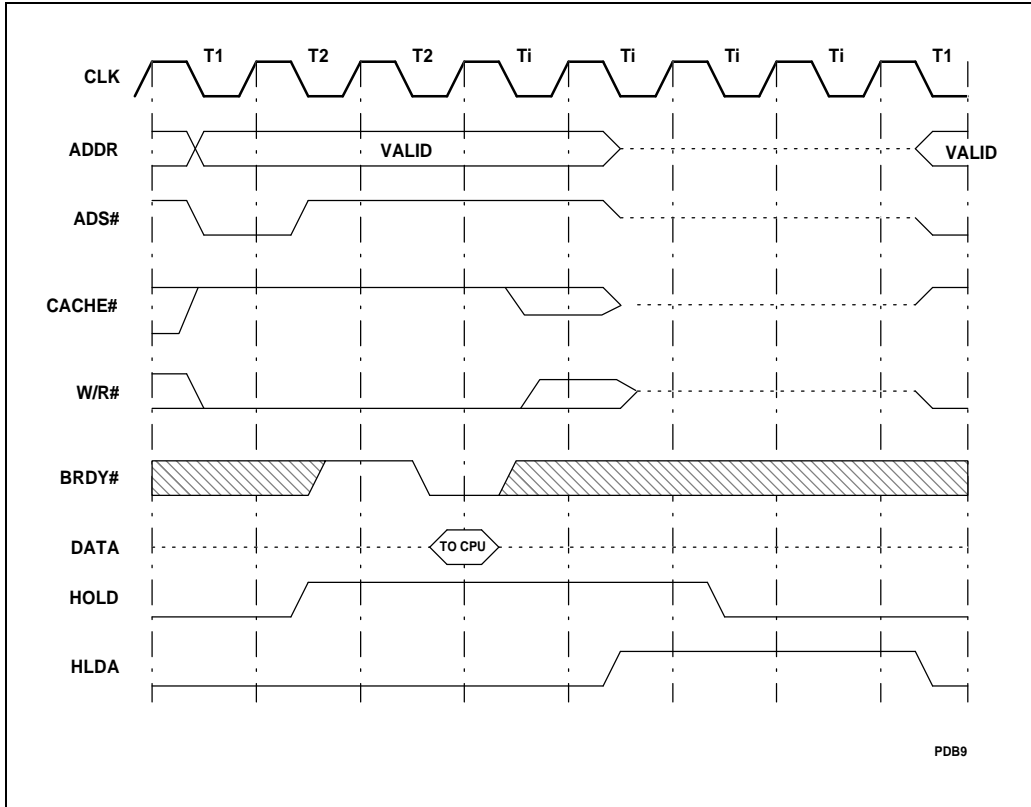
Figure 6-15. HOLD/HLDA Cycles
