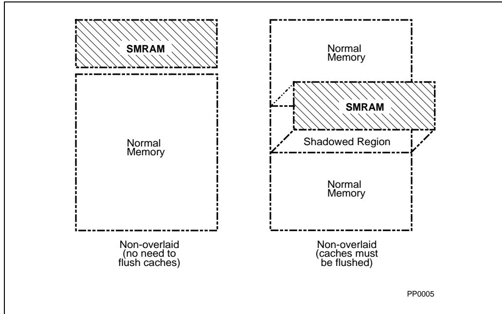
Figure 14-5. SMRAM Location
