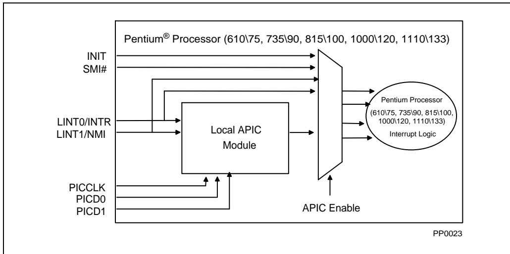
Figure 19-6. Local APIC Interface
