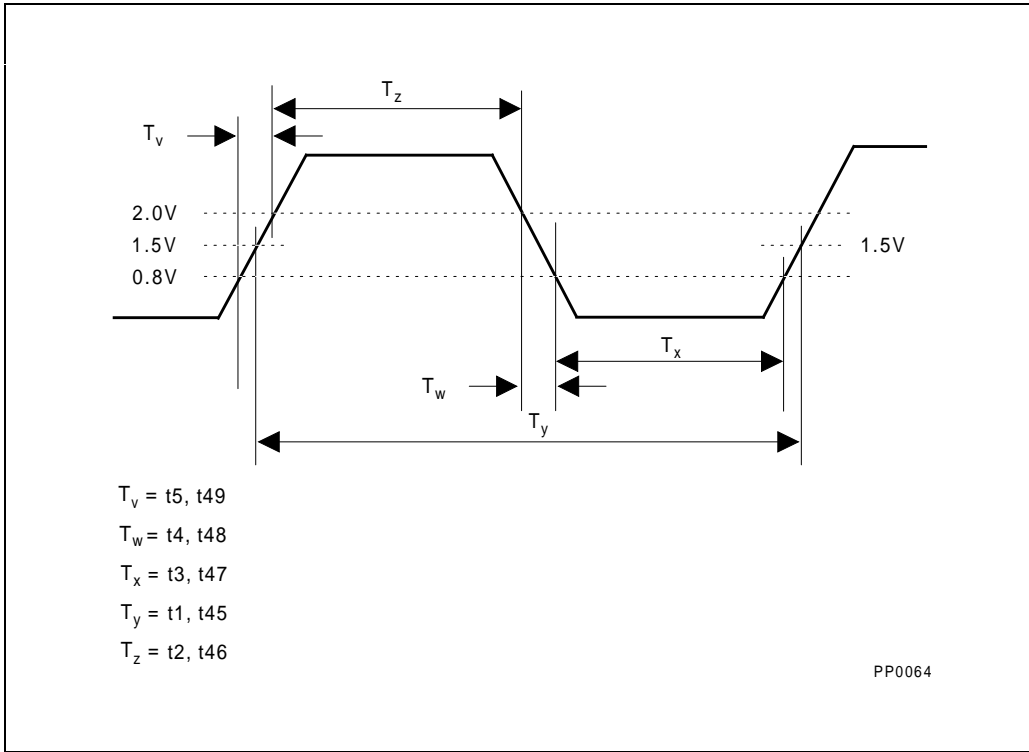
Figure 7-1. Clock Waveform
