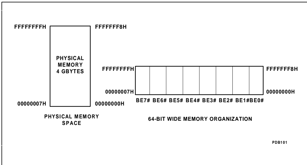
Figure 6-1. Memory Organization
