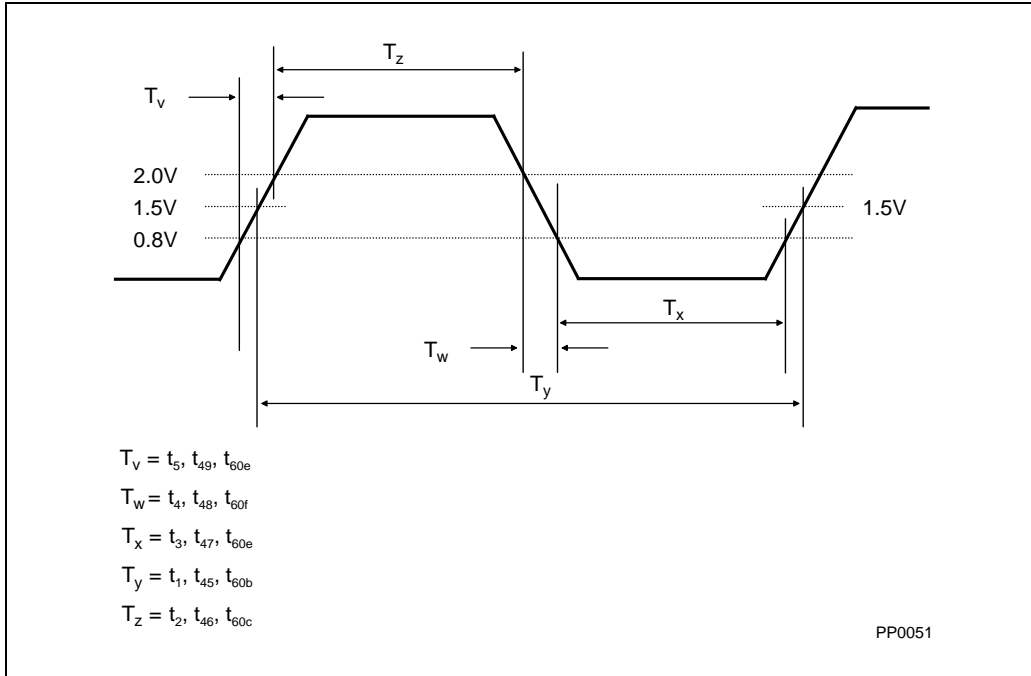
Figure 23-1. Clock Waveform
