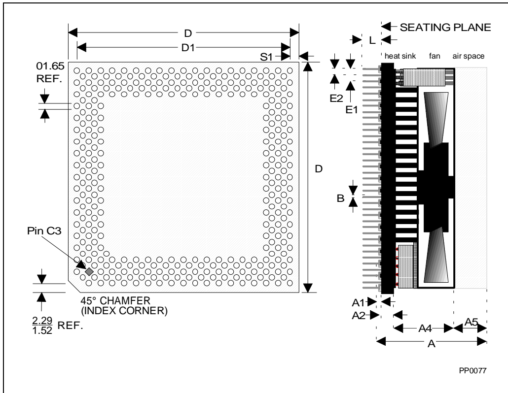
Figure 32-3. Future OverDrive® Processor Package Dimensions
