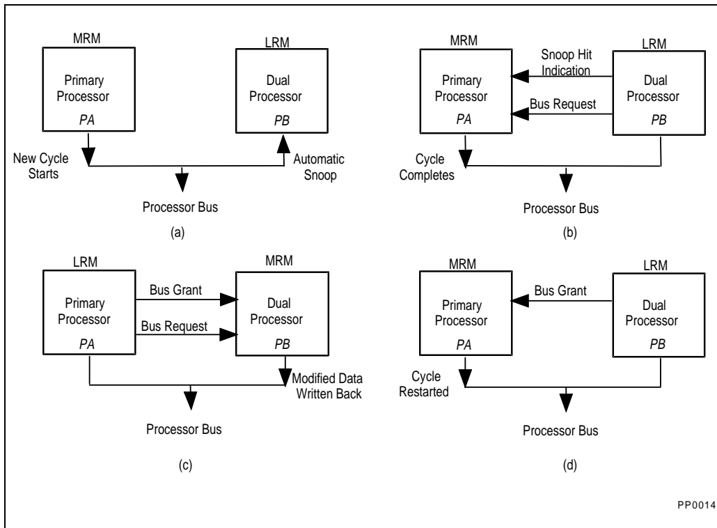
Figure 18-3. Dual Processor L1 Cache Consistency
