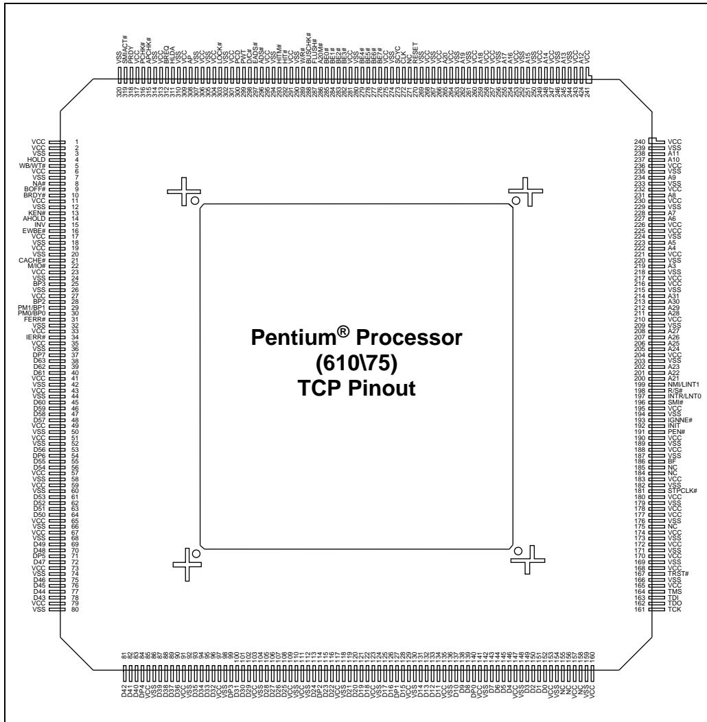
Figure 34-1. Pentium® Processor (610\75) TCP Pinout
