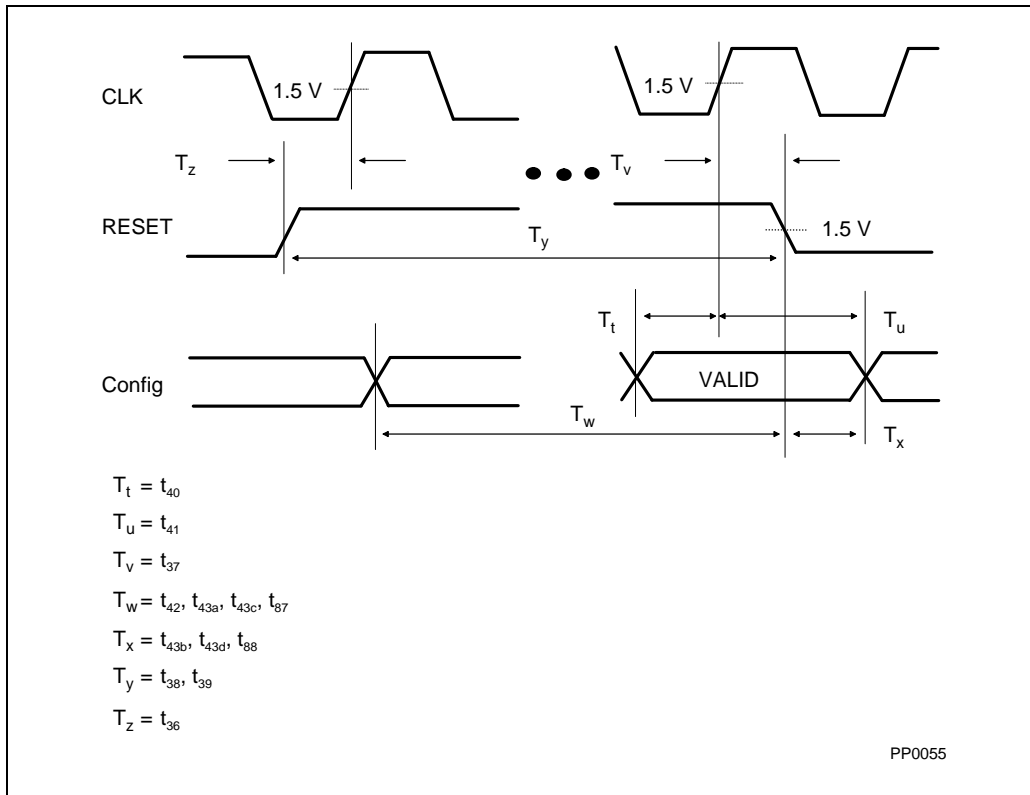
Figure 23-5. Reset and Configuration Timings
