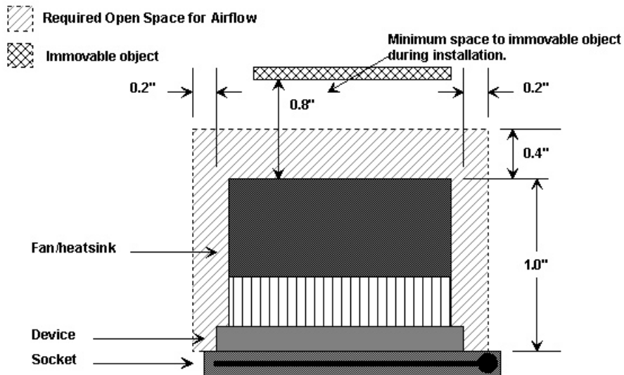
Figure 16-10. IVP Criteria — Space Requirements
