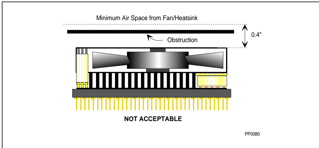
Figure 32-6. Fan/Heatsink Unacceptable Airflow Blockage
