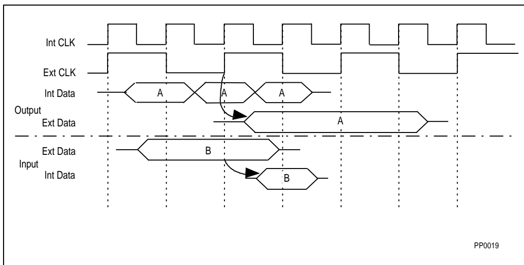
Figure 19-2. Pentium® Processor (610\75, 735\90, 815\100, 1000\120, 1110\133) 1/2 Bus Internal/External Data Movement
