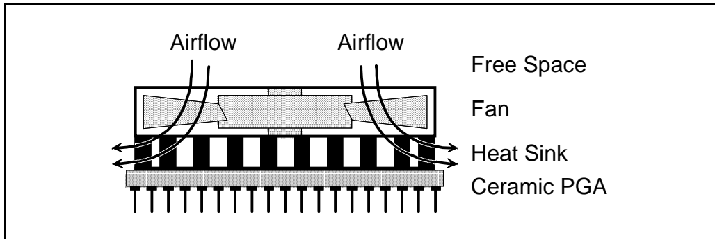
Figure 16-8. Fan/Heatsink Example
