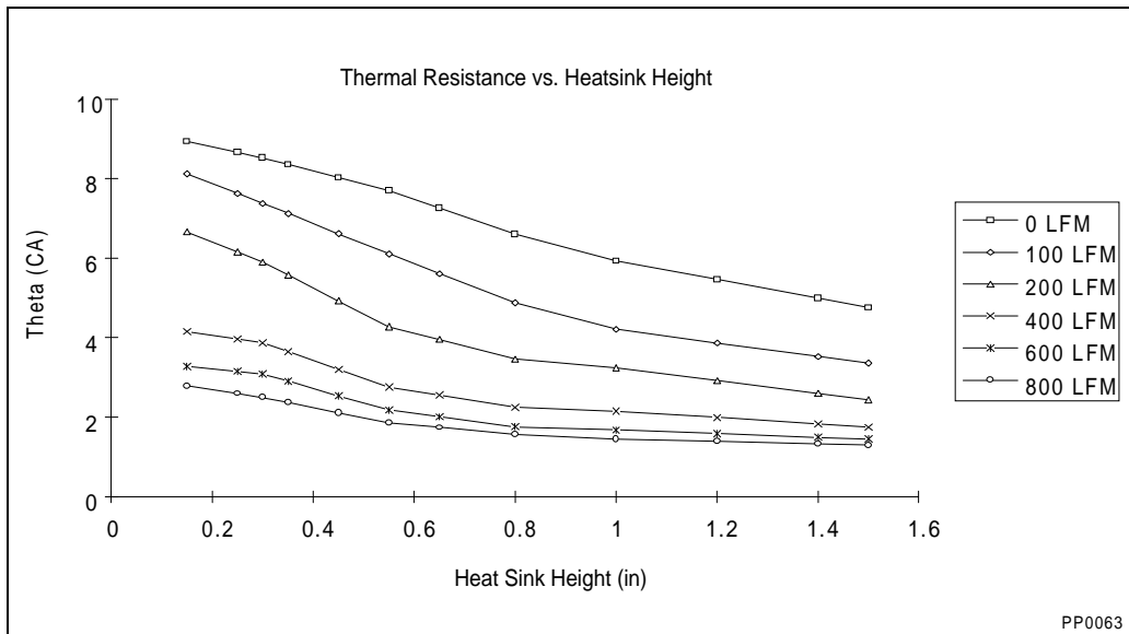
Figure 26-2. Thermal Resistance vs. Heat Sink Height
