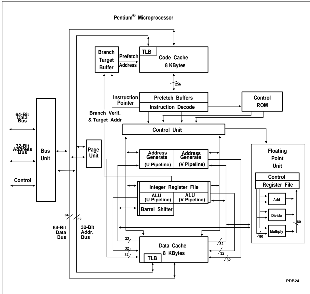
Figure 2-1. Pentium® Processor Block Diagram
