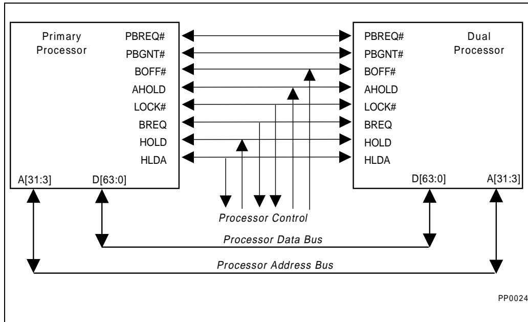
Figure 20-2. Dual Processor Arbitration Interface
