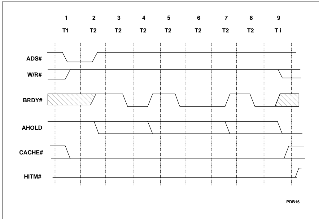
Figure 6-24. AHOLD Restriction during Write Cycles
