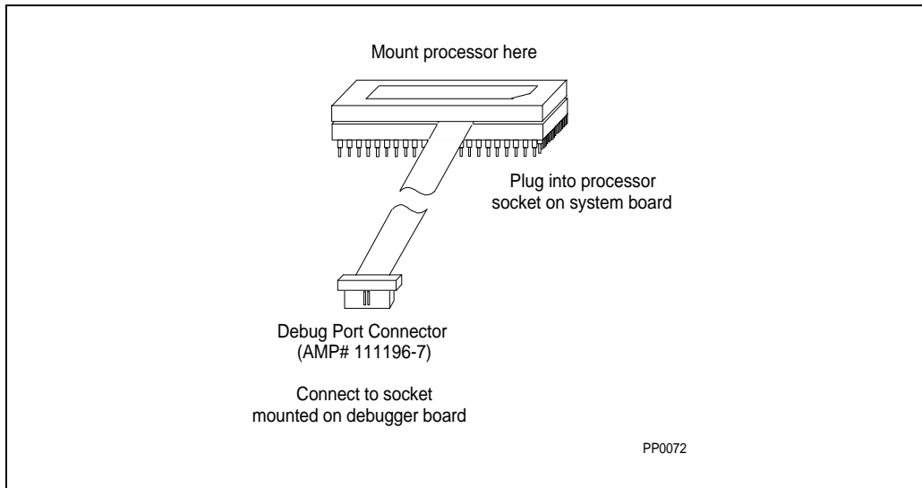
Figure 31-8. Uni-Processor Debug
