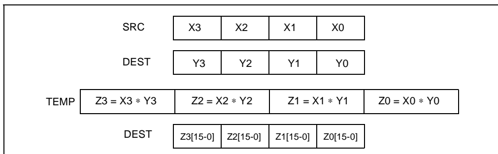
Figure 3-8. PMULLW Instruction Operation Using 64-bit Operands
