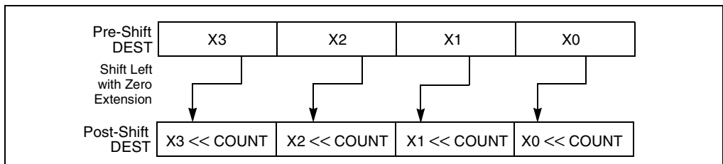
Figure 3-11. PSLLW, PSLLD, and PSLLQ Instruction Operation Using 64-bit Operand
