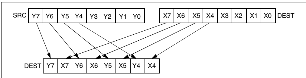
Figure 3-14. PUNPCKHBW Instruction Operation Using 64-bit Operands
