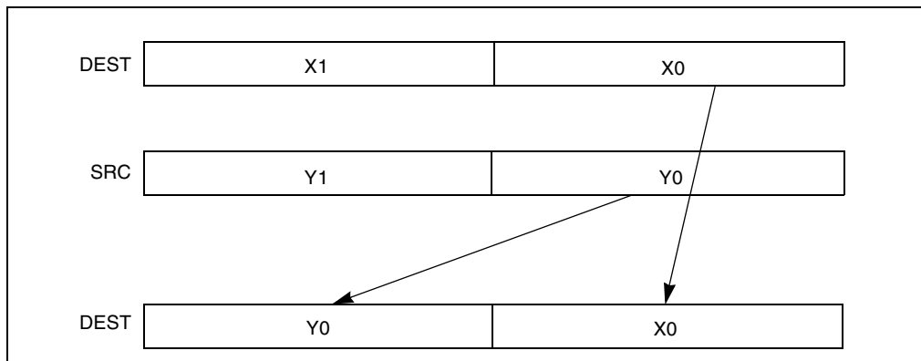
Figure 3-21. UNPCKLPD Instruction Low Unpack and Interleave Operation
