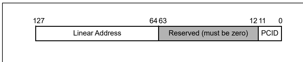
Figure 3-25. INVPCID Descriptor
