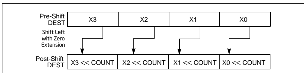
Figure 4-13. PSLLW, PSLLD, and PSLLQ Instruction Operation Using 64-bit Operand
