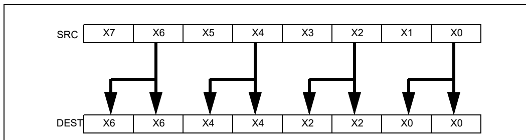
Figure 4-4. MOVSLDUP Operation
