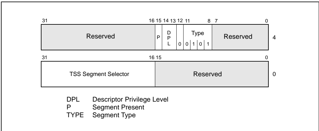
Figure 7-6. Task-Gate Descriptor
