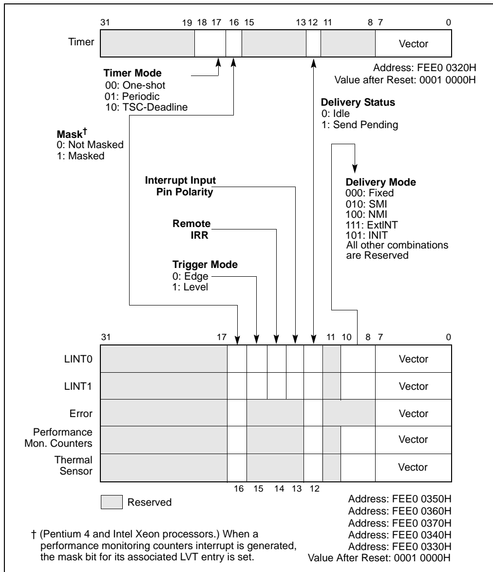
Figure 10-8. Local Vector Table (LVT)
