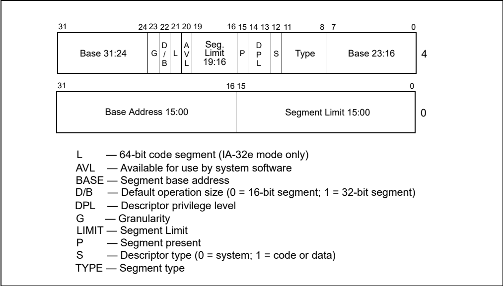
Figure 3-8. Segment Descriptor
