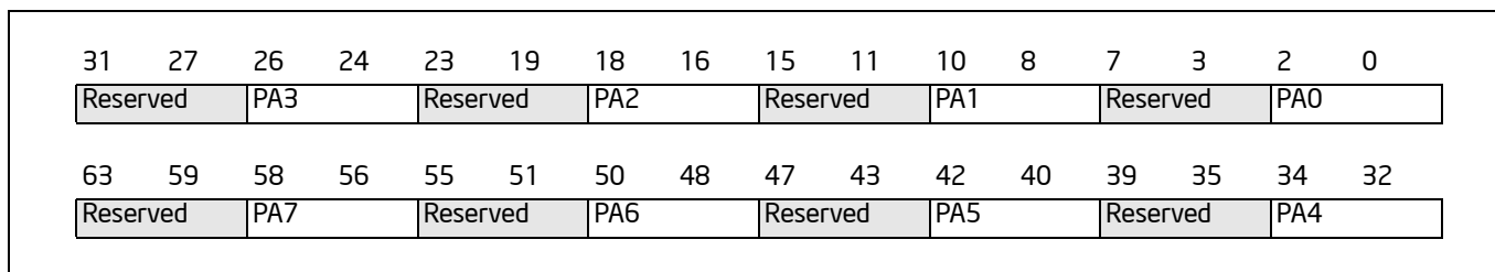
Figure 11-9. IA32_PAT MSR
