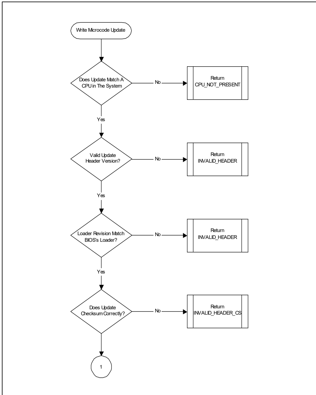
Figure 11-8. Microcode Update Write Operation Flow [1]
