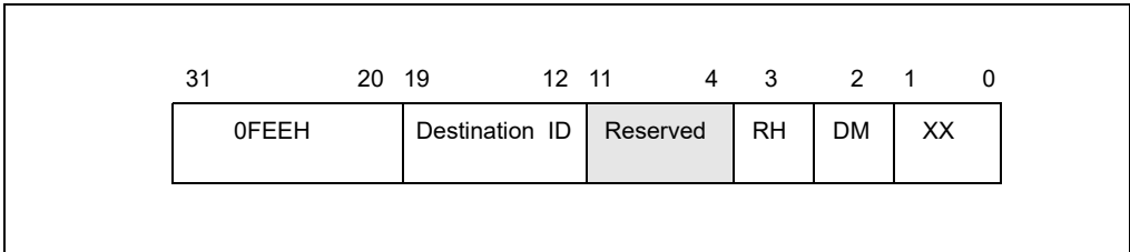
Figure 12-24. Layout of the MSI Message Address Register
