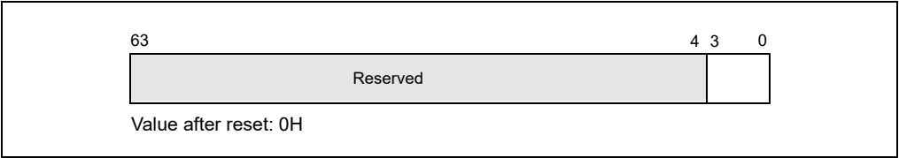
Figure 12-22. CR8 Register
