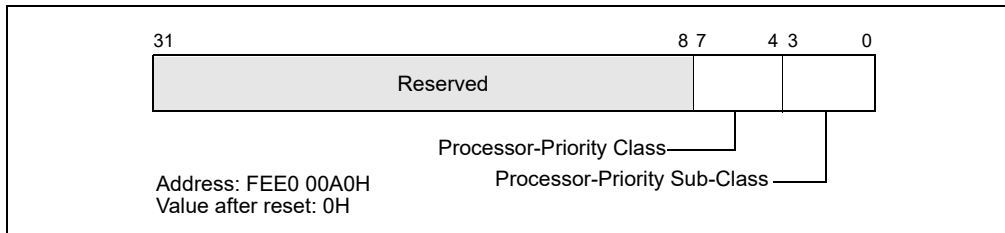
Figure 12-19. Processor-Priority Register (PPR)
