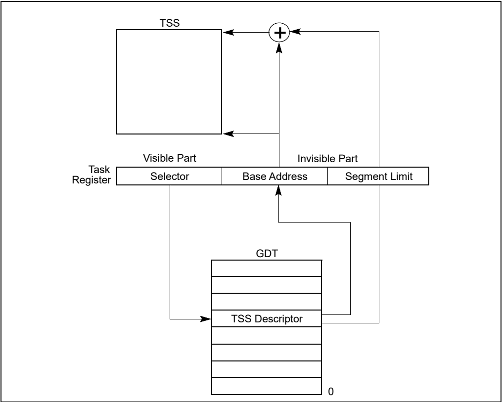
Figure 9-5. Task Register
