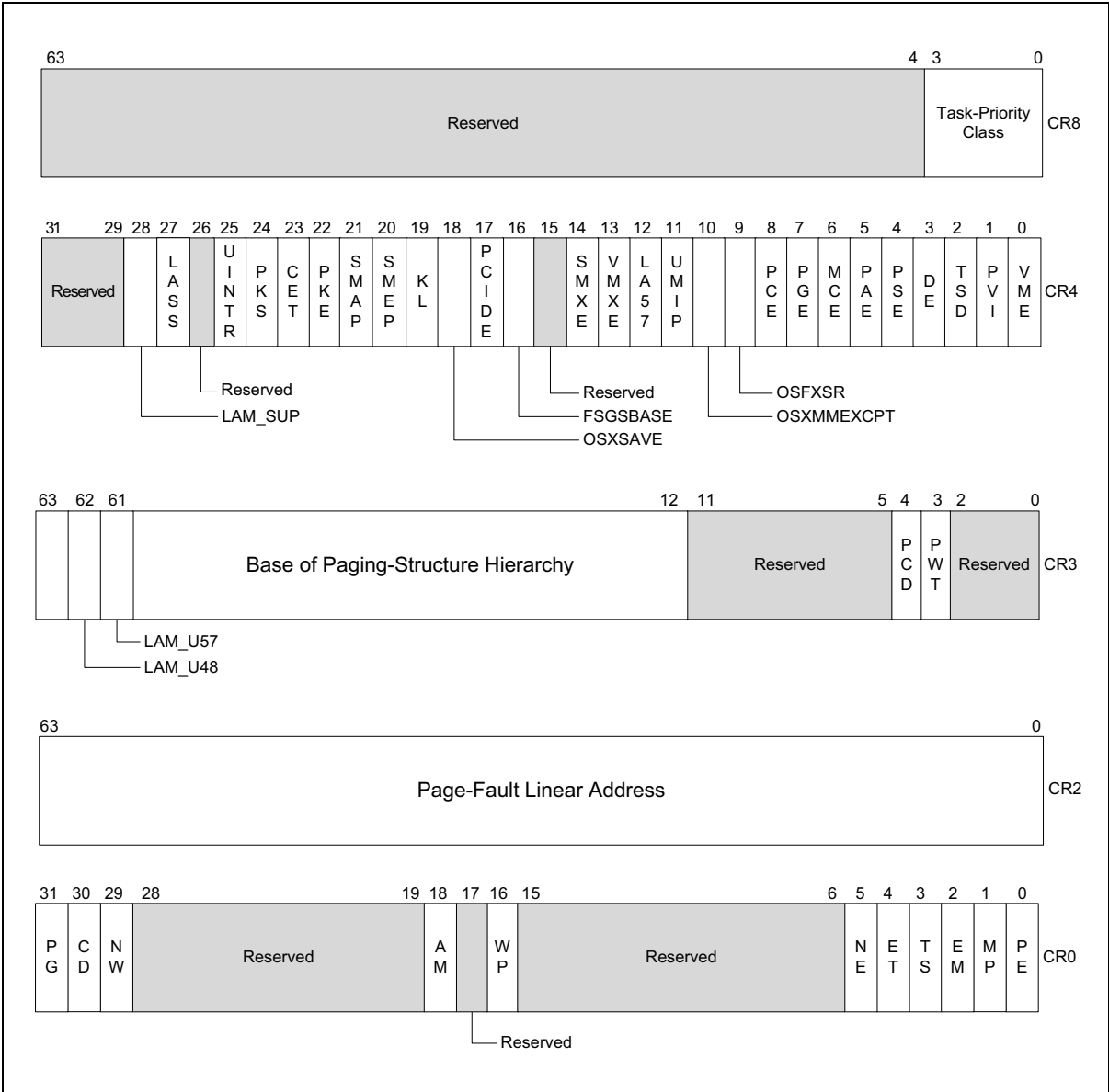
Figure 2-7. Control Registers
