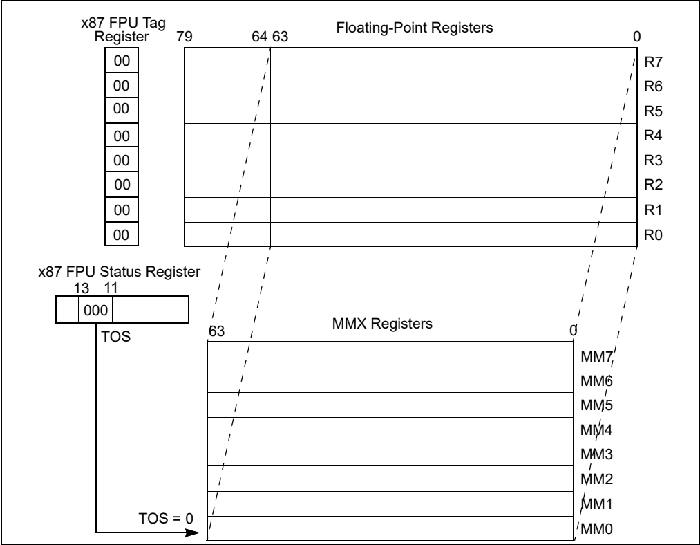
Figure 14-1. Mapping of MMX Registers to Floating-Point Registers
