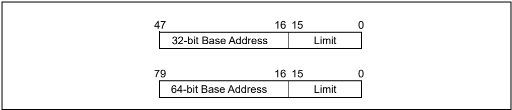
Figure 3-11. Pseudo-Descrptor Formats
