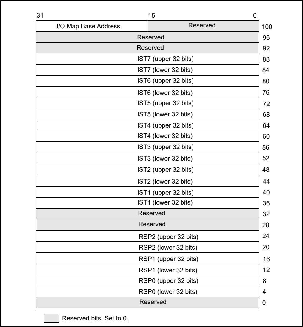
Figure 9-11. 64-Bit TSS Format
