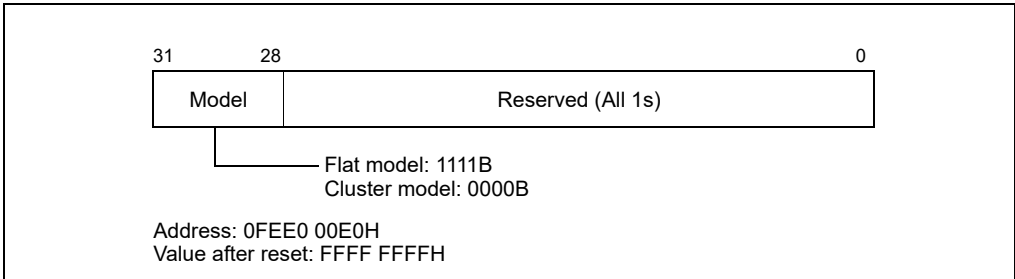
Figure 12-14. Destination Format Register (DFR)
