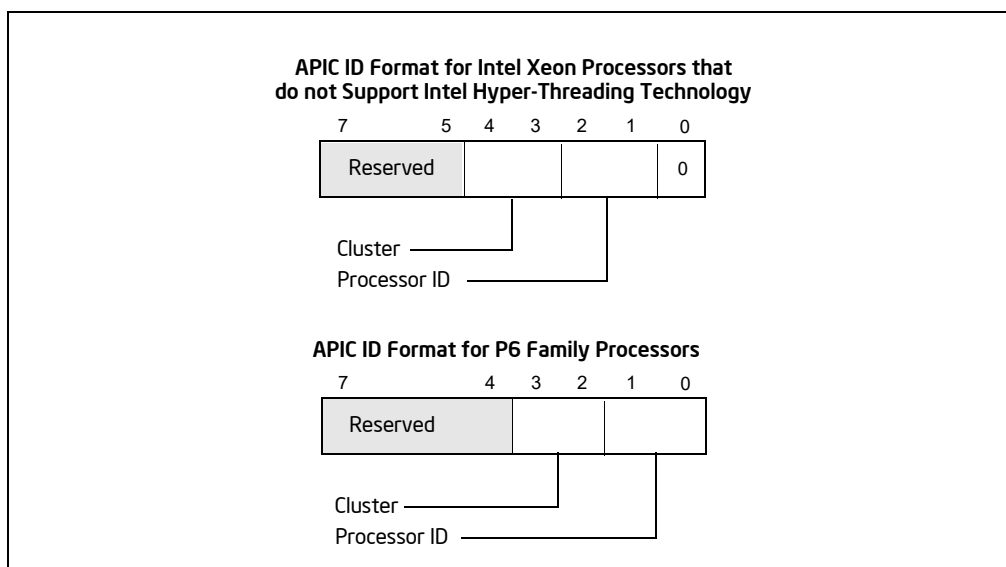
Figure 10-2. Interpretation of APIC ID in Early MP Systems
