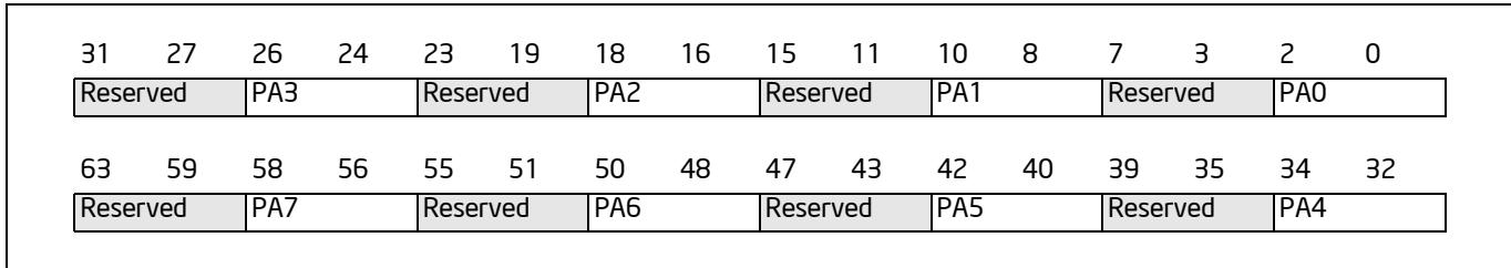
Figure 13-9. IA32_PAT MSR
