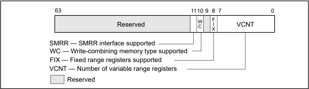
Figure 13-5. IA32_MTRRCAP Register
