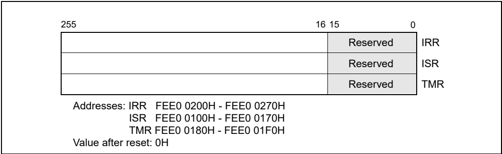
Figure 12-20. IRR, ISR, and TMR Registers
