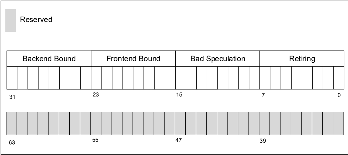
Figure 21-39. MSR_PERF_METRICS Definition
