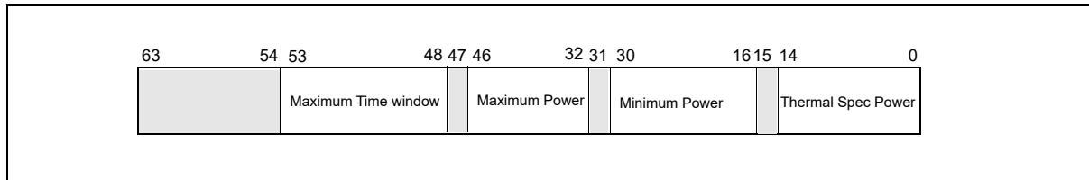
Figure 16-46. MSR_DRAM_POWER_INFO Register
