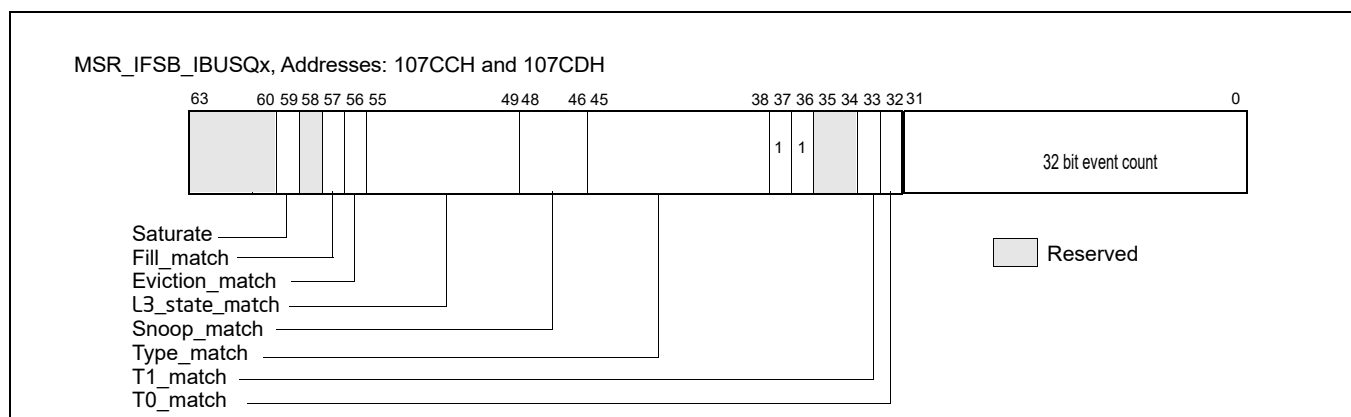
Figure 21-56. MSR_IFSB_IBUSQx, Addresses: 107CCH and 107CDH
