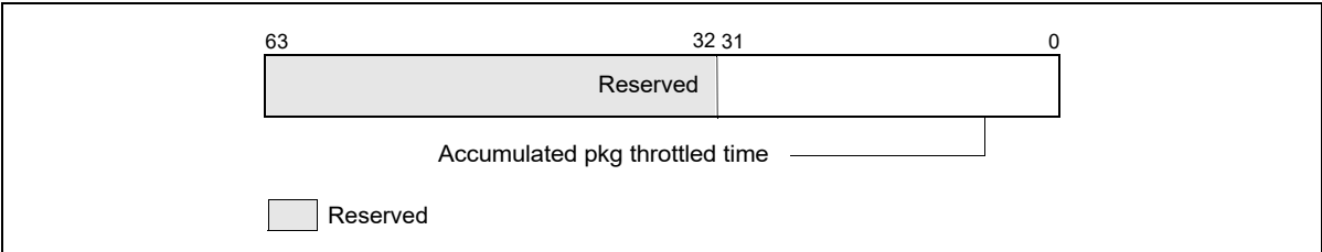
Figure 16-39. MSR_PKG_PERF_STATUS MSR
