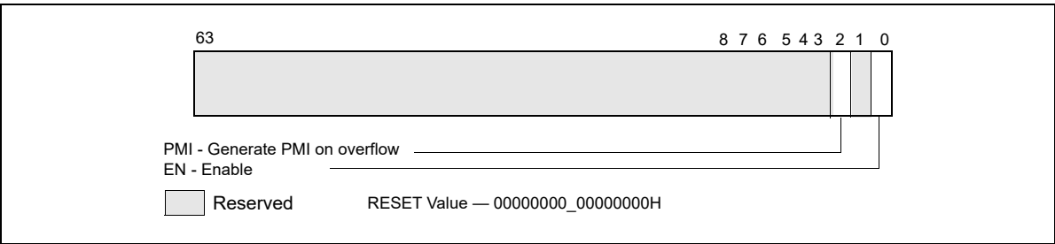
Figure 21-25. Layout of MSR_UNCORE_FIXED_CTR_CTRL MSR
