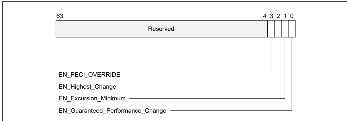
Figure 16-12. IA32_HWP_INTERRUPT MSR
