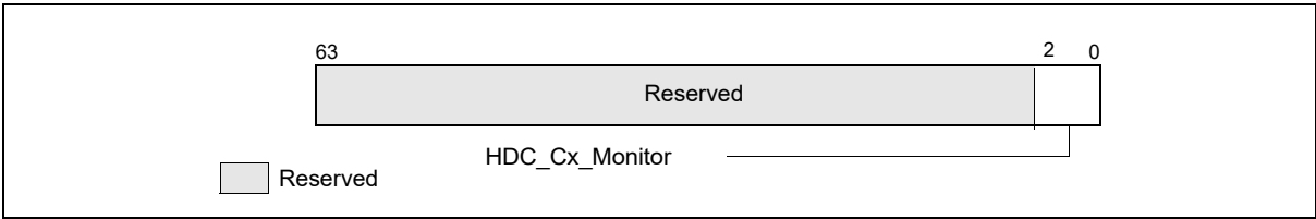
Figure 17-22. MSR_PKG_HDC_CONFIG MSR
