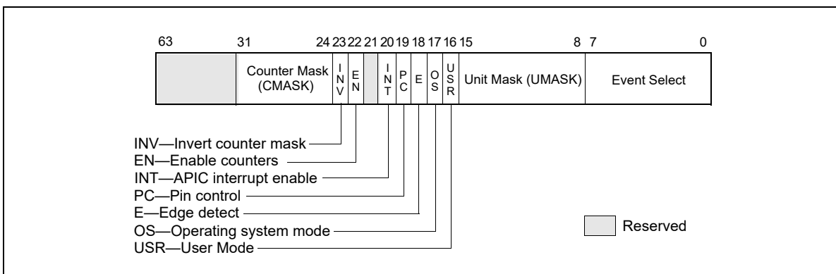
Figure 22-1. Layout of IA32_PERFEVTSELx MSRs
