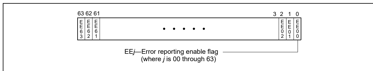
Figure 18-5. IA32_MCI_CTL Register
