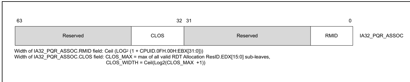
Figure 20-23. IA32_PQR_ASSOC MSR
