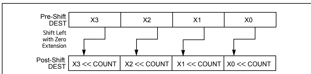
Figure 4-12. PSLW, PSLD, and PSLQ Instruction Operation Using 64-bit Operand
