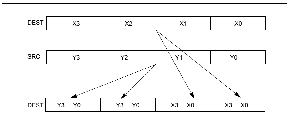
Figure 4-19. SHUFPS Shuffle Operation
