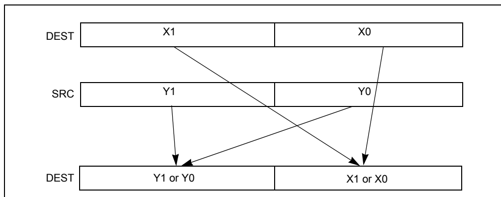
Figure 4-21. SHUFDP Shuffle Operation
