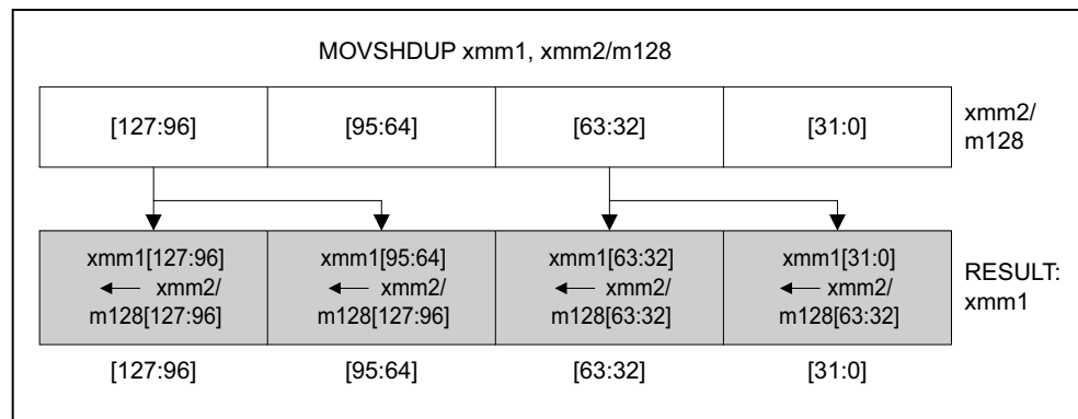
Figure 3-25. MOVSHDUP—Move Packed Single-FP High and Duplicate
