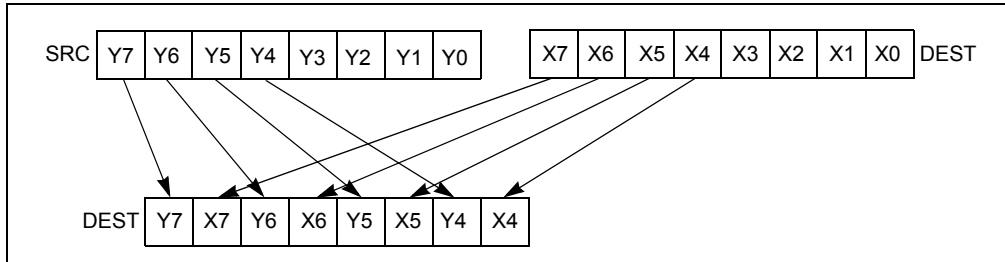
Figure 4-20. PUNPCKHBW Instruction Operation Using 64-bit Operands
